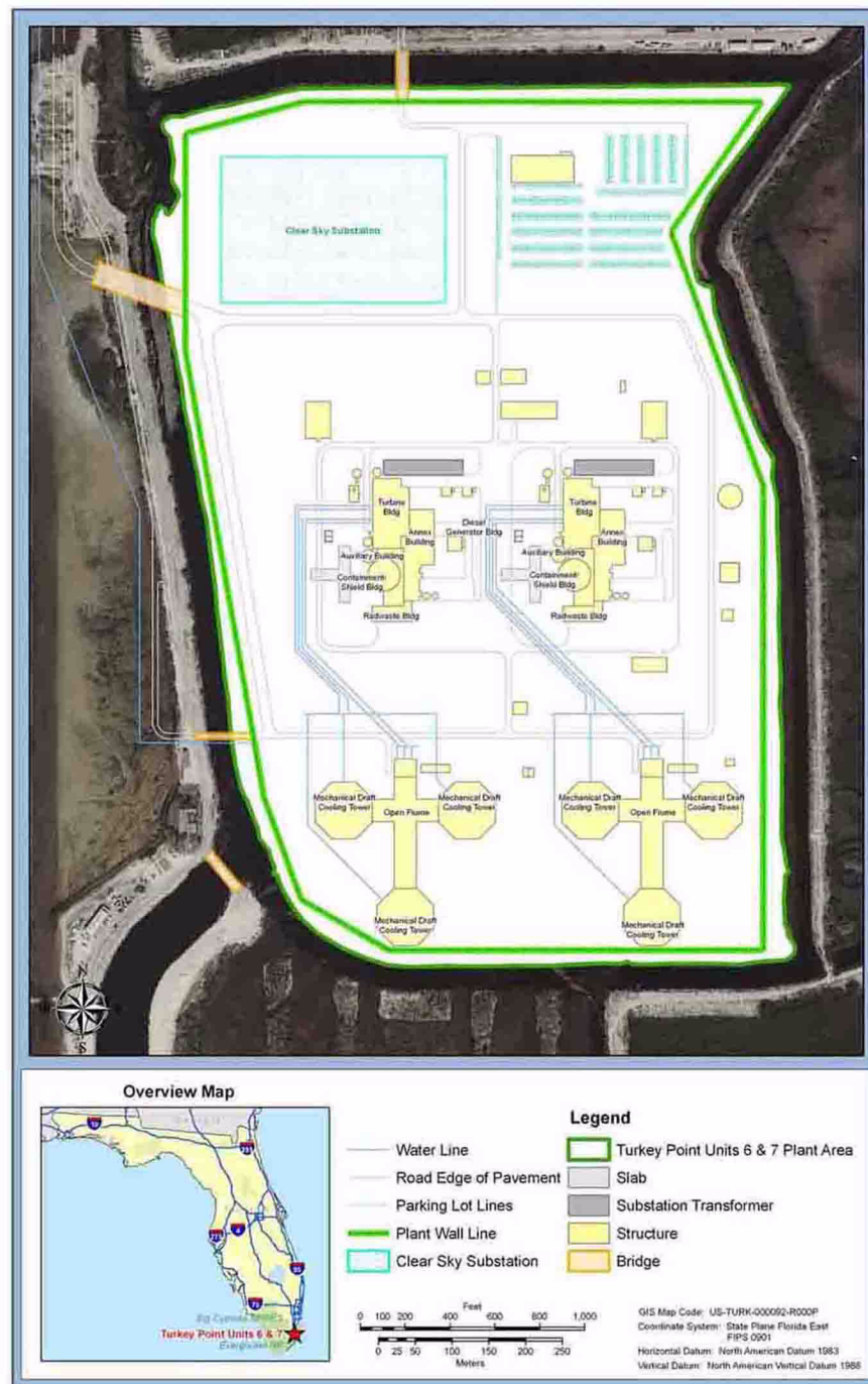
Figure 2.1-205 Principal Plant Structures within the Site Area
