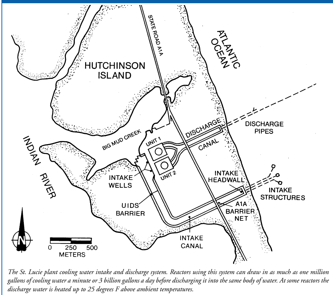
Figure 2: St. Lucie Plant cooling water intake and discharge system
