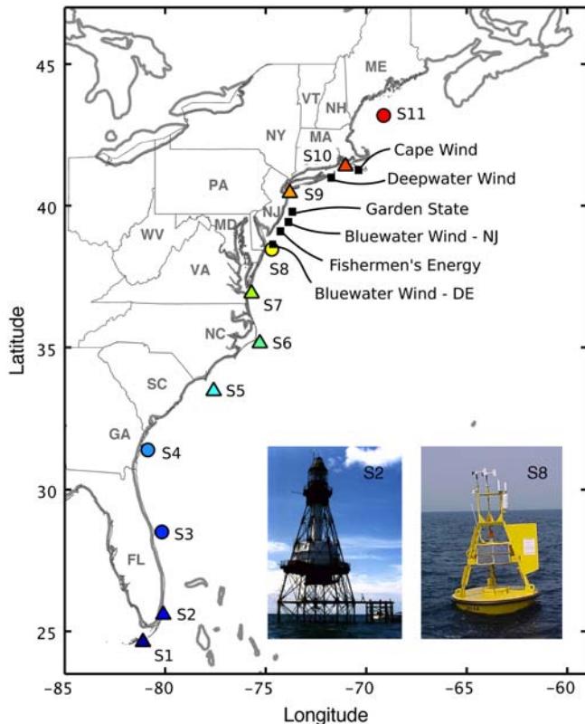
Fig. 1. Proposed offshore wind projects off the U.S. coast (black squares and names). NDBC offshore meteorological stations selected for this study, running from Florida (S1) to Maine (S11) with color bullets for buoys and color triangles for towers. Inset photos: disc buoy (S8), with anemometer height of z_{ref} = 5 m, and a lighthouse tower (S2) at z_{ref} = 44 m.
