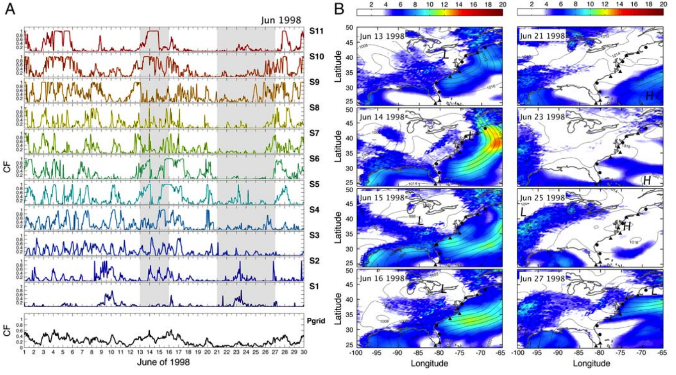
Fig. 7. (A) Capacity factors in June 1998 for 11 stations and for the Grid (Lowermost). The two gray date ranges are expanded to the right. (B) Sea level pressure (lines, in hPa) and wind speed (color scale, m s^{-1} ) for the event of June 13–16 (Left) and June 21–27 (Right).
