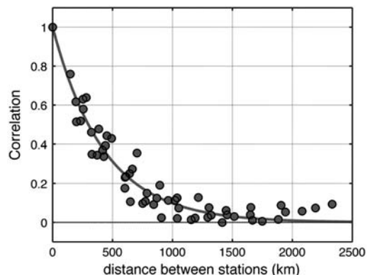
Fig. 2. Correlation R between pairs of stations, by distance. The gray curve represents an exponential fit R = \exp(-x/D) for the optimum value of D = 430 km.
