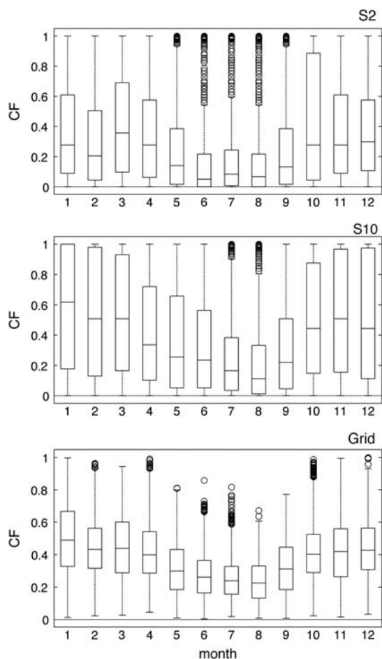
Fig. 4. Capacity factor monthly variability for individual wind parks at S2, S10, and for P_{grid} , shown as boxplots. The central mark in each box is the median; box edges are the 25th and 75th percentiles. The whiskers extend to the most extreme data-points not considered outliers (approximately \pm 2.7\sigma and 99.3% coverage if data is normally distributed). Outliers are plotted as circles.
