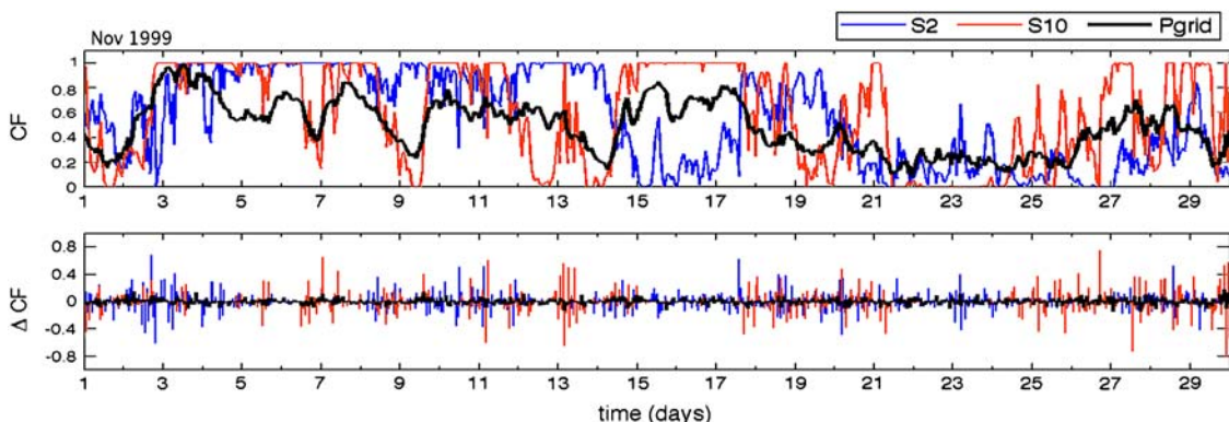
Fig. 3. (Top) One month of power, expressed as CF, from two isolated wind parks (blue and orange lines) compared with power from the Atlantic Transmission Grid ( P_{grid} , thick black line). (Bottom) Hourly changes in CF, comparing individual wind parks (blue and orange) with the Grid (black line).
