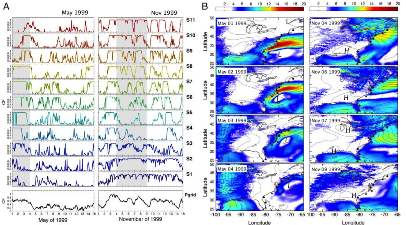
Fig. 6. (A) Capacity factors for 11 stations in May 1999 and November 1999; line colors match station colors in Fig. 1. The lowest graph, P_{grid} , is the aggregate CF if all stations are connected by transmission. The two gray date ranges are each expanded to 4 d on the maps (B). (B) Sea level pressure (lines, in hPa) and wind speed (color scale at top, in m s^{-1} ) for the events from May 1–4 (Left) and November 4–9 (Right), 1999.
