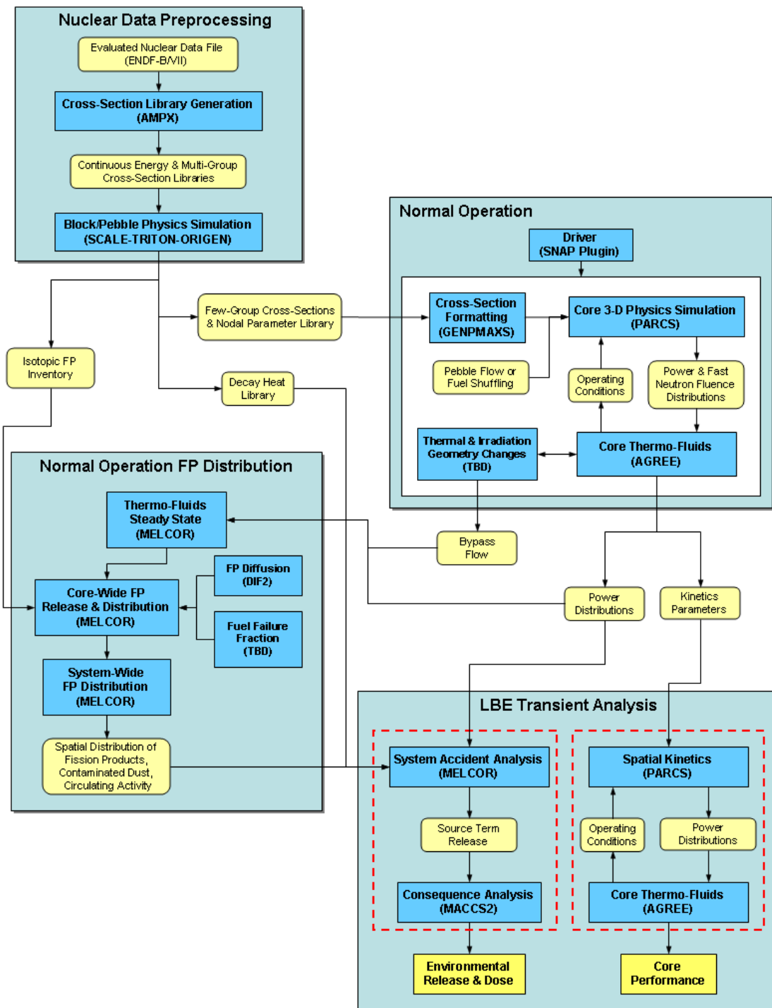
Figure 1. Schematic of the NRC Accident Analysis Evaluation Model Concept for HTGRs.
