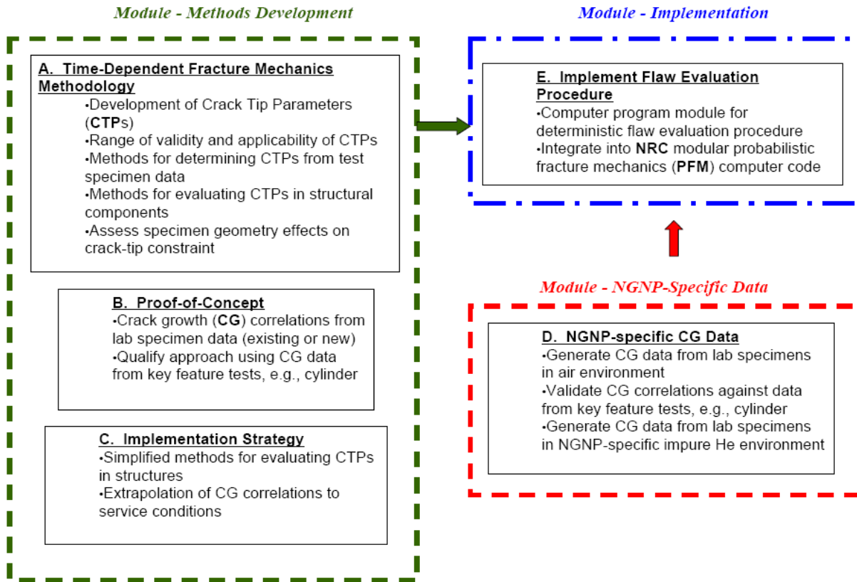
Figure 2. Metallic Material Evaluation Model and Modules.
