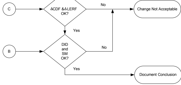
Figure 4-940 Plant Change Evaluation [NEI 04-02 Figure 5-1] Note references in Figure refer to NEI 04-02 Sections
