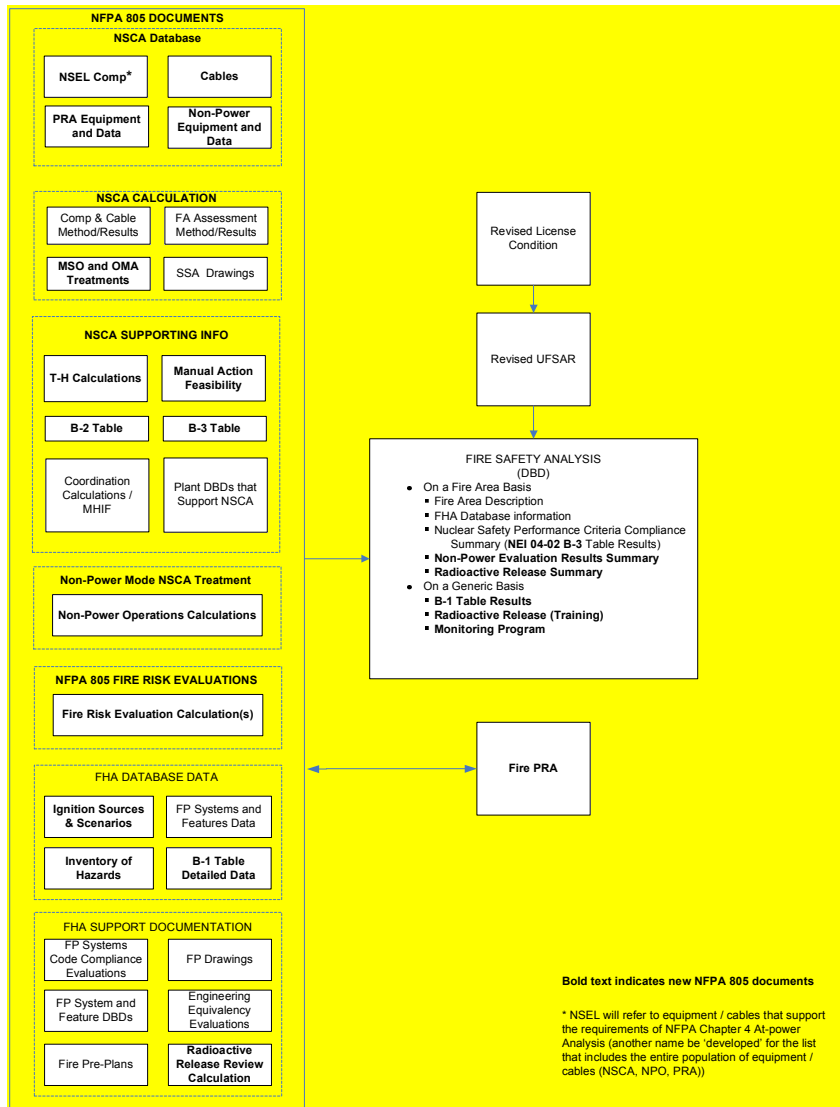
Figure 4-89 – NFPA 805 Planned Post-Transition Documents and Relationships
