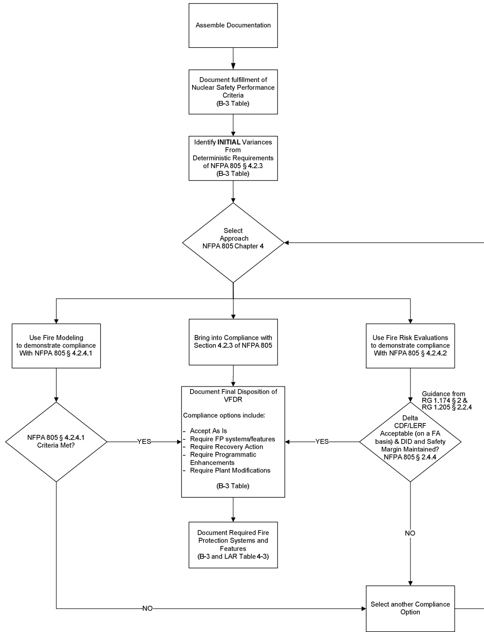
Figure 4-45 – Summary of Fire Area-by-Fire Area Review [Based on Draft FAQ 07-0055 Revision 0]
