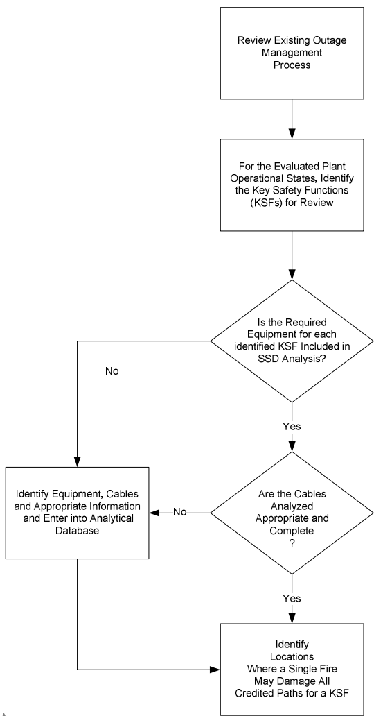
Figure 4-56 Review POSs, KSFs, Equipment, and Cables, and Identify Pinch Points
