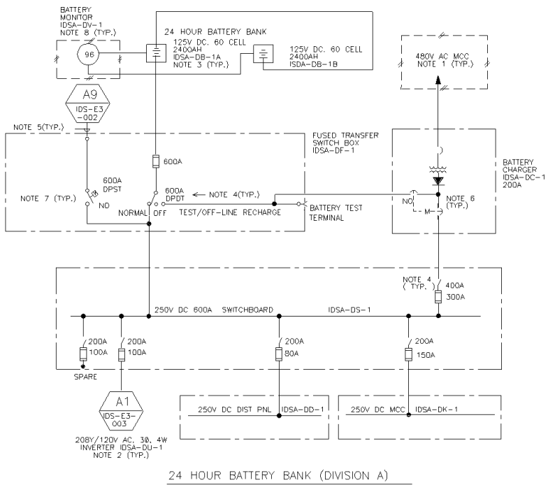
24 HOUR BATTERY BANK (DIVISION A)
