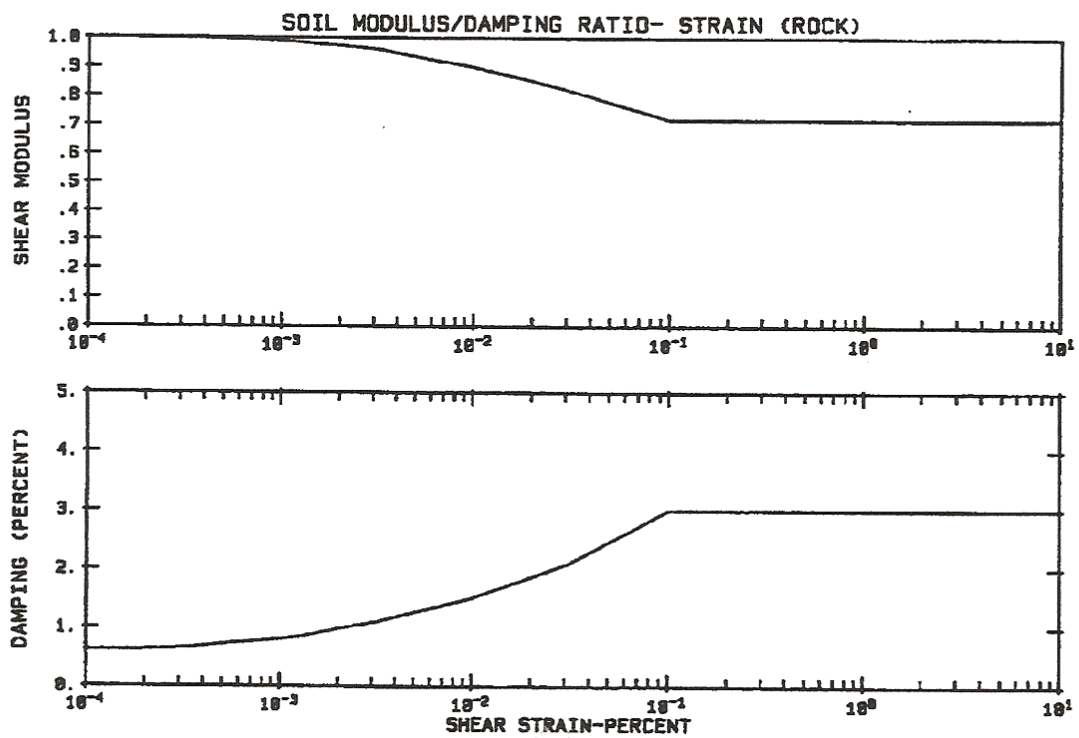
Modulus Reduction Curves for Generic Soil Sites
