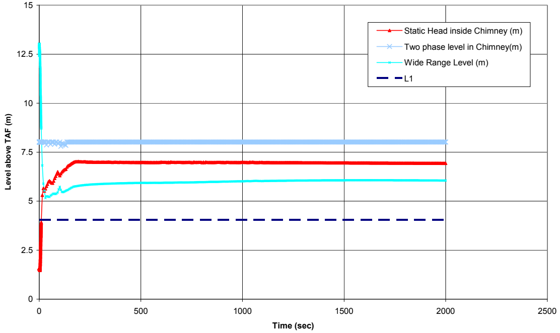
Figure 15.5-10c. Station Blackout
