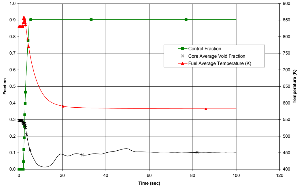
Figure 15.5-11f. MSIV Closure With Flux Scram
