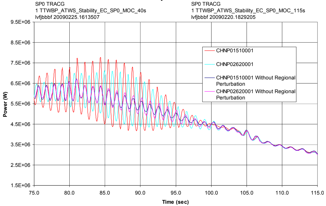
Figure 15.5-9. Core Stability During Turbine Trip with Full Bypass ATWS Event
