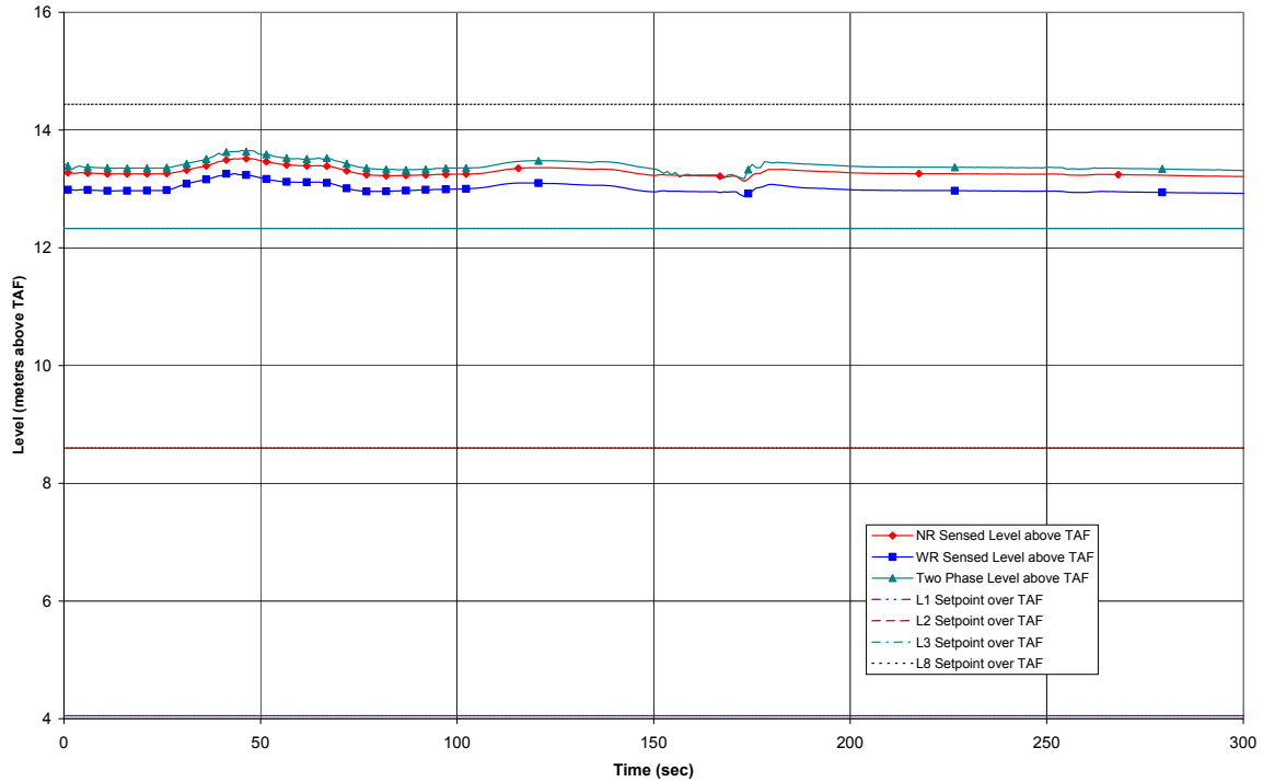
Figure 15.2-11c. Inadvertent Isolation Condenser Initiation
