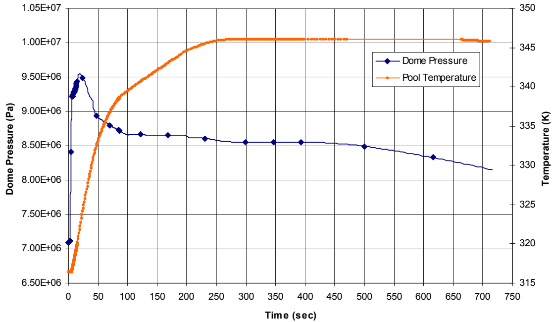
Figure 15.5-3b. ATWS MSIV Closure - SLC System Bounding Case
