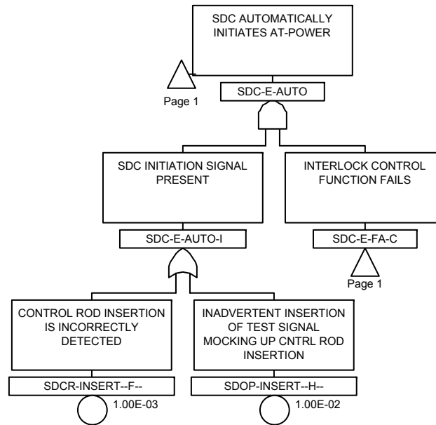
Figure 15A-3c. Fault Tree – Inadvertent Shutdown Cooling Function Operation (page 3 of 3)
