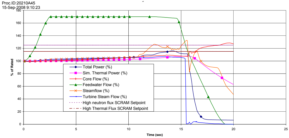
Figure 15.3-2a. Feedwater Controller Failure – Maximum Flow Demand
