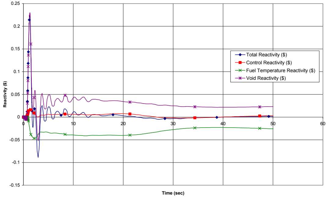
Figure 15.2-2e. Fast Closure of One Turbine Control Valve
