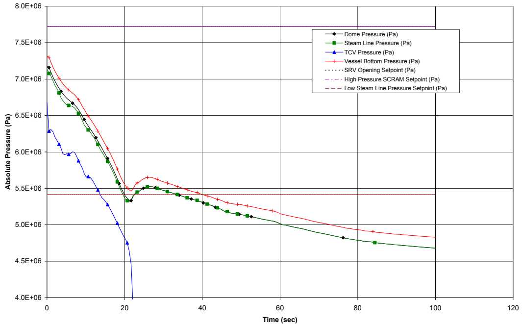
Figure 15.3-3d. Pressure Regulator Failure – Opening of All Turbine Control and Bypass Valves
