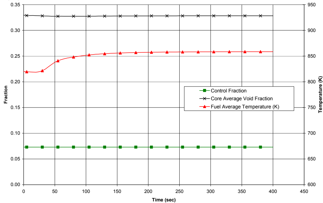
Figure 15.3-1f. Loss of Feedwater Heating with SCRRI/SRI Failure
