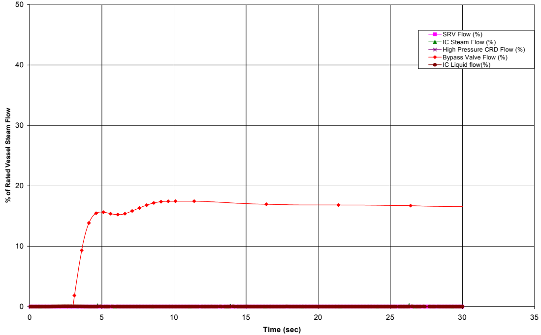
Figure 15.2-3b. Slow Closure of One Turbine Control Valve
