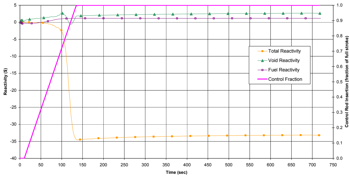
Figure 15.5-2c. ATWS MSIV Closure with FMCRD Run-in
