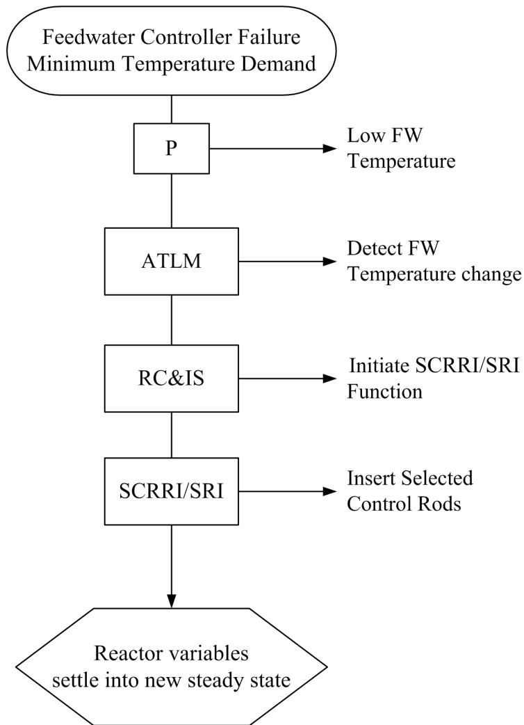
Figure 15.1-17b. Event Diagram – Feedwater Controller Failure - Minimum Temperature Demand
