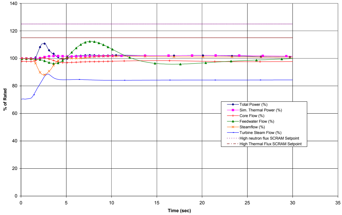
Figure 15.2-3a. Slow Closure of One Turbine Control Valve
