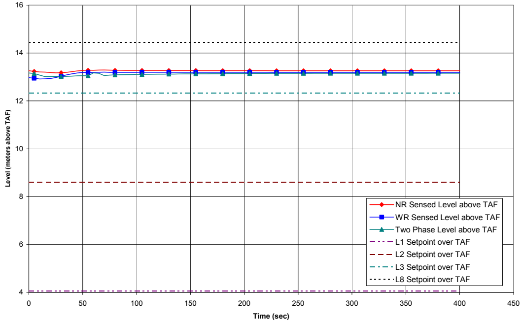
Figure 15.3-1c. Loss of Feedwater Heating with SCRRI/SRI Failure
