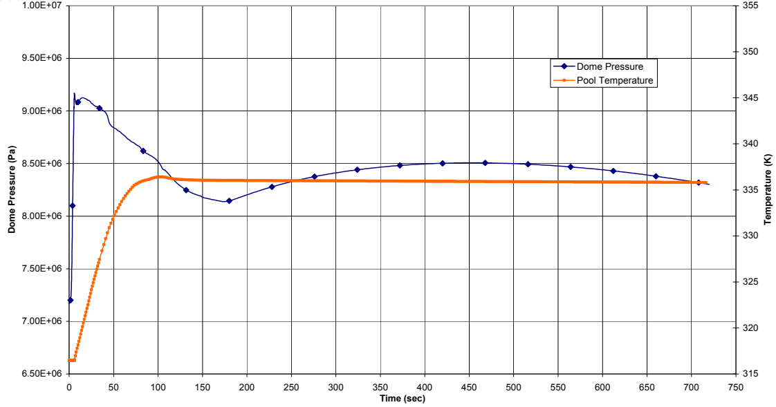
Figure 15.5-2b. ATWS MSIV Closure with FMCRD Run-in
