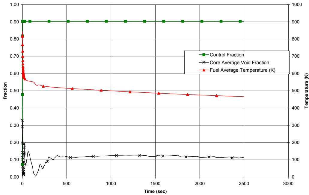
Figure 15.3-9f. Stuck Open Safety Relief Valve
