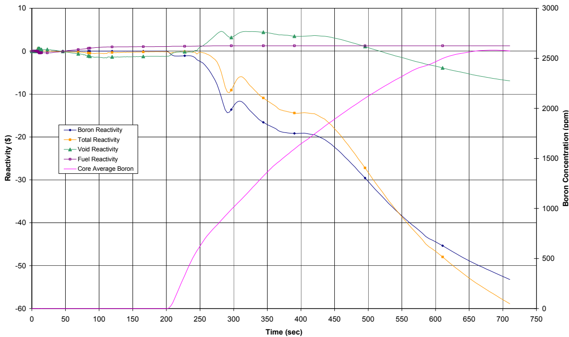
Figure 15.5-4c. ATWS Loss of Condenser Vacuum SLC System Bounding Case
