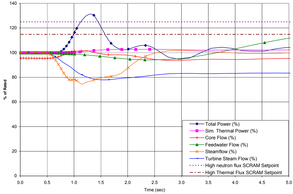
Figure 15.2-2h. Fast Closure of One Turbine Control Valve (Figure 15.2-2a from 0 to 5s)
