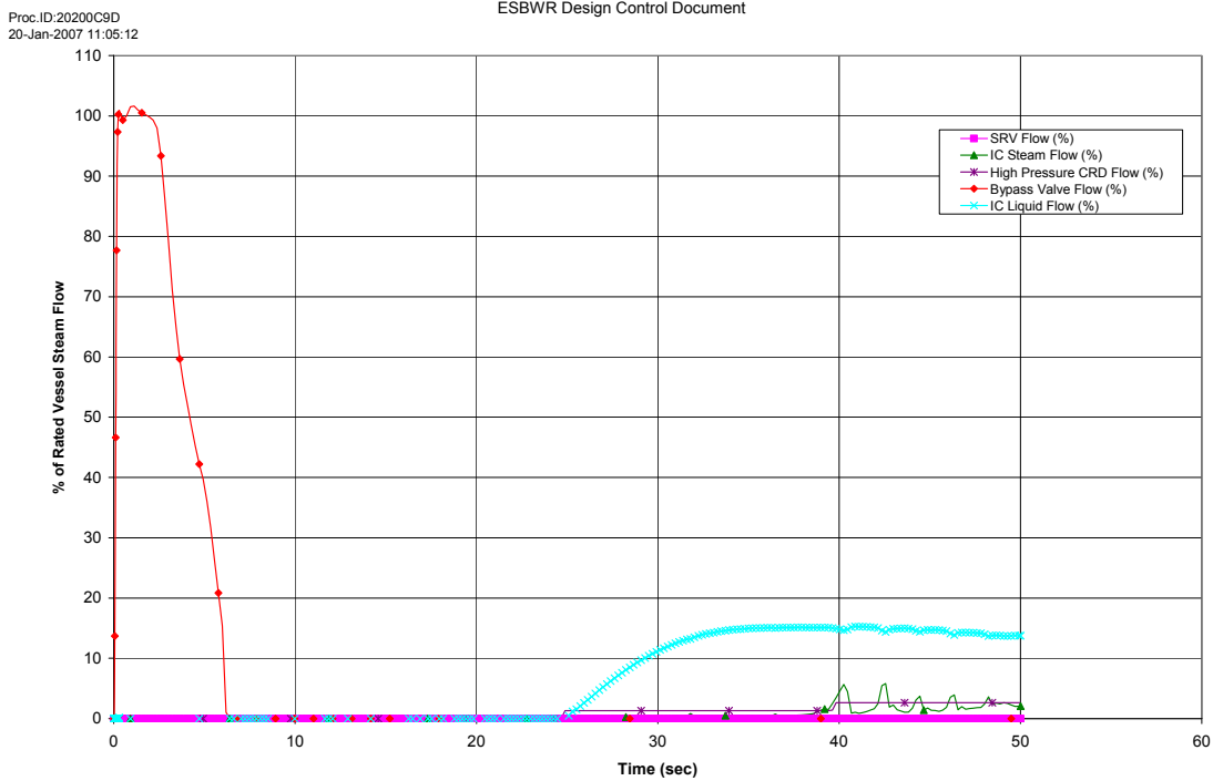
Figure 15.2-10a. Loss of Condenser Vacuum
