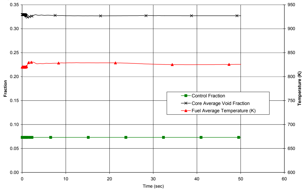
Figure 15.2-2f. Fast Closure of One Turbine Control Valve
