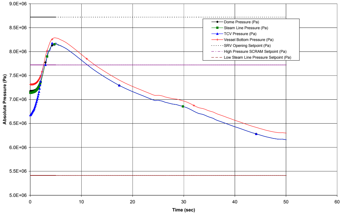
Figure 15.3-4d. Pressure Regulator Failure – Closure of All Turbine Control and Bypass Valves
