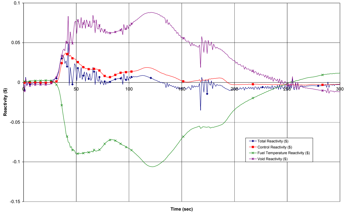
Figure 15.2-11e. Inadvertent Isolation Condenser Initiation
