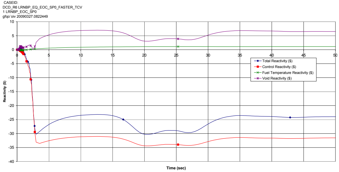
Figure 15.3-5e. Generator Load Rejection With Total Turbine Bypass Failure
