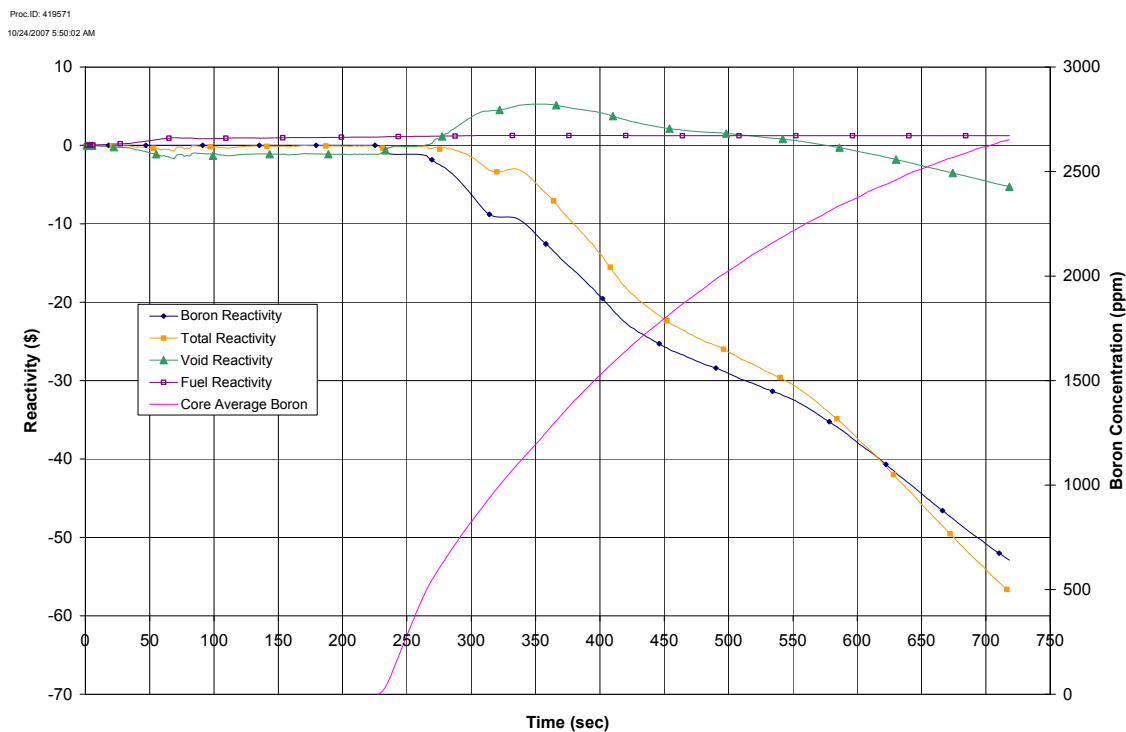
Figure 15.5-7c. ATWS Loss of Feedwater Flow with Boron Injection
