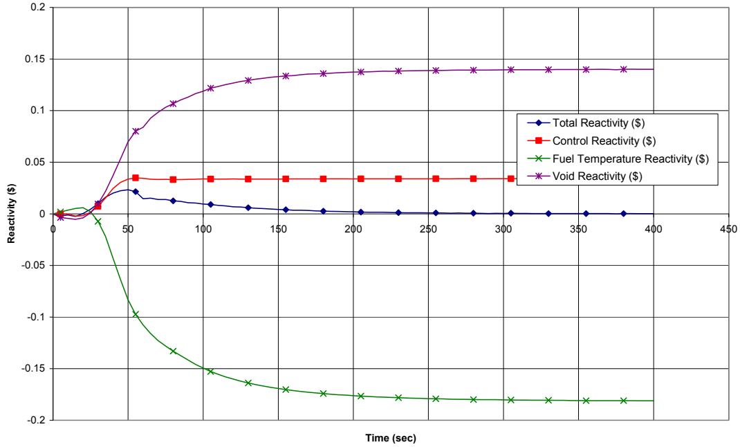
Figure 15.3-1e. Loss of Feedwater Heating with SCRRI/SRI Failure
