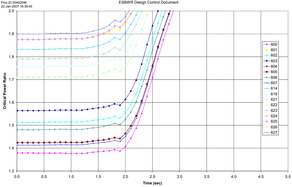
Figure 15.2-9g. Closure of All MSIVs
