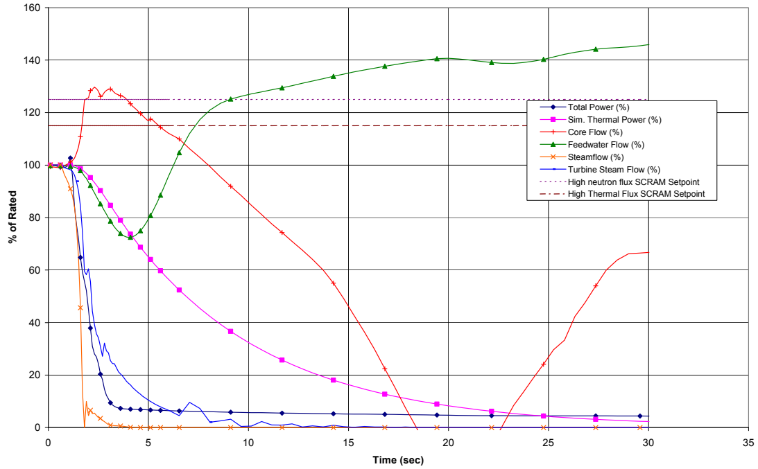
Figure 15.2-9a. Closure of All MSIVs
