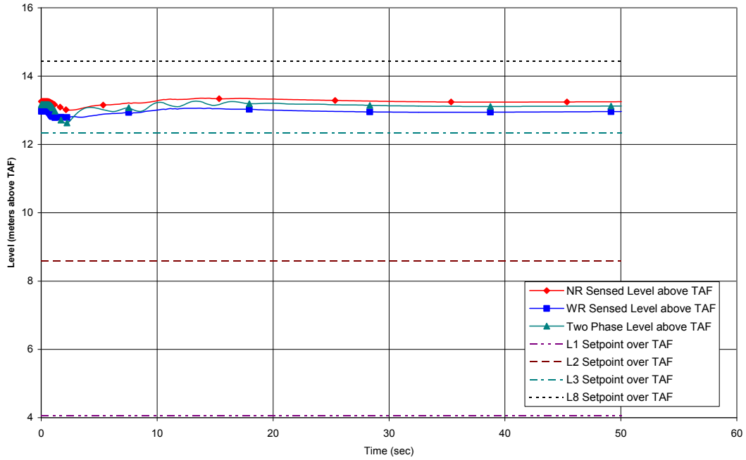
Figure 15.2-2c. Fast Closure of One Turbine Control Valve
