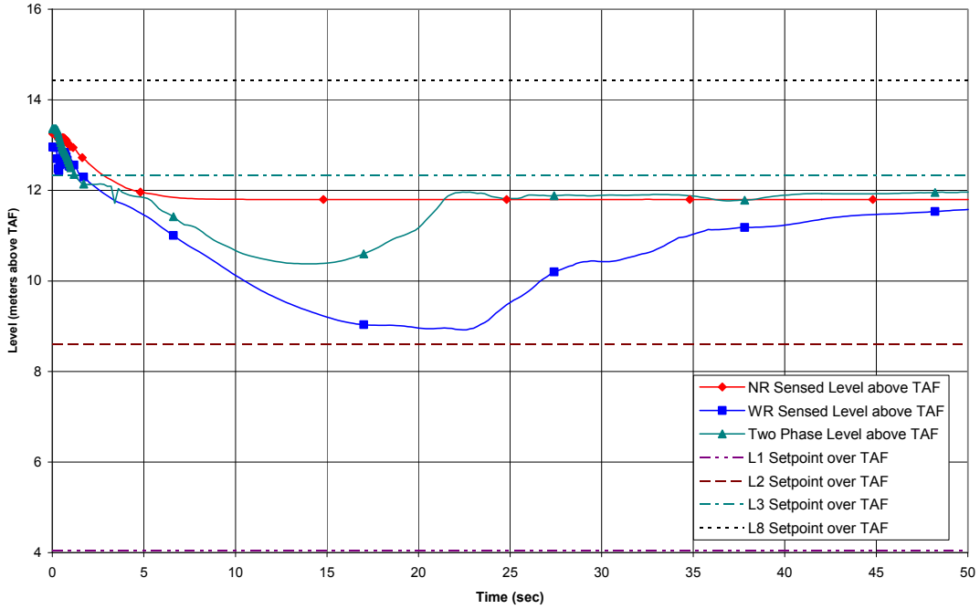
Figure 15.2-7c. Turbine Trip with a Single Failure in the Turbine Bypass System
