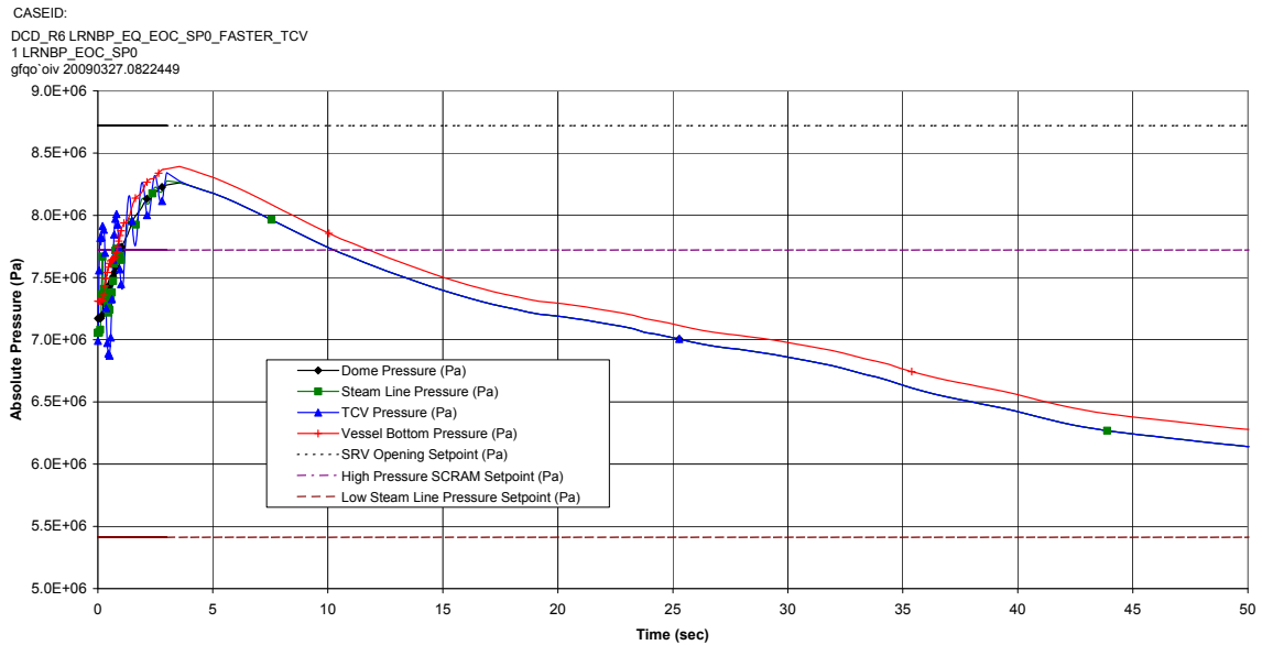
Figure 15.3-5d. Generator Load Rejection With Total Turbine Bypass Failure
