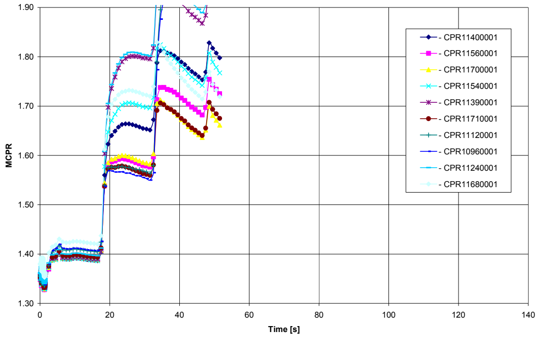
Figure 15.2-6g. Turbine Trip with Turbine Bypass
