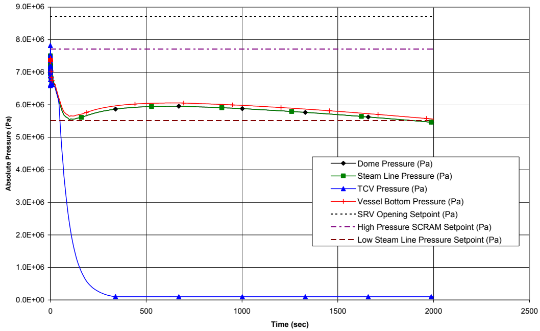
Figure 15.5-10d. Station Blackout
