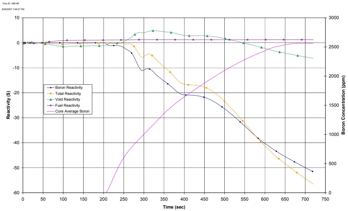
Figure 15.5-6c. ATWS Loss of Normal AC Power to Station Auxiliaries with Boron Injection
