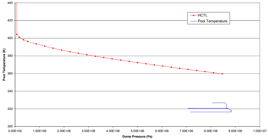
Figure 15.5-8d. ATWS Load Rejection with a Single Failure in the Turbine Bypass System with Boron Injection
