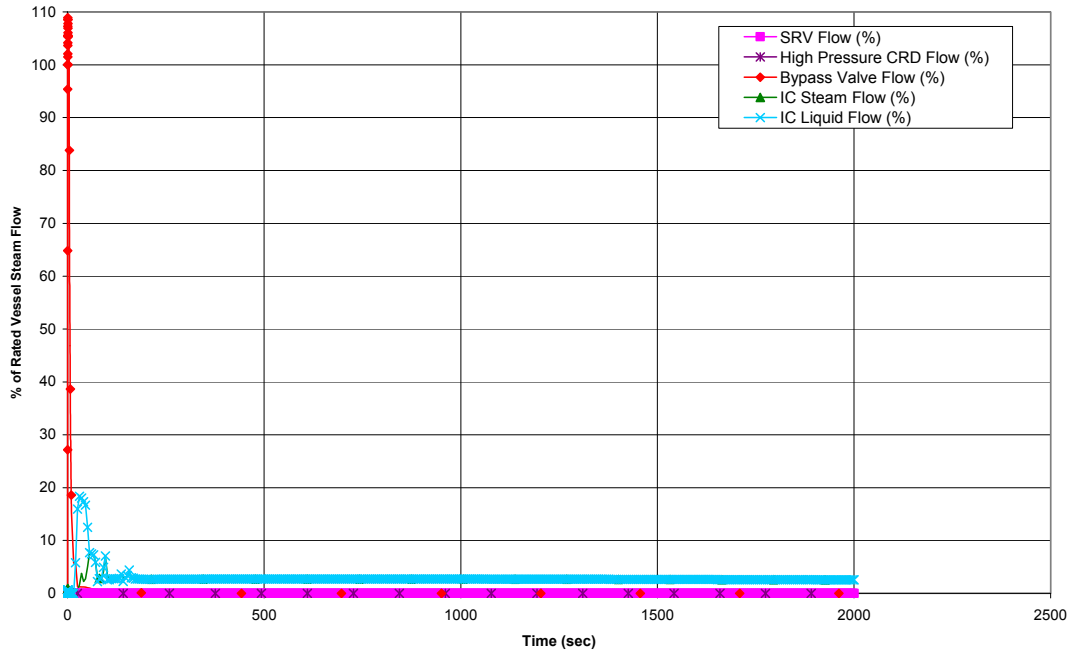
Figure 15.5-10b. Station Blackout
