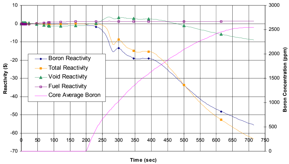
Figure 15.5-3c. ATWS MSIV Closure - SLC System Bounding Case
