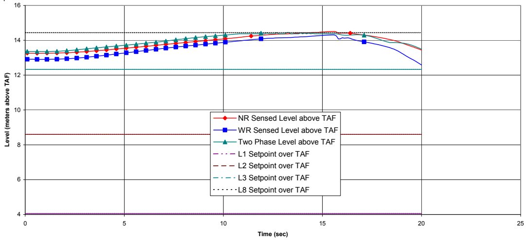
Figure 15.3-2c. Feedwater Controller Failure – Maximum Flow Demand
