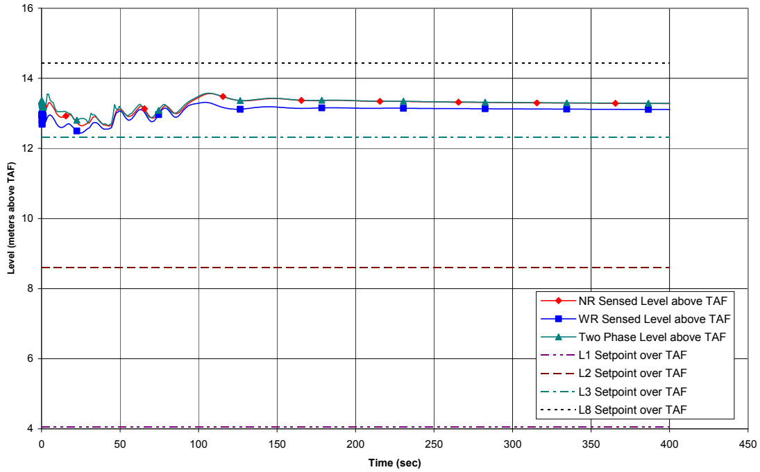
Figure 15.2-6c. Turbine Trip with Turbine Bypass
