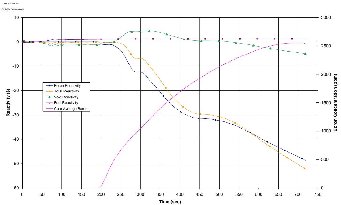
Figure 15.5-8c. ATWS Load Rejection with a Single Failure in the Turbine Bypass System with Boron Injection
