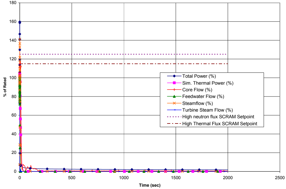
Figure 15.5-10a. Station Blackout
