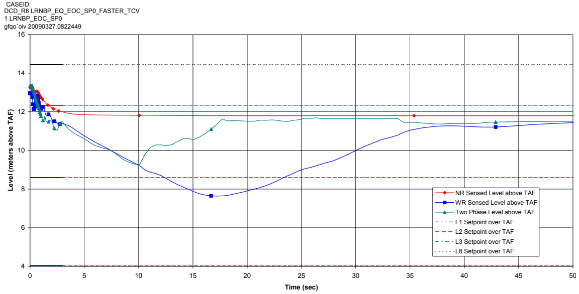
Figure 15.3-5c. Generator Load Rejection With Total Turbine Bypass Failure
