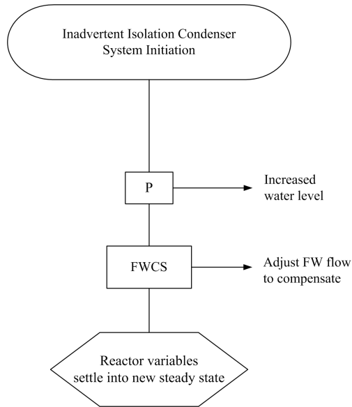
Figure 15.1-12. Event Diagram – Inadvertent Isolation Condenser Initiation
