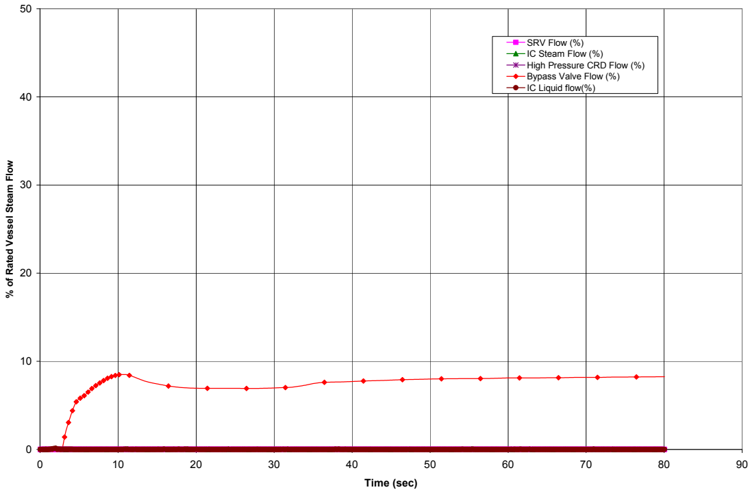
Figure 15.2-8b. Closure of One MSIV
