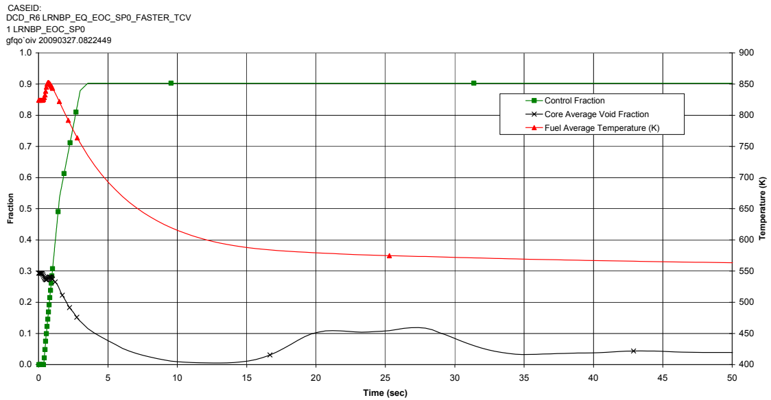
Figure 15.3-5f. Generator Load Rejection With Total Turbine Bypass Failure
