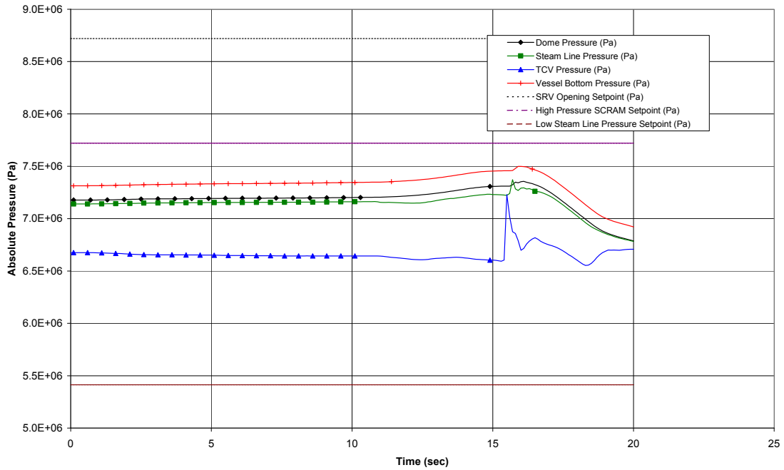
Figure 15.3-2d. Feedwater Controller Failure – Maximum Flow Demand
