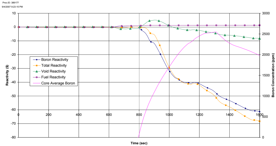
Figure 15.5-5c. ATWS Loss of Feedwater Heating with Boron Injection
