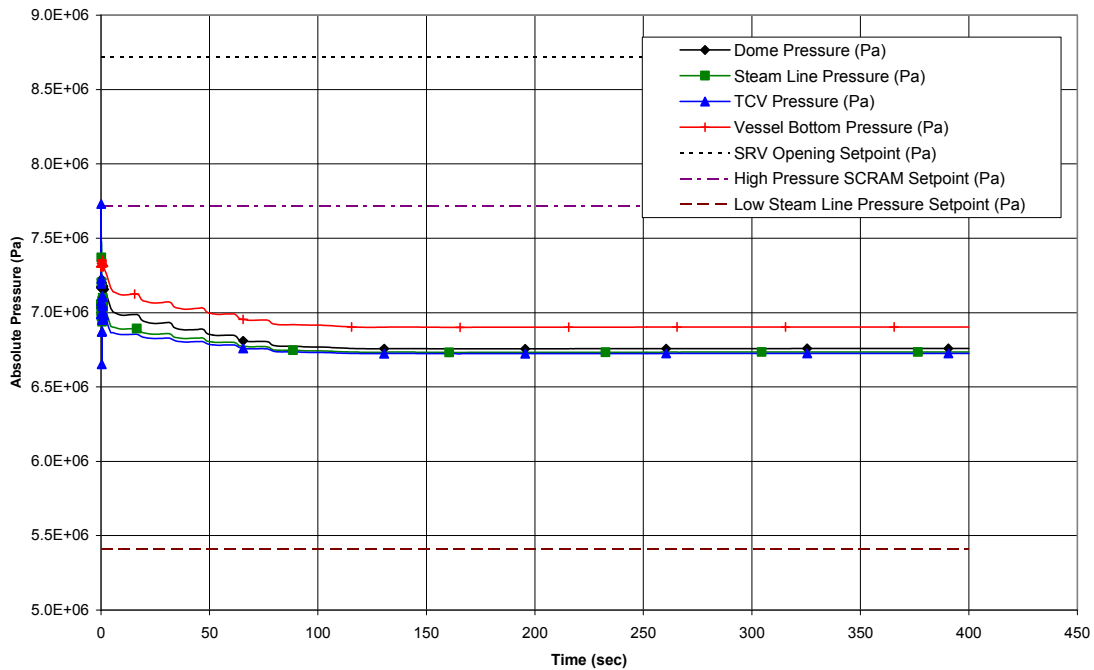
Figure 15.2-6d. Turbine Trip with Turbine Bypass
