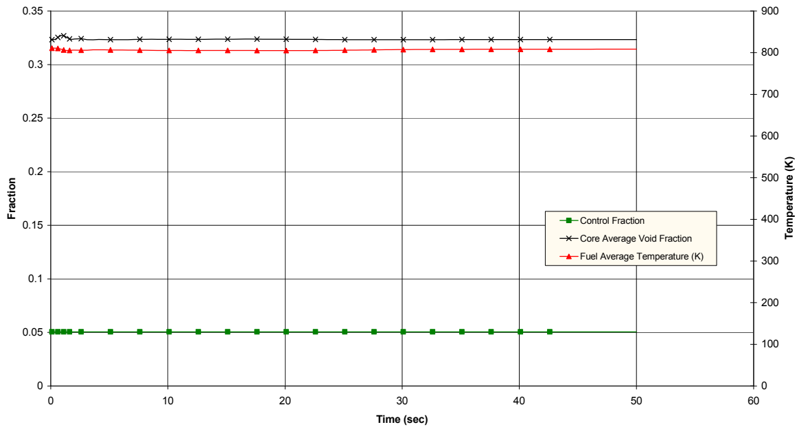
Figure 15.2-14f. Opening of One Turbine Control or Bypass Valve
