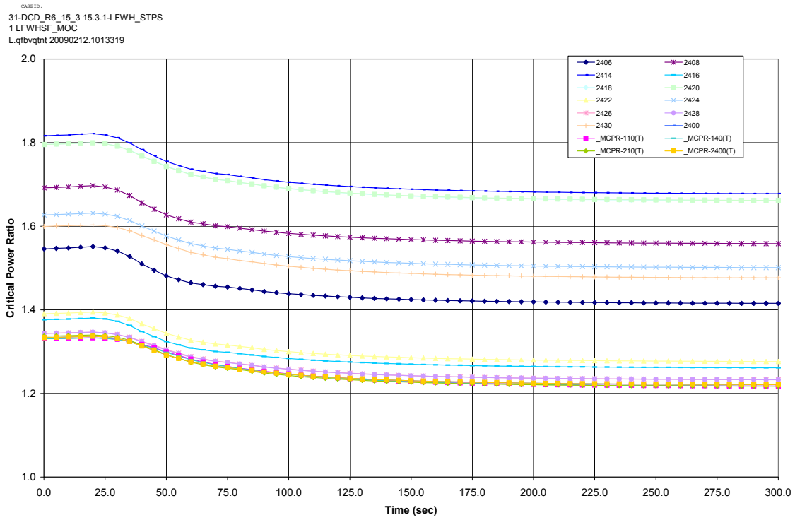
Figure 15.3-1g. Loss of Feedwater Heating with SCRRI/SRI Failure
