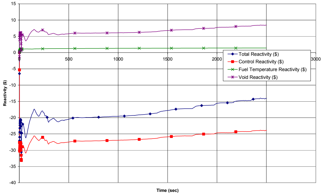
Figure 15.3-9e. Stuck Open Safety Relief Valve
