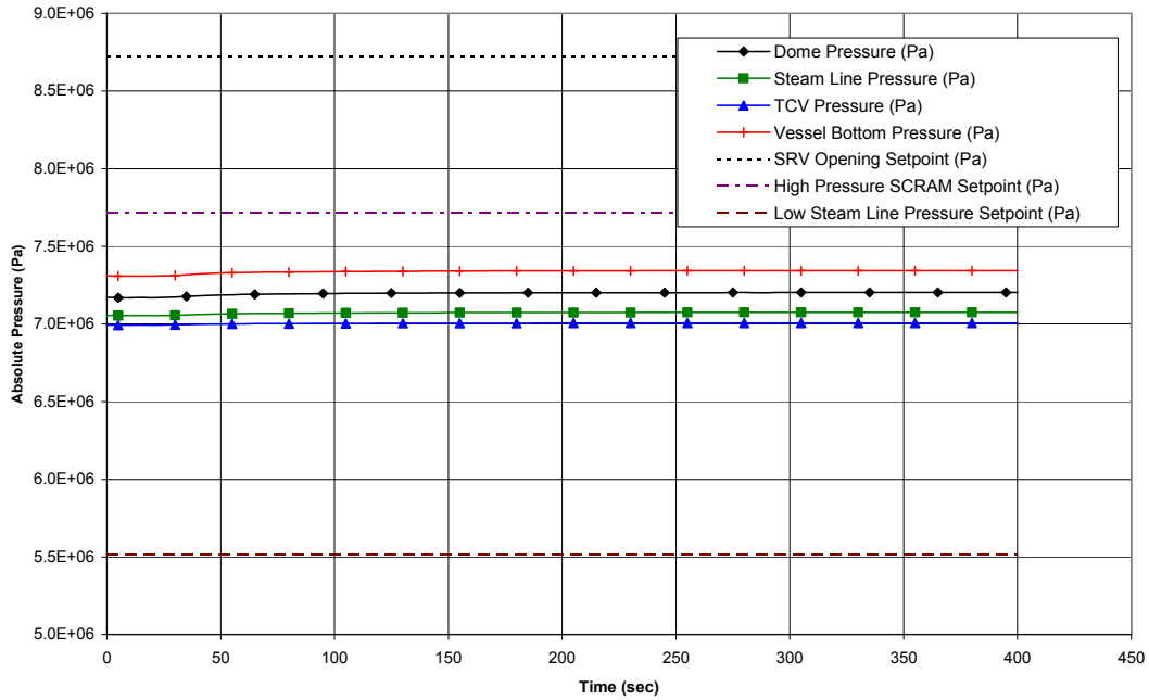
Figure 15.3-1d. Loss of Feedwater Heating with SCRRI/SRI Failure
