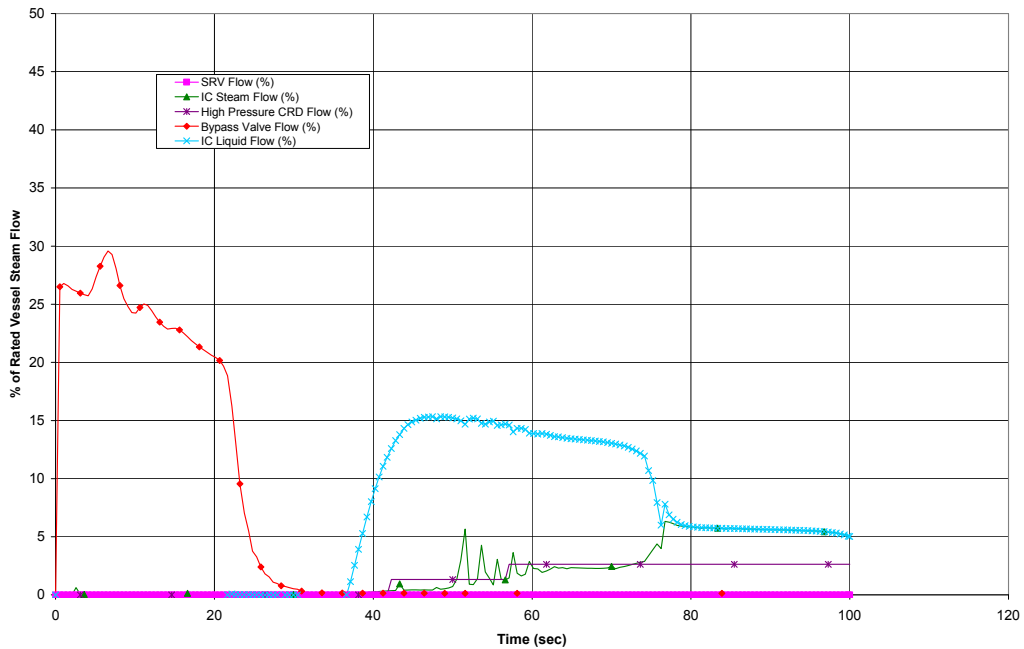
Figure 15.3-3b. Pressure Regulator Failure – Opening of All Turbine Control and Bypass Valves
