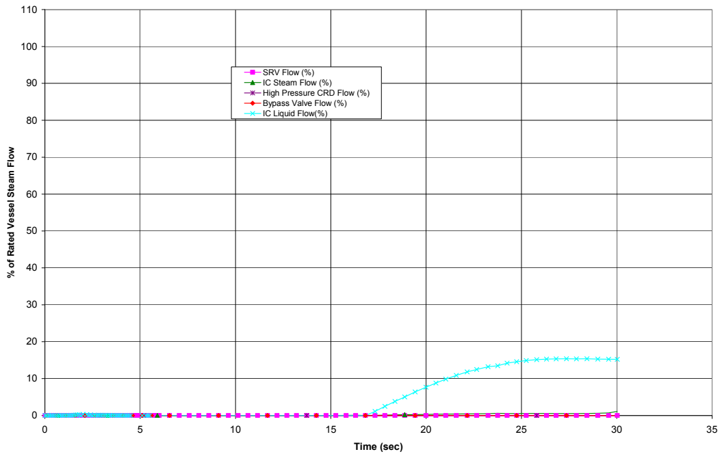
Figure 15.2-9b. Closure of All MSIVs
