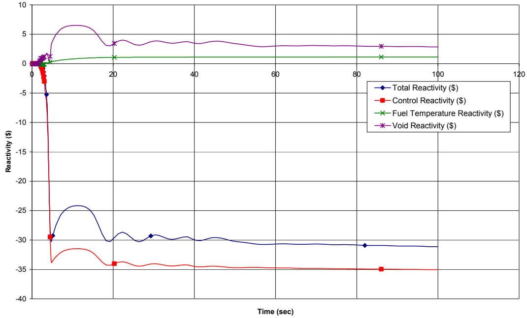
Figure 15.5-11e. MSIV Closure With Flux Scram
