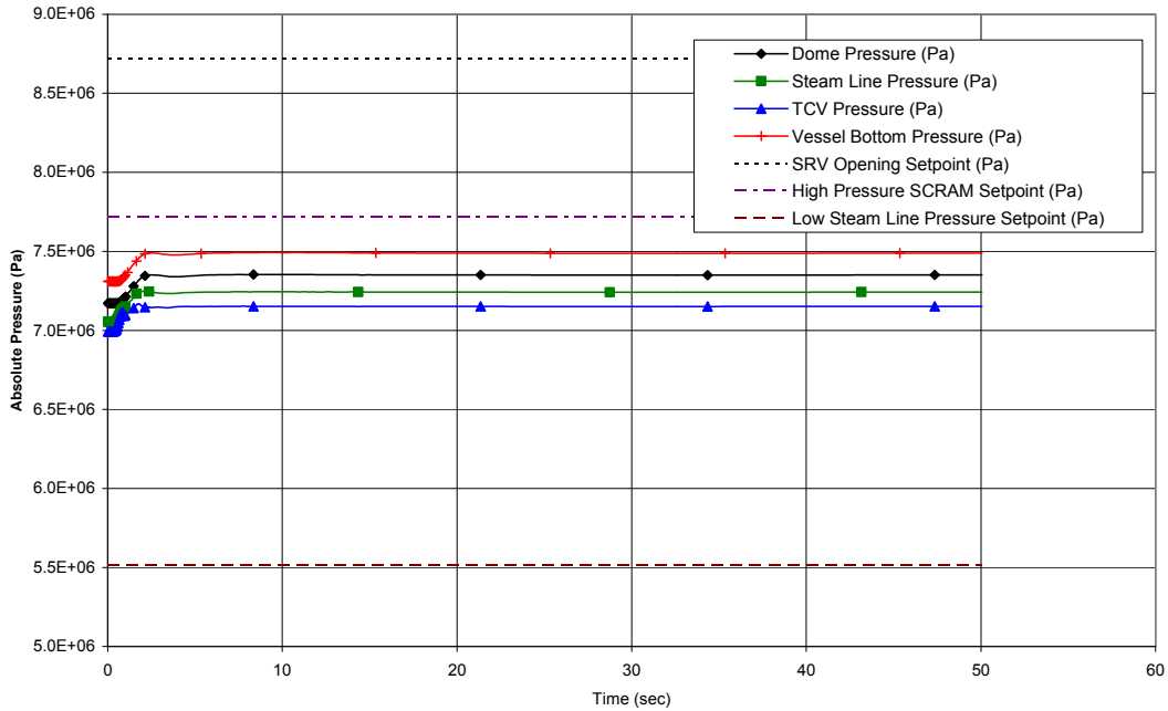
Figure 15.2-2d. Fast Closure of One Turbine Control Valve
