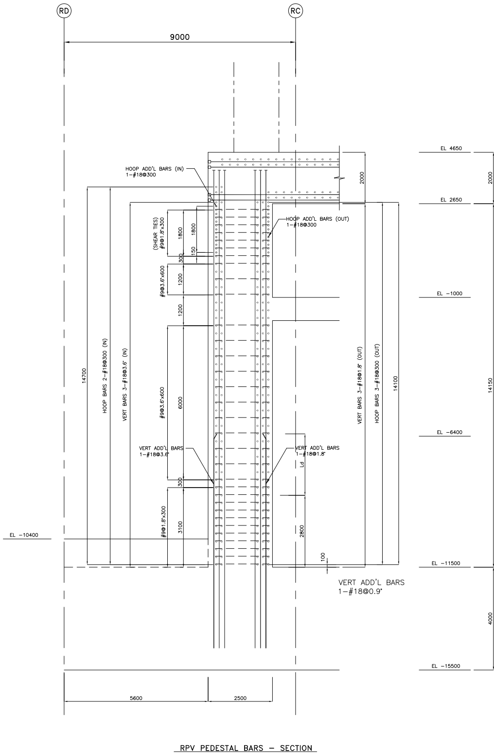
Figure 3G.1-45. Reinforcing Steel of RPV Pedestal
