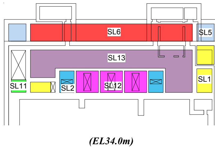
Figure 3G.5-14. RB Upper Pools - Slab Sections for Heat Transfer Calculation
