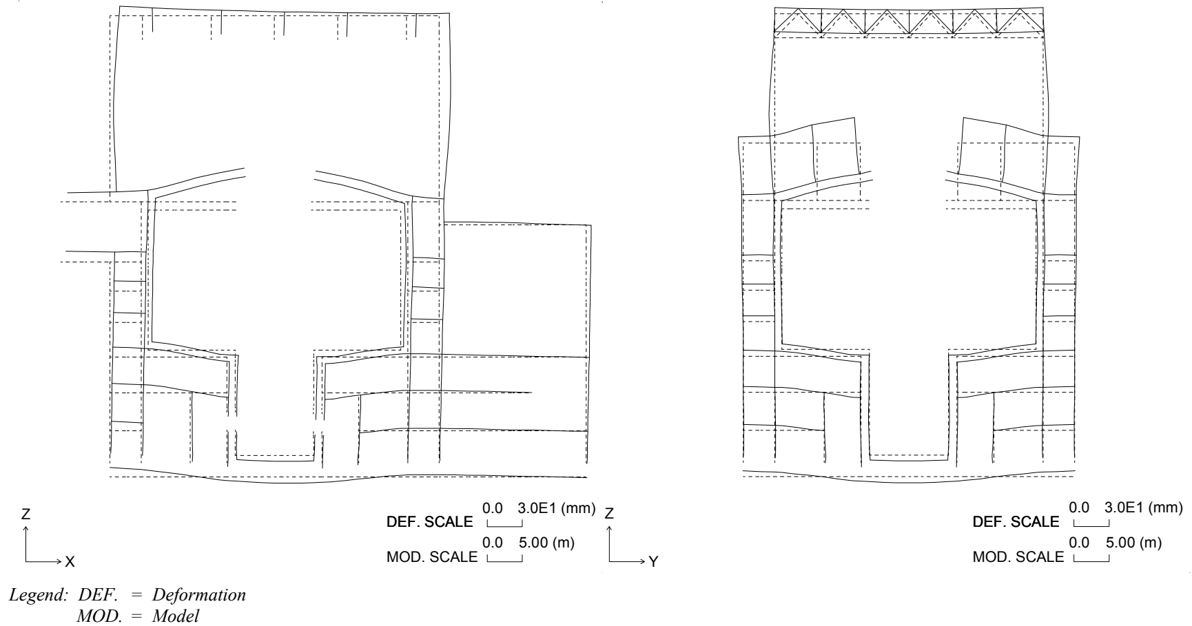
Figure 3G.1-31. Section Deformation for Drywell Unit Pressure (1 MPa)
