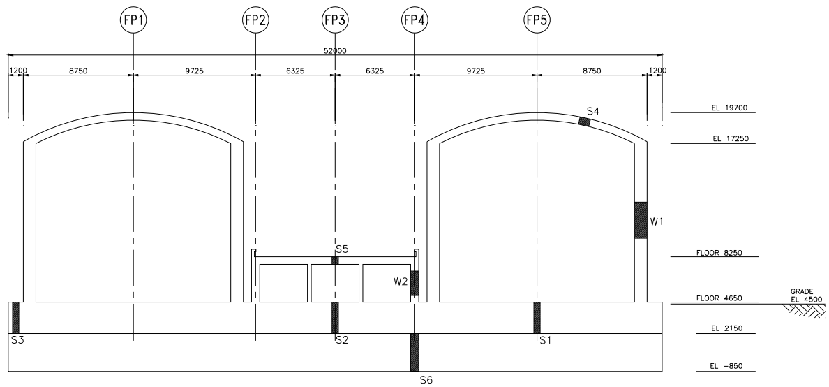
Figure 3G.4-7. Sections Where Thermal Loads Are Defined
