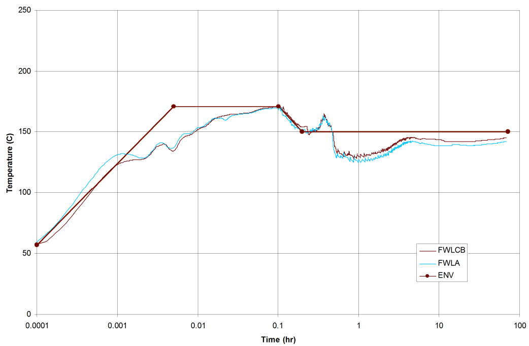
Figure 3G.5-2. DW Design Temperature Curve (ENV) vs. TRACG Medium-Term Bounding Temperature Curve
