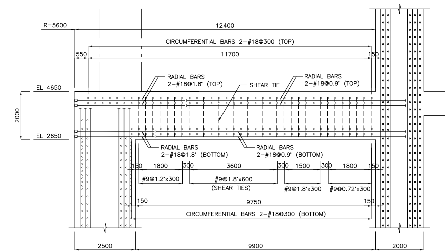
SUPPRESSION POOL SLAB – SECTION
