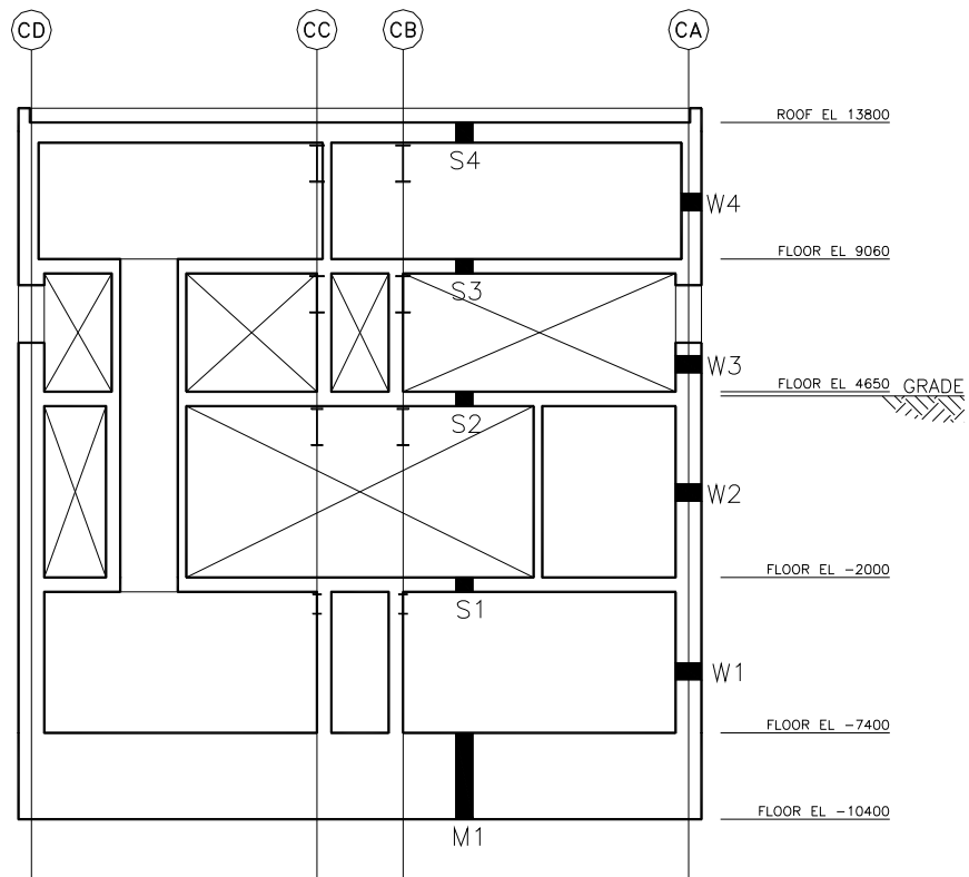
Figure 3G.2-13. Sections Where Thermal Loads Are Defined
