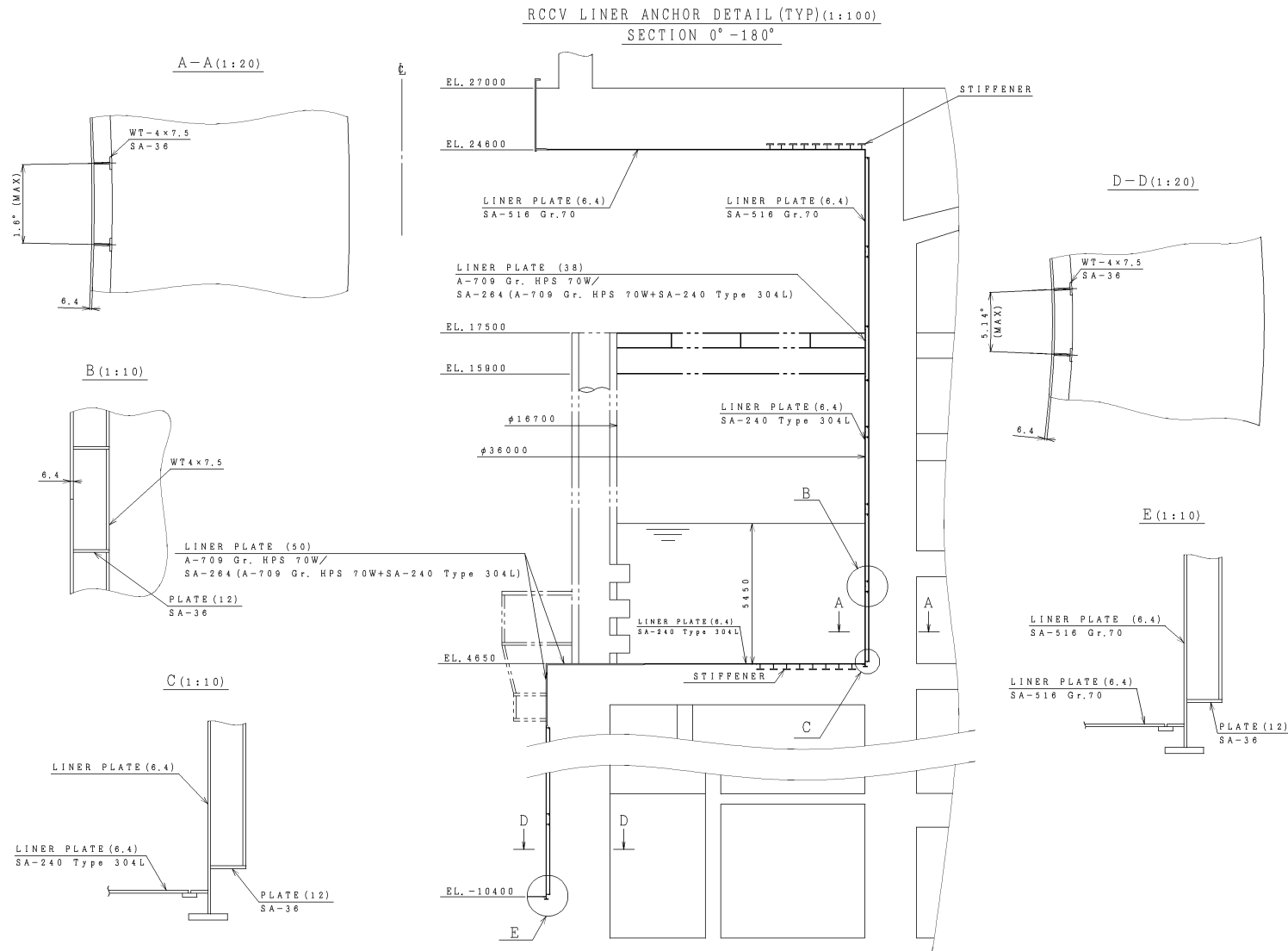
Figure 3G.1-48. Liner Anchor
