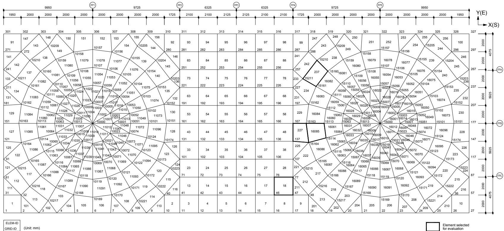
Figure 3G.4-3a. Finite Element Model of FWSC (Foundation Mat)
