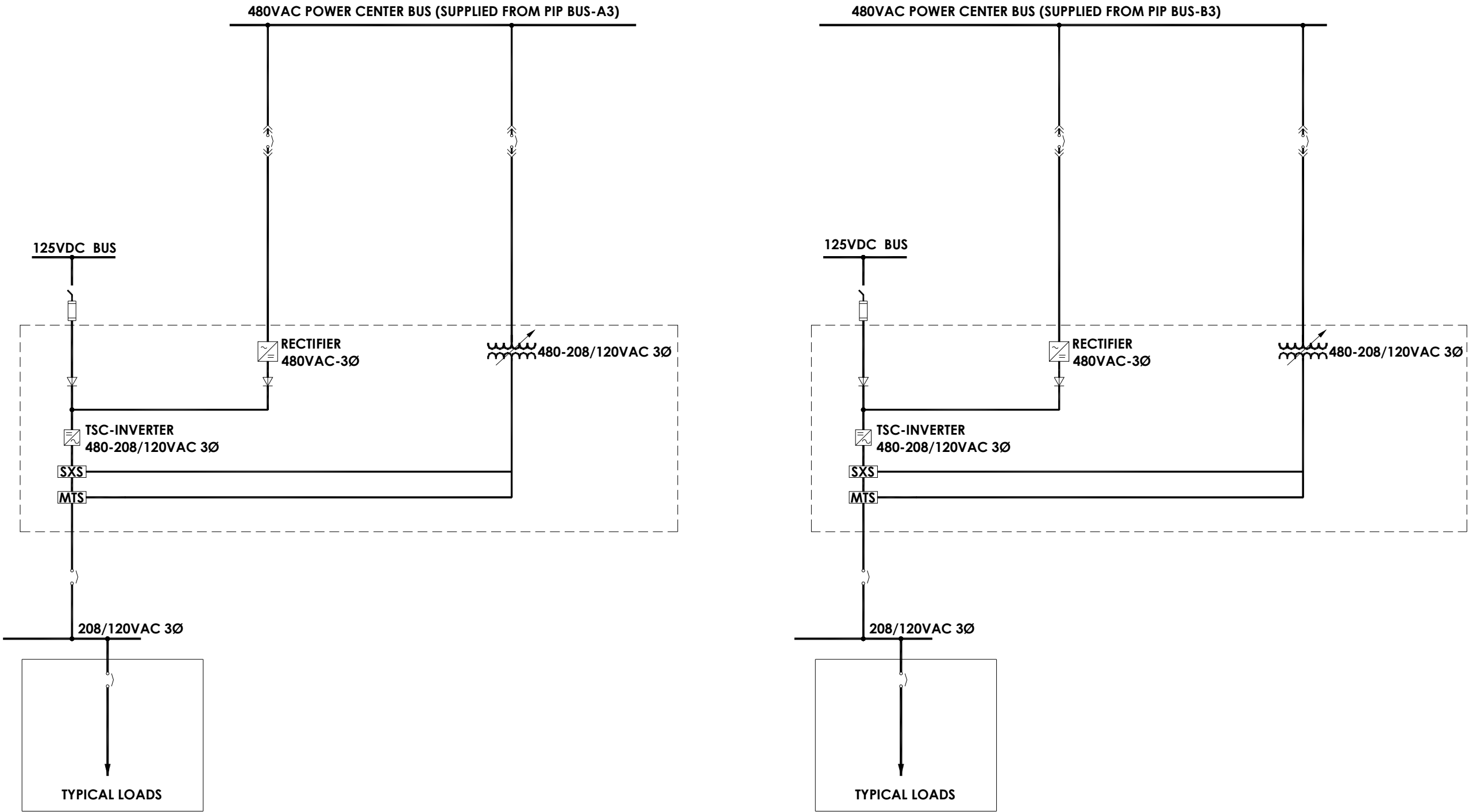
NONSAFETY-RELATED UNINTERRUPTIBLE TSC SYSTEM
