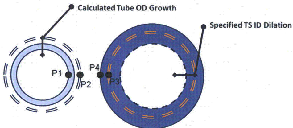
Figure 2-11 Constant Tubesheet Bore Dilation Model
