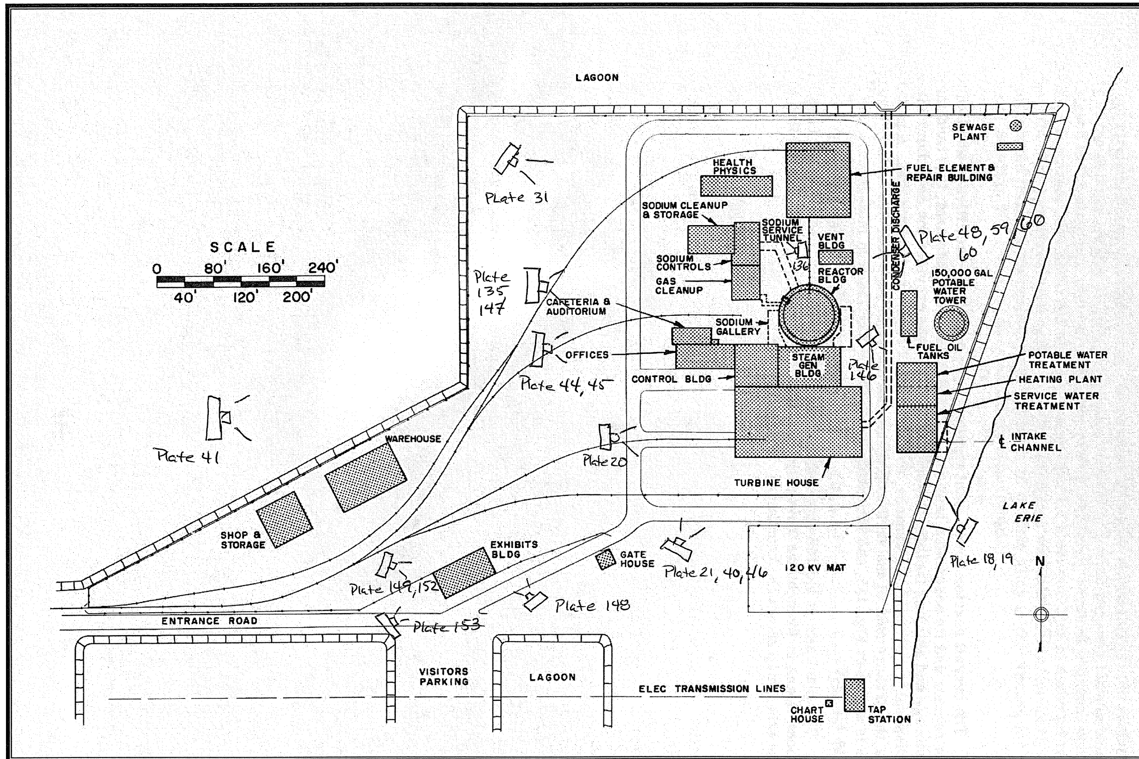
Plate 15 Site plan of power plant (Courtesy DECo)
