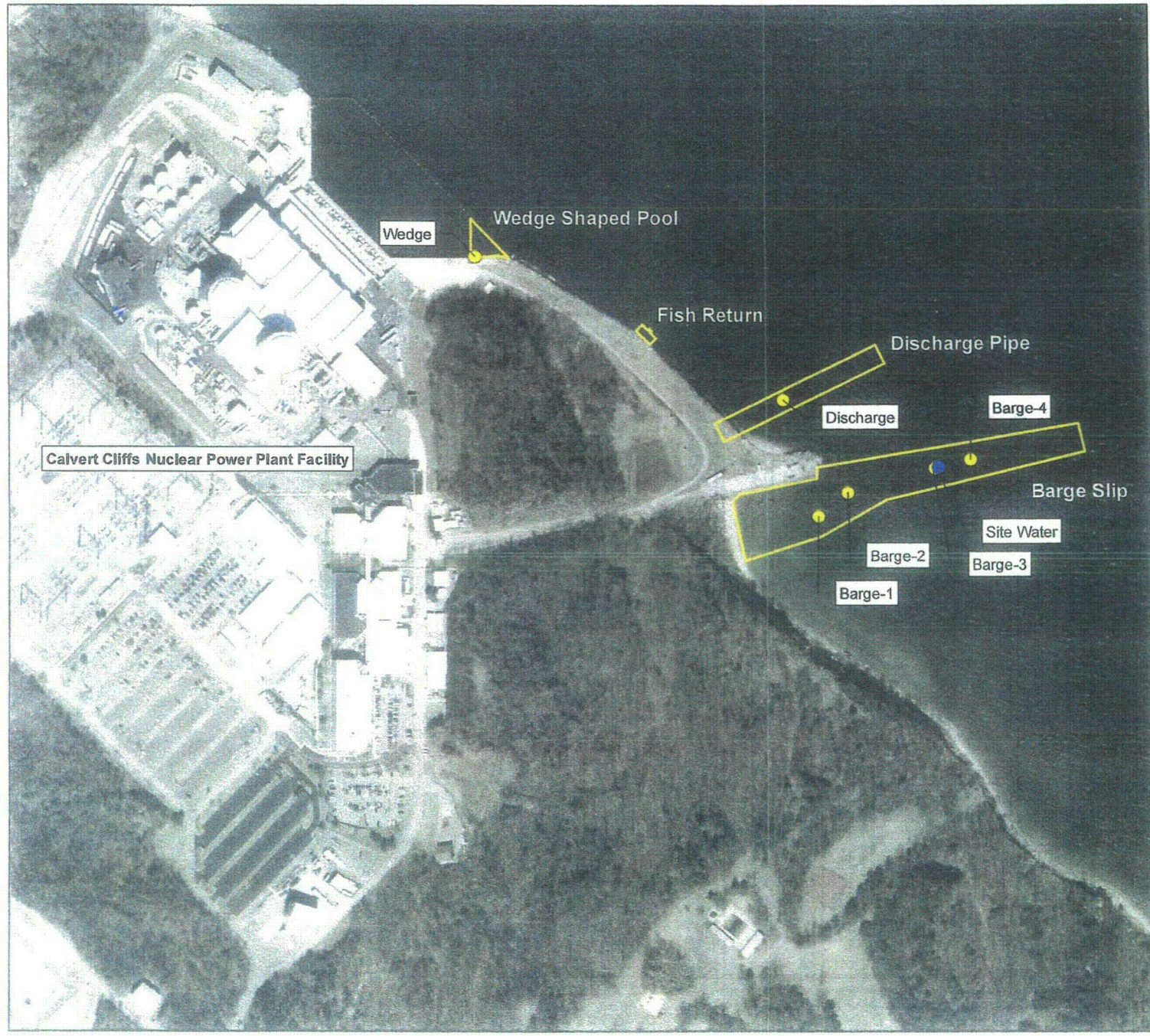
Figure 2 Proposed Dredging Areas and Project Sampling Locations
