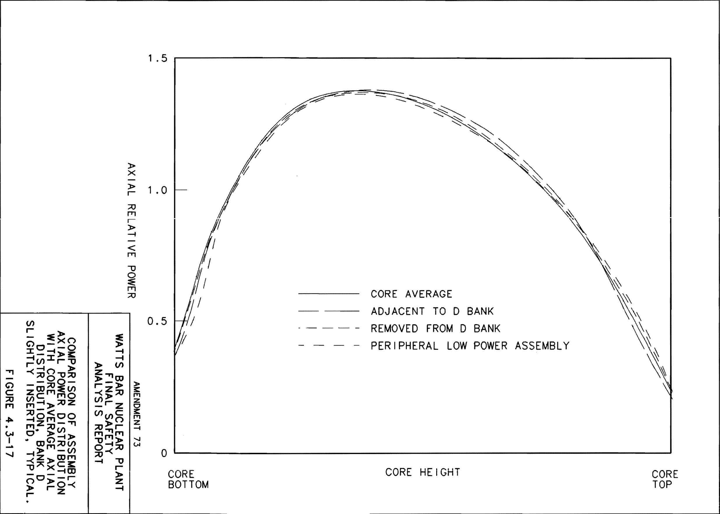
Figure 4.3-17 Comparison of Assembly Axial Power Distribution With Core Average Axial Distribution, Bank D Slightly Inserted, Typical
