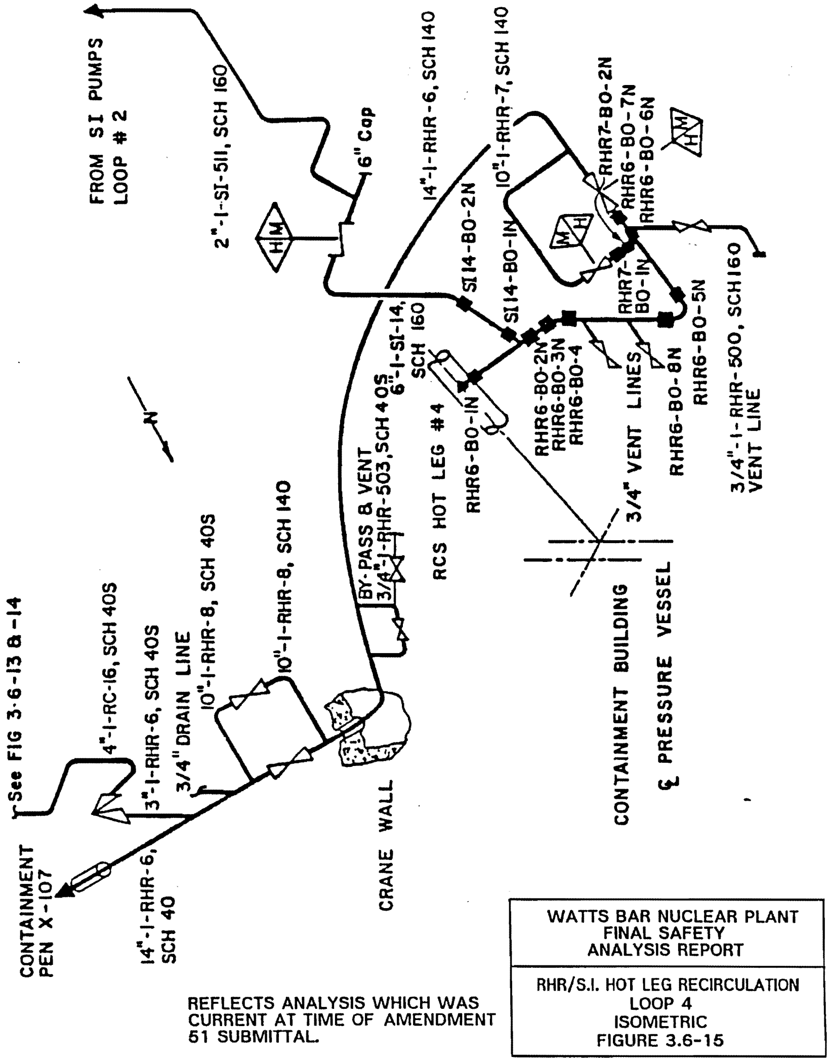
Figure 3.6-15 RHR/S.I. Hot Leg Recirculation Loop 4 Isometric
