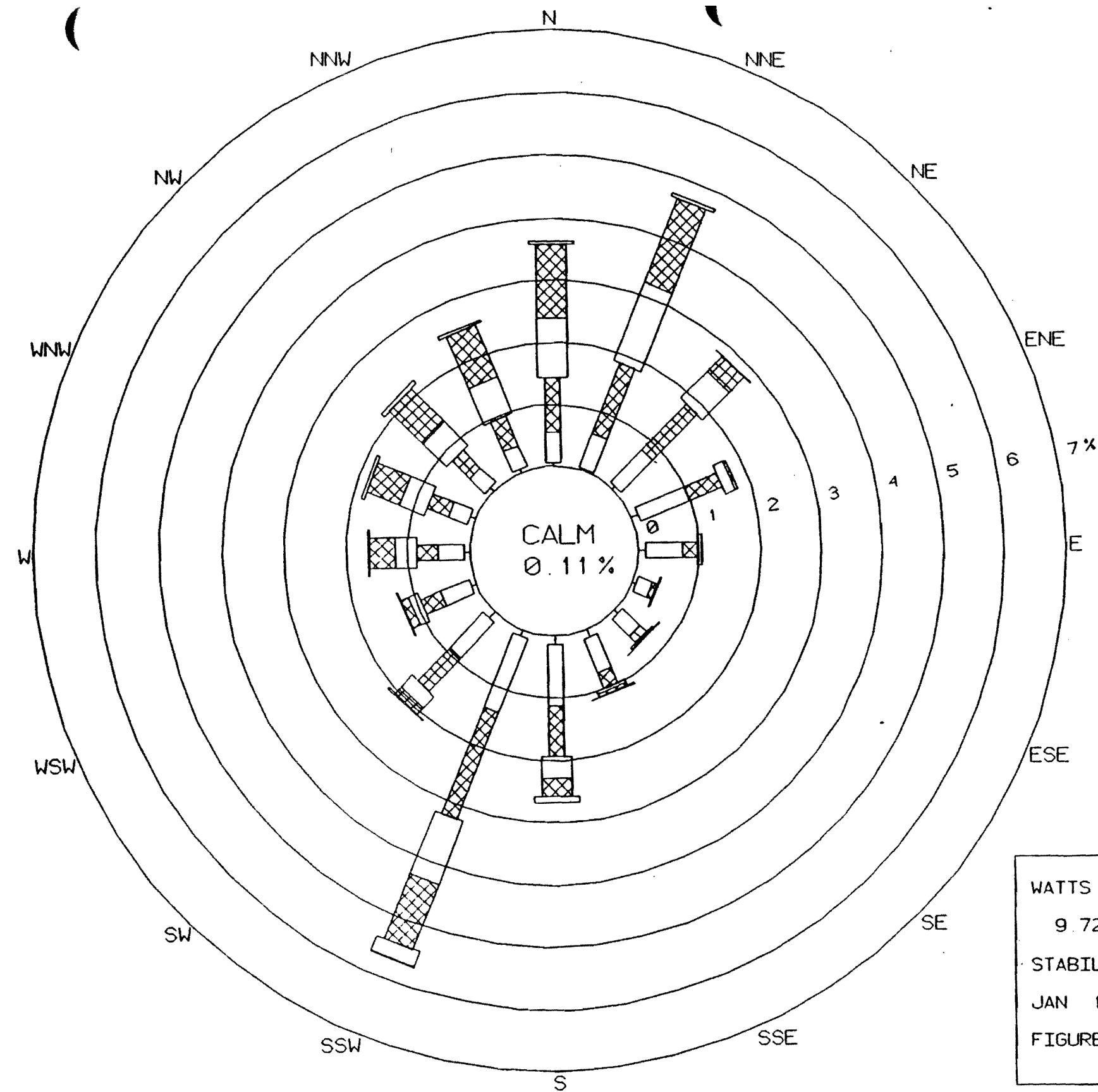
Figure 2.3-10 Wind Speed at 9.72 Meters for Stability Class D, Watts Bar Nuclear Plant, January 1, 1974 - December 31, 1993
