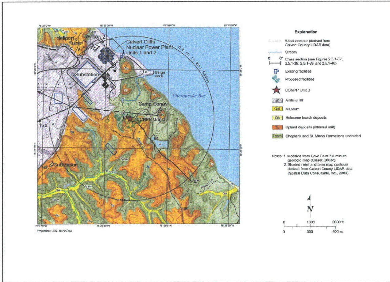
Figure 2.6-3— CCNPP Site 0.6 MI (1KM) Geologic Map
