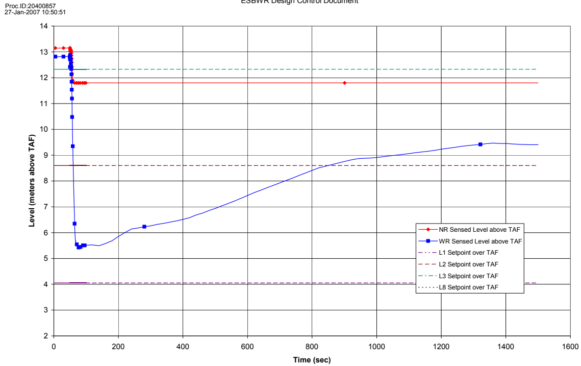
Figure 15.2-15c. Loss of Non-Emergency AC Power to Station Auxiliaries
