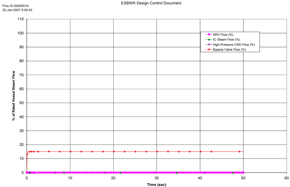
Figure 15.2-14b. Opening of One Turbine Control or Bypass Valve
