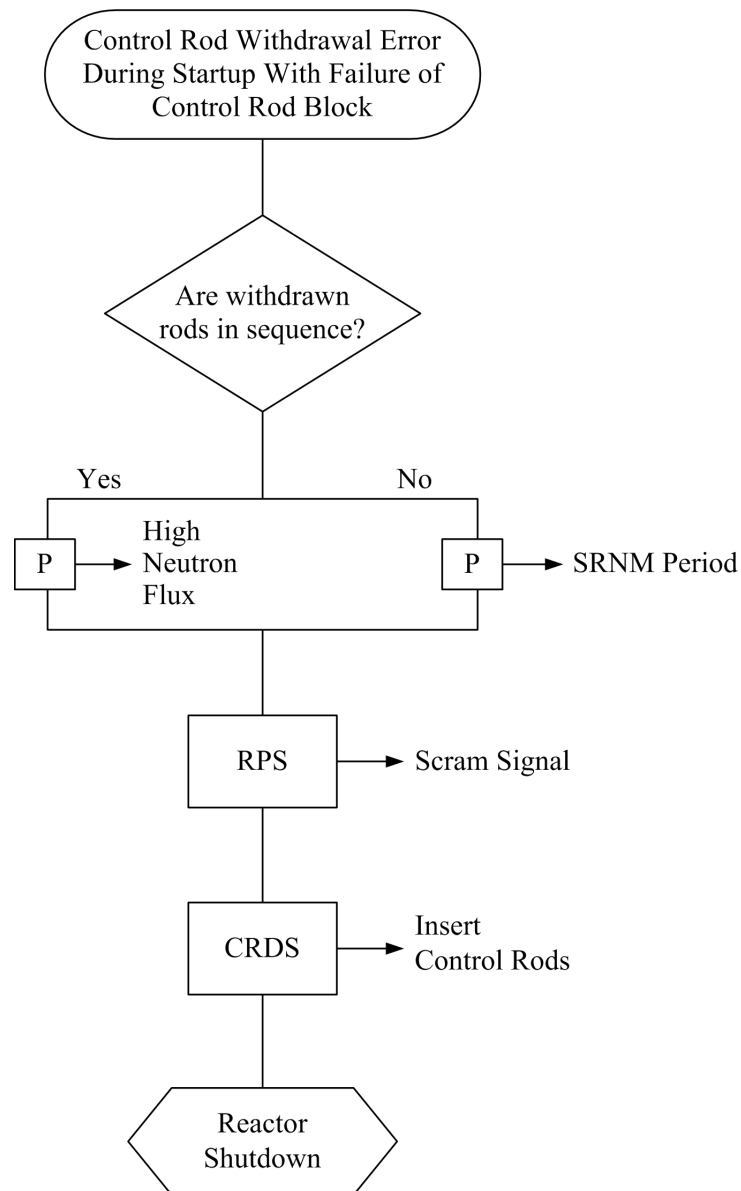
Figure 15.1-24b. Event Diagram – Control Rod Withdrawal Error During Startup With Failure of Control Rod Block
