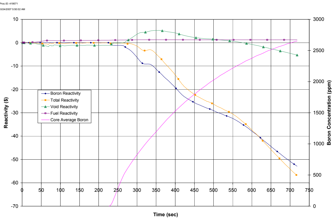
Figure 15.5-7c. ATWS Loss of Feedwater Flow with Boron Injection
