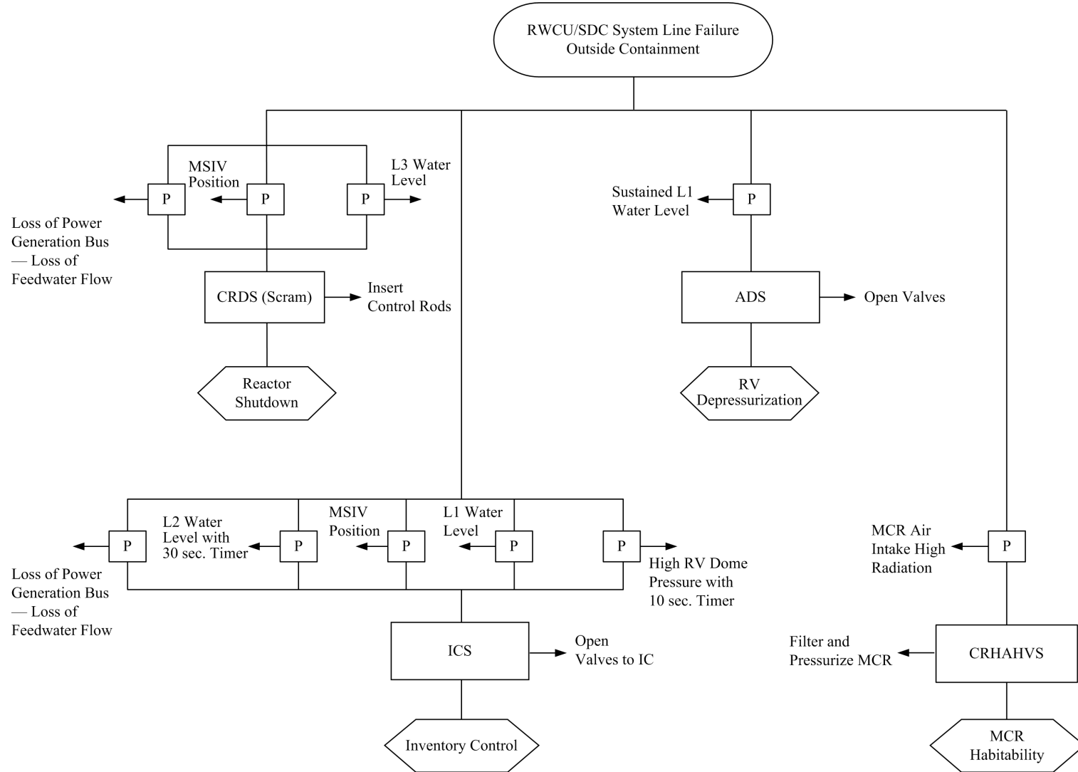
Figure 15.1-39a. Event Diagram – RWCUC/SDC System Line Failure Outside Containment
