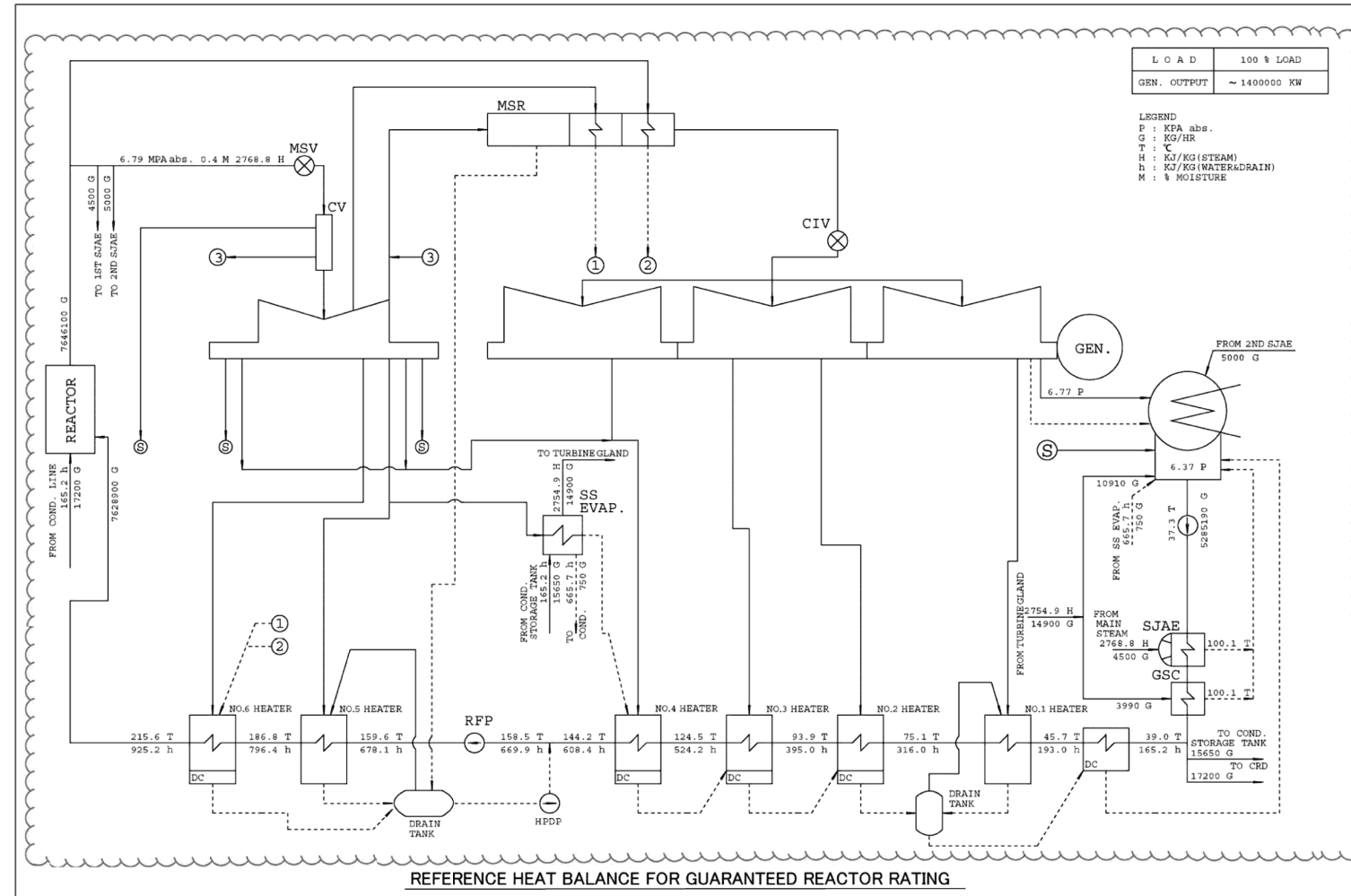
Figure 10.1-2 Reference Heat Balance for Guaranteed Reactor Rating
