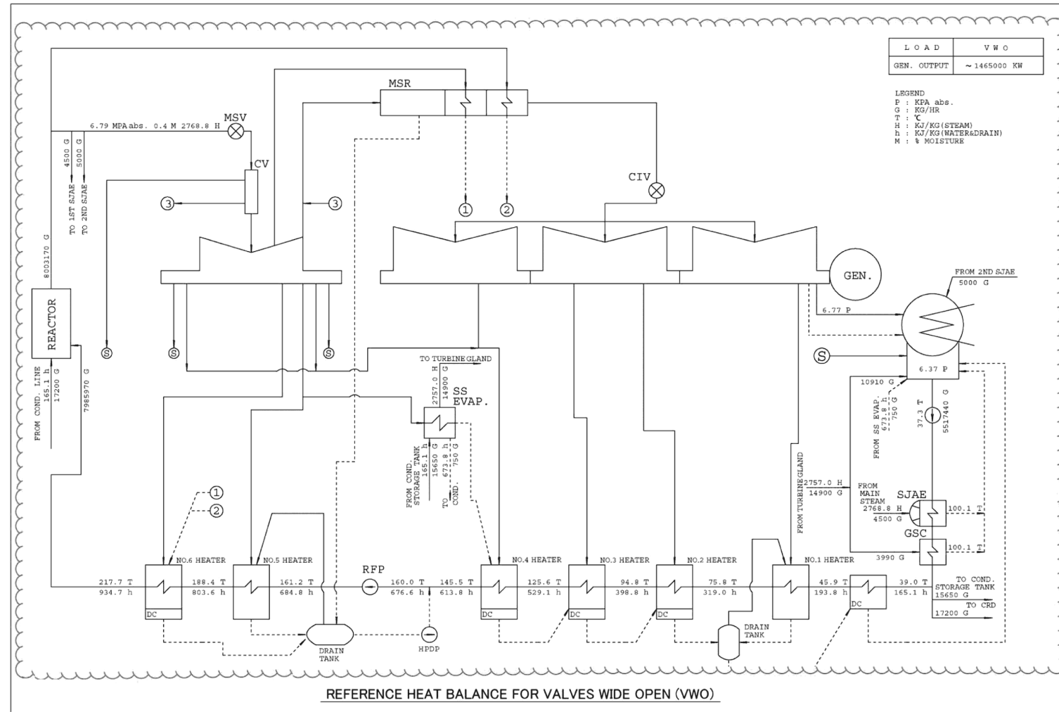
Figure 10.1-3 Reference Heat Balance for Valves-Wide-Open (VWO)
