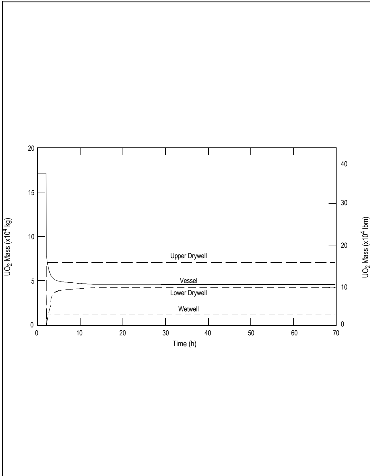
Figure 19E.2-4e LCHP-PS-R-N: Loss of all Core Cooling with Vessel Failure at High Pressure, Passive Flooder and Drywell Sprays Operate, Rupture Disk Opens: UO 2 Mass
