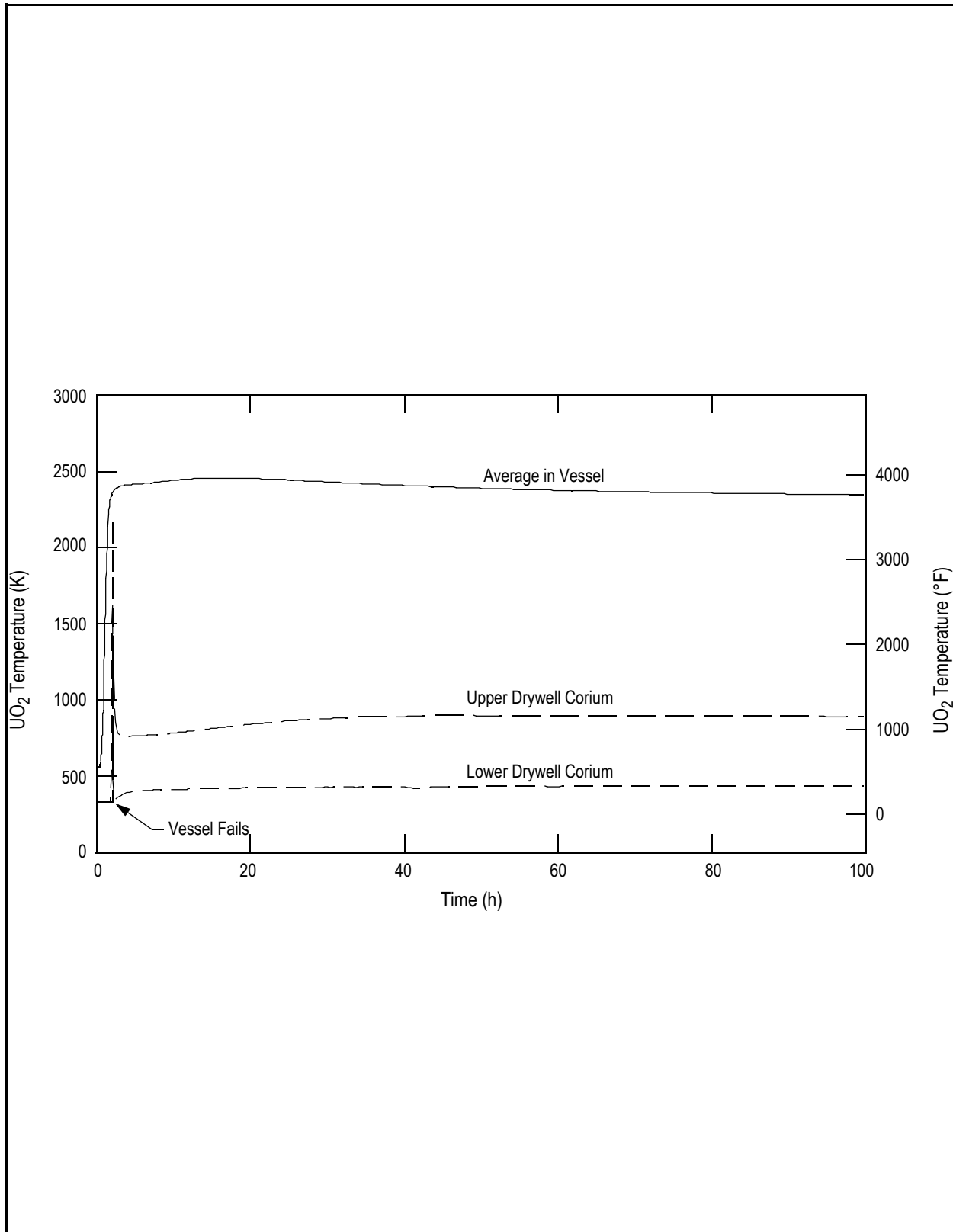
Figure 19E.2-5c LCHP-PF-P-M: Loss of all Core Cooling with Vessel Failure at High Pressure, Passive Flooder Operates, Penetration Leakage: UO 2 Temperature
