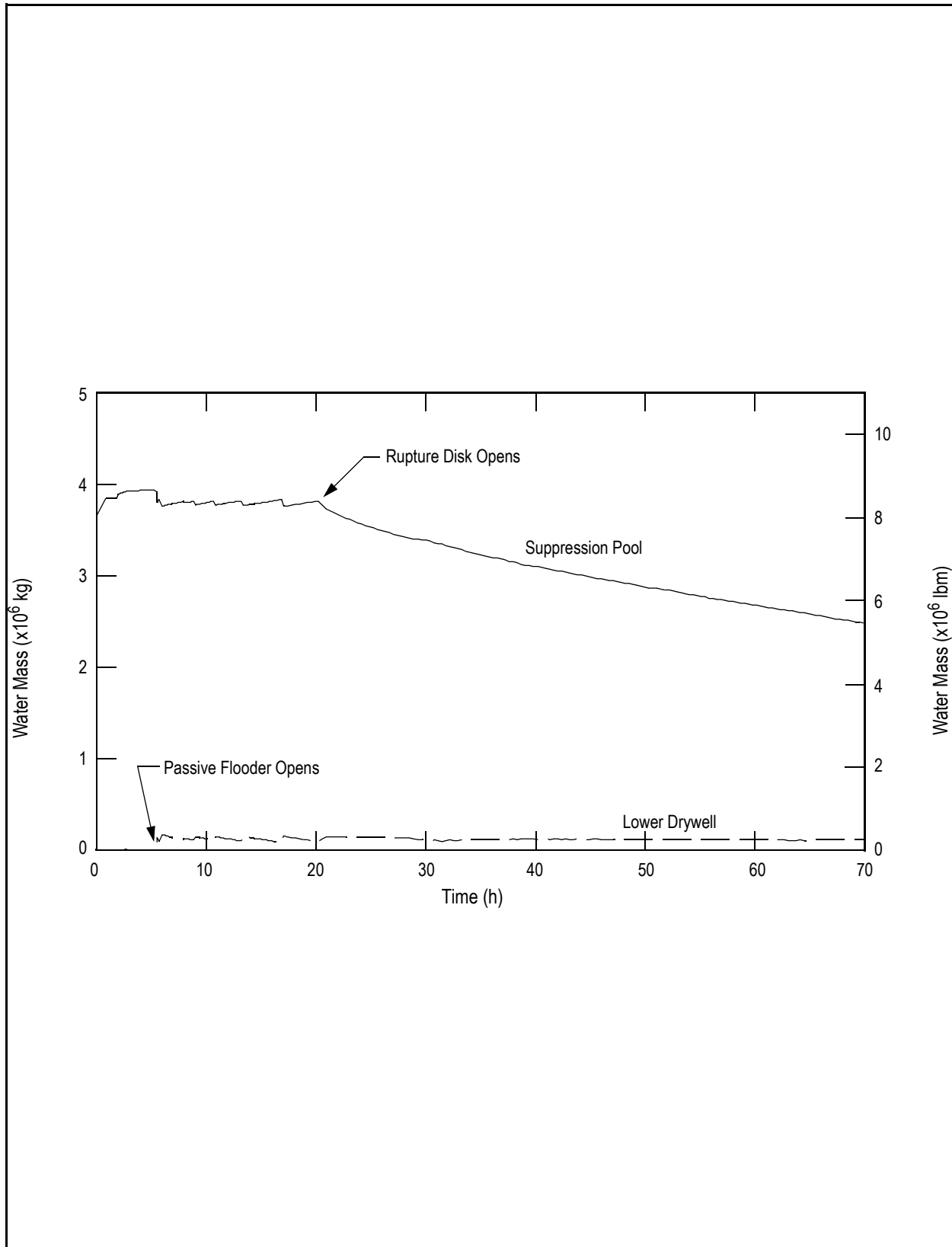
Figure 19E.2-2e LCLP-PF-R-N: Loss of all Core Cooling with Vessel Failure at Low Pressure, Passive Flooder Operates and Rupture Disk Opens: Water Mass
