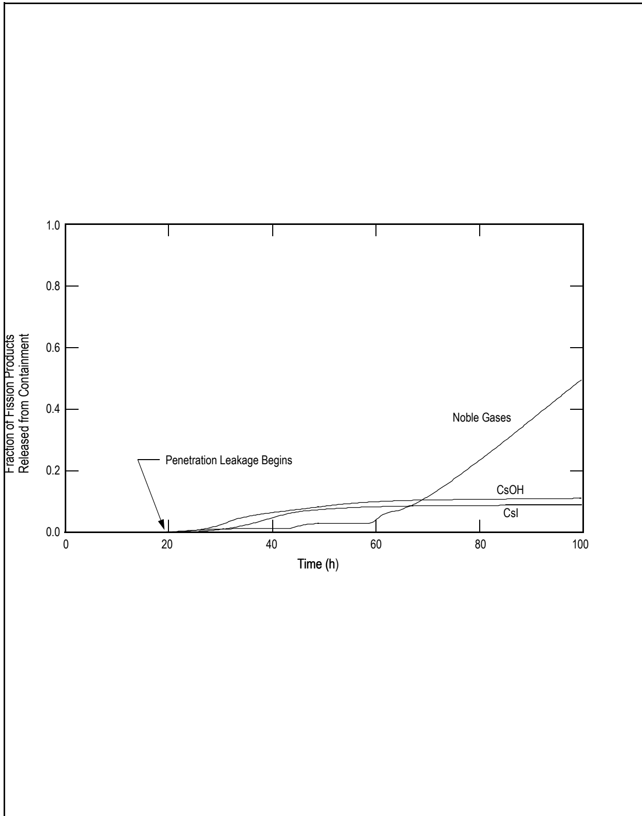
Figure 19E.2-5e LCHP-PF-P-M: Loss of all Core Cooling with Vessel Failure at High Pressure, Passive Flooder Operates, Penetration Leakage: Fission Product Release
