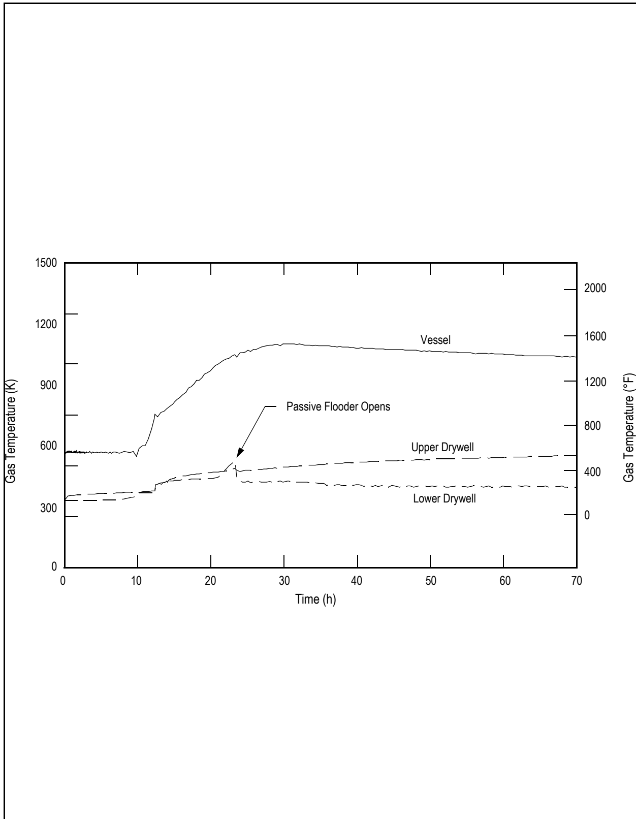
Figure 19E.2-7c SBRC-PF-R-N: Station Blackout with RCIC Operating, Passive Flooder Operates and Rupture Disk Opens: Gas Temperature
