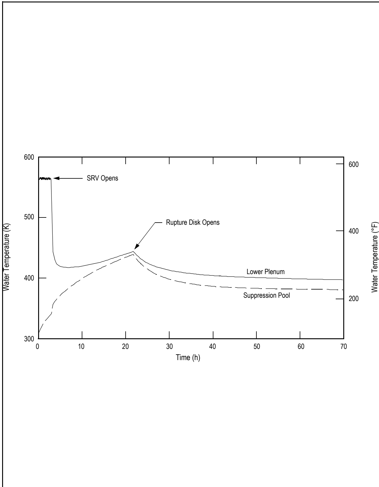
Figure 19E.2-8b LHRC-00-R-0: Isolation with Loss of Containment Heat Removal and Rupture Disk Opens: Water Temperature
