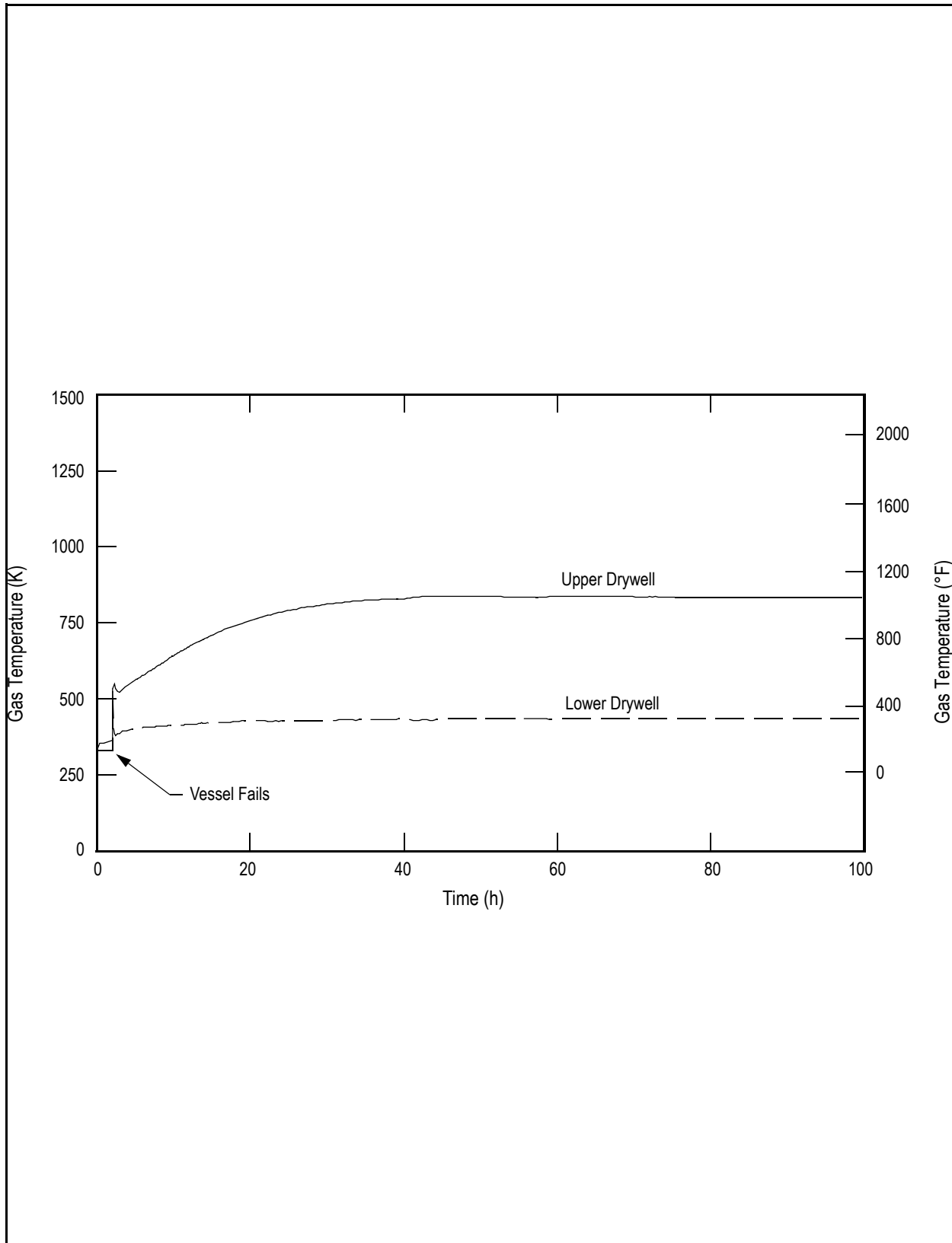
Figure 19E.2-5b LCHP-PF-P-M: Loss of all Core Cooling with Vessel Failure at High Pressure, Passive Flooder Operates, Penetration Leakage: Gas Temperature
