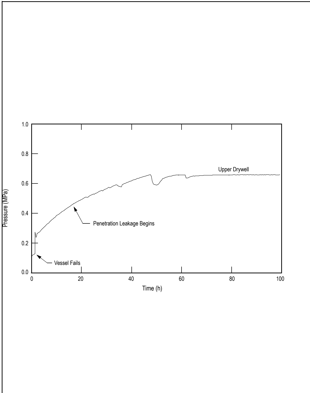
Figure 19E.2-11a NSCH-PF-P-M: Concurrent Loss of all Core Cooling and ATWS with Vessel Failure at High Pressure, Passive Flooder, Penetration Leakage: Drywell Pressure
