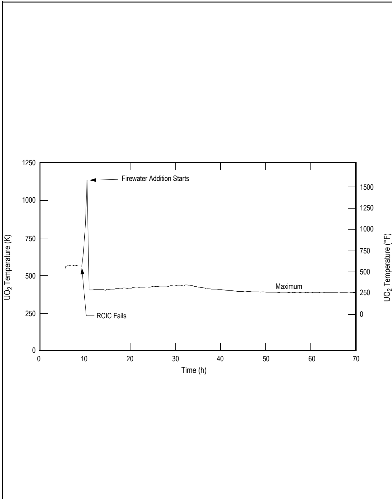
Figure 19E.2-6c SBRC-FA-R-0: Station Blackout, RCIC Runs Eight Hours, Firewater Addition Prevents Core Damage, Rupture Disk Opens: UO 2 Temperature
