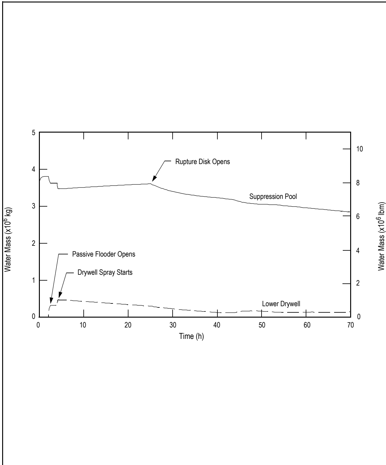
Figure 19E.2-4f LCHP-PS-R-N: Loss of all Core Cooling with Vessel Failure at High Pressure, Passive Flooder and Drywell Sprays Operate, Rupture Disk Opens: Water Mass
