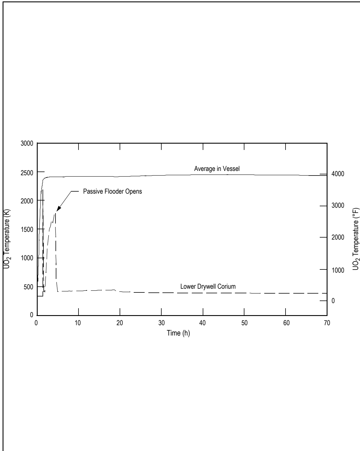
Figure 19E.2-10b NSCL-PF-R-N: Concurrent Loss of all Core Cooling and ATWS with Vessel Failure at Low Pressure, Passive Flooder and Rupture Disk: UO 2 Temperature
