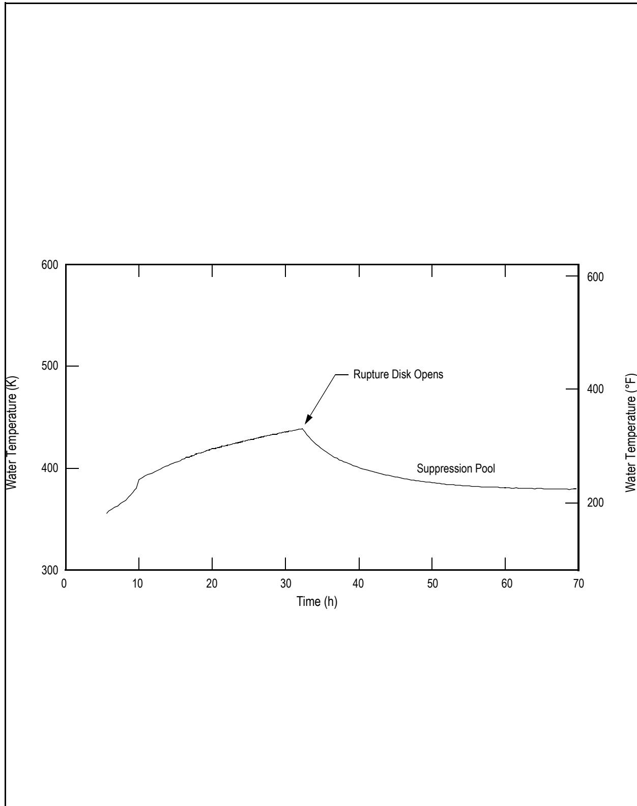
Figure 19E.2-6b SBRC-FA-R-0: Station Blackout, RCIC Runs Eight Hours, Firewater Addition Prevents Core Damage, Rupture Disk Opens: Water Temperature
