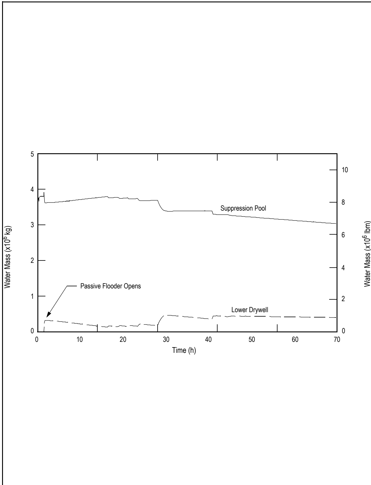
Figure 19E.2-5d LCHP-PF-P-M: Loss of all Core Cooling with Vessel Failure at High Pressure, Passive Flooder Operates, Penetration Leakage: Water Mass
