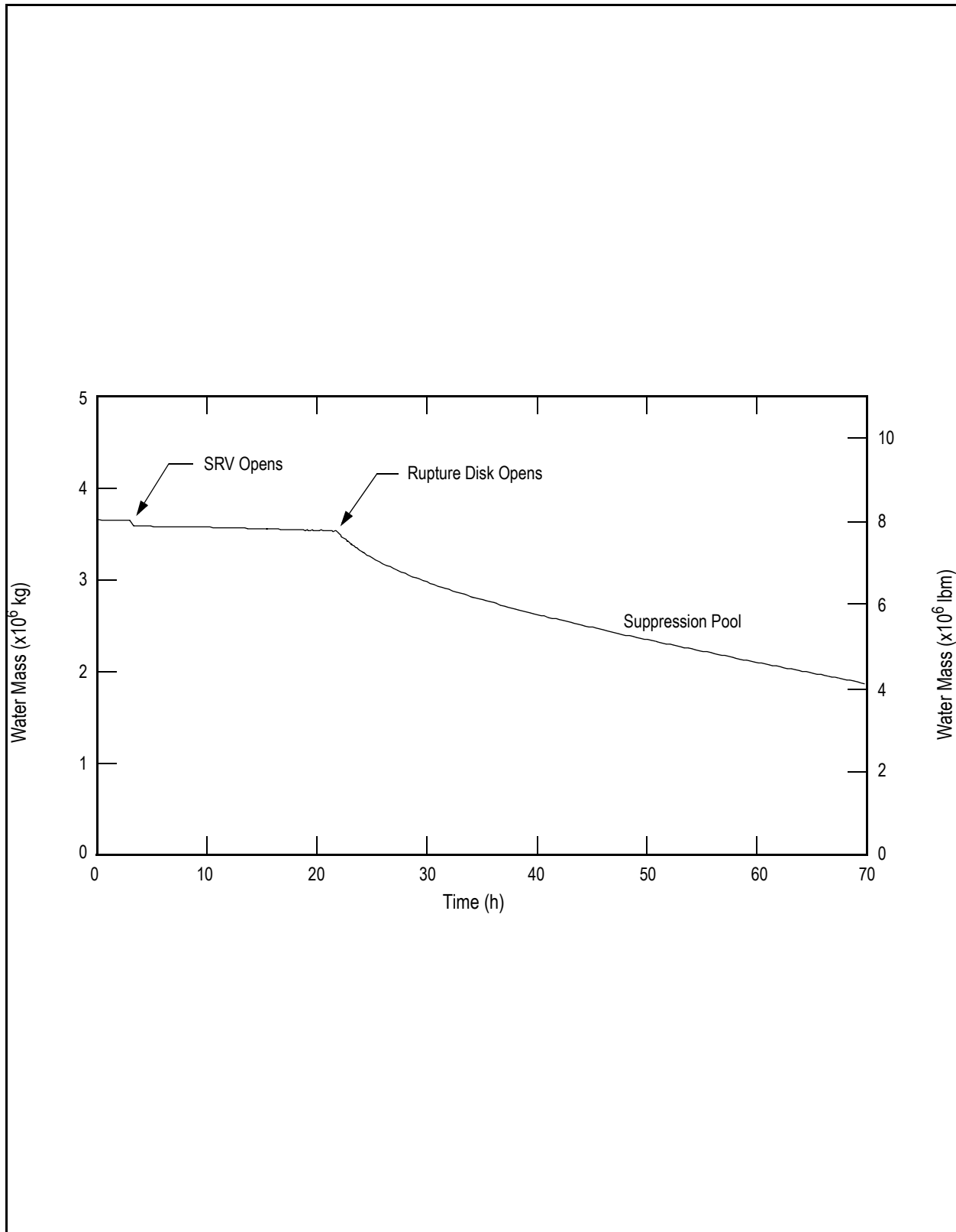
Figure 19E.2-8c LHRC-00-R-0: Isolation with Loss of Containment Heat Removal and Rupture Disk Opens: Water Mass
