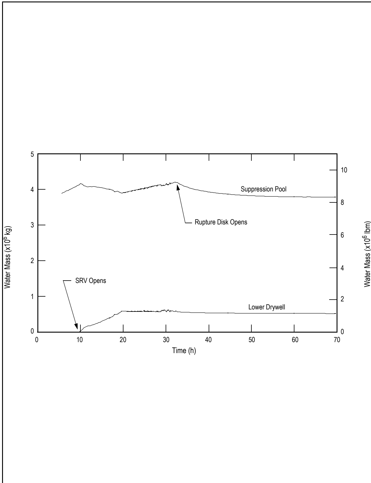
Figure 19E.2-6e SBRC-FA-R-0: Station Blackout, RCIC Runs Eight Hours, Firewater Addition Prevents Core Damage, Rupture Disk Opens: Water Mass
