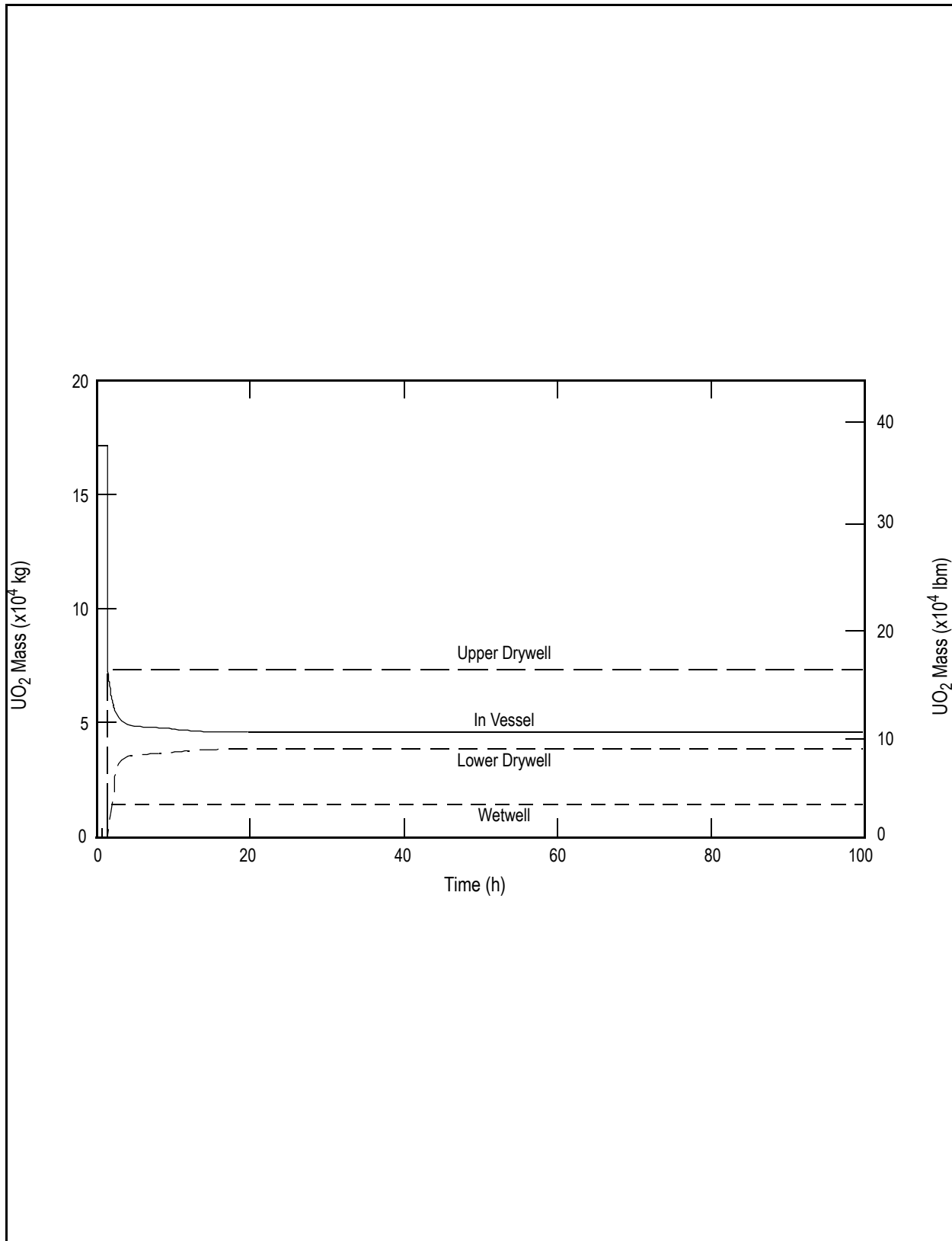
Figure 19E.2-11c NSCH-PF-P-M: Concurrent Loss of all Core Cooling and ATWS with Vessel Failure at High Pressure, Passive Flooder, Penetration Leakage: UO 2 Mass
