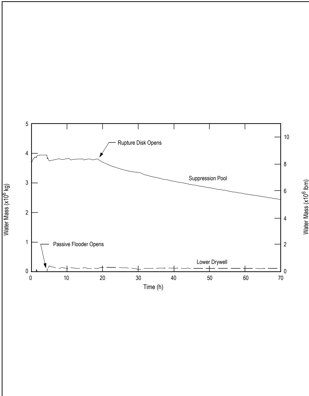
Figure 19E.2-10c NSCL-PF-R-N: Concurrent Loss of all Core Cooling and ATWS with Vessel Failure at Low Pressure, Passive Flooder and Rupture Disk: Water Mass
