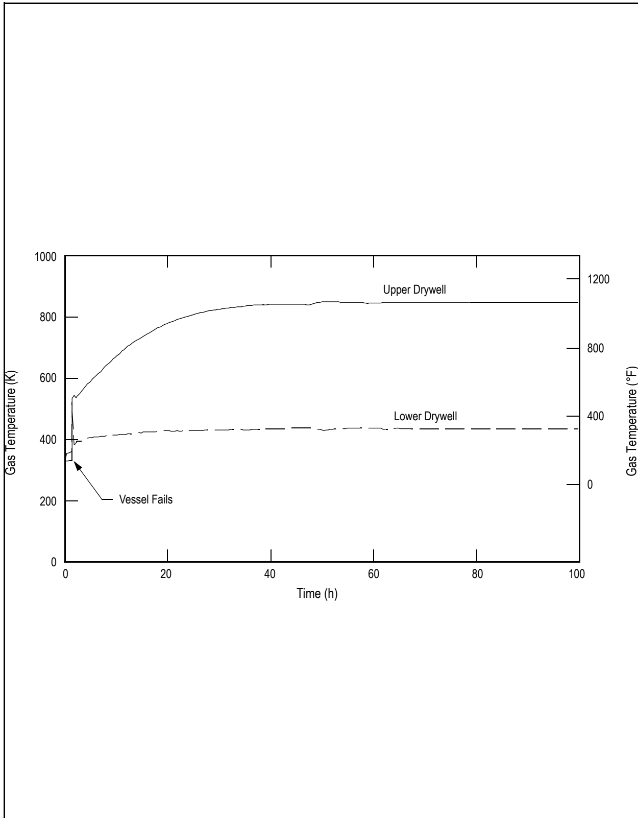
Figure 19E.2-11b NSCH-PF-M: Concurrent Loss of all Core Cooling and ATWS with Vessel Failure at High Pressure, Passive Flooder, Penetration Leakage Rupture Disk Opens: Gas Temperature
