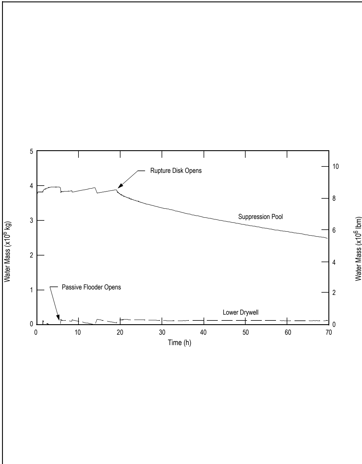
Figure 19E.2-9c LBLC-PF-R-N: Large Break LOCA with Loss of all Core Cooling, Passive Flooder Operates and Rupture Disk Opens: Water Mass
