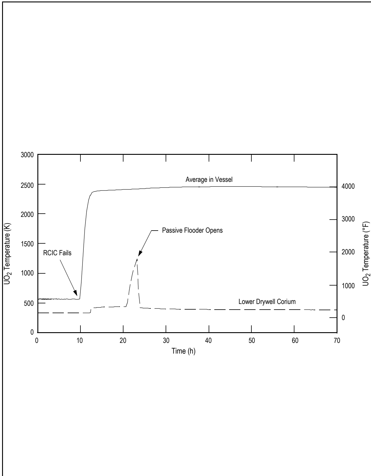
Figure 19E.2-7d SBRC-PF-R-N: Station Blackout with RCIC Operating, Passive Flooder Operates and Rupture Disk Opens: UO 2 Temperature
