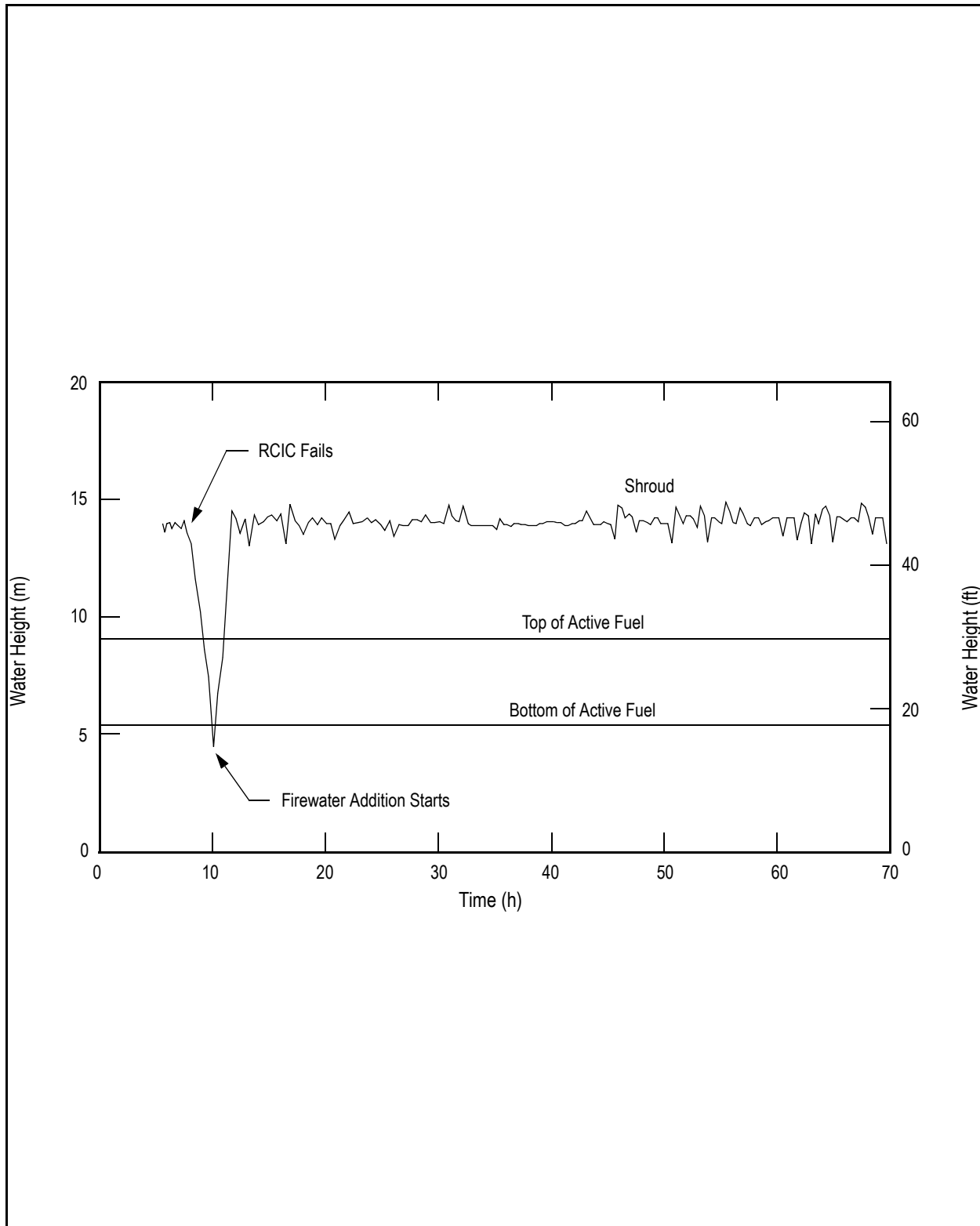
Figure 19E.2-6d SBRC-FA-R-0: Station Blackout, RCIC Runs Eight Hours, Firewater Addition Prevents Core Damage, Rupture Disk Opens: Vessel Water Height
