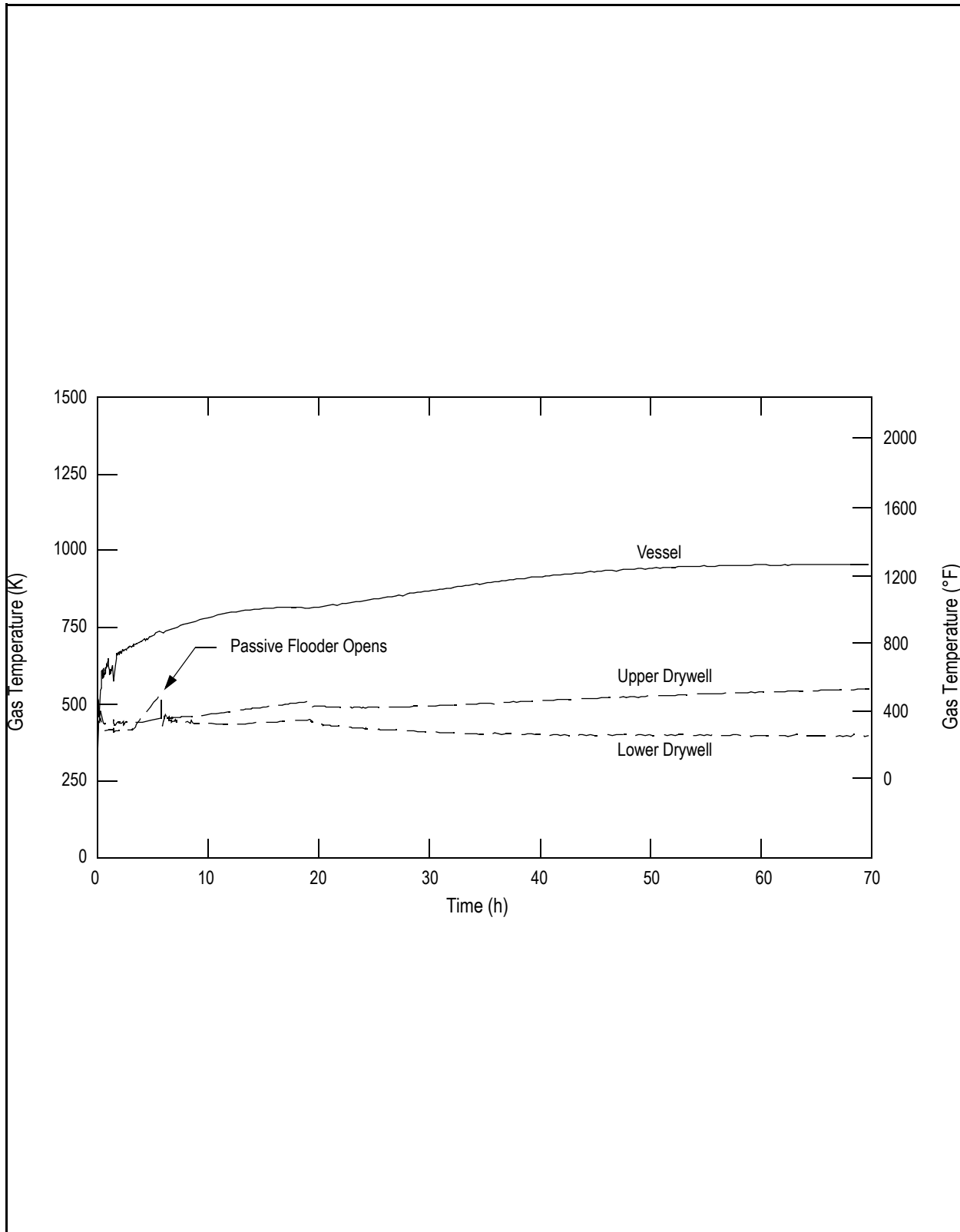
Figure 19E.2-9b LBLIC-PF-R-N: Large Break LOCA with Loss of all Core Cooling, Passive Flooder Operates and Rupture Disk Opens: Gas Temperature
