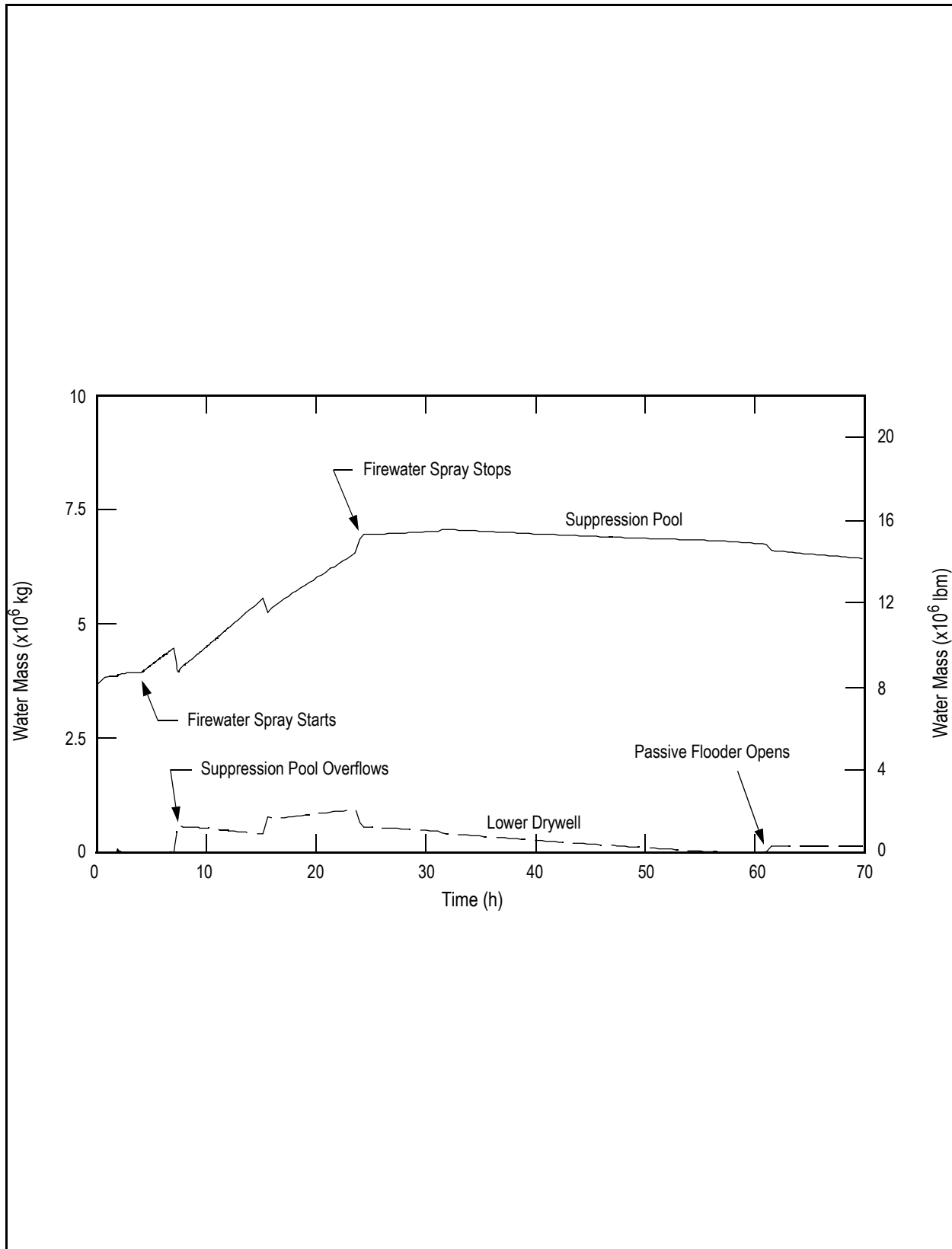
Figure 19E.2-3c LCLP-FS-R-N: Loss of all Core Cooling with Vessel Failure at Low Pressure, Firewater Spray Operates and Rupture Disk Opens: Water Mass
