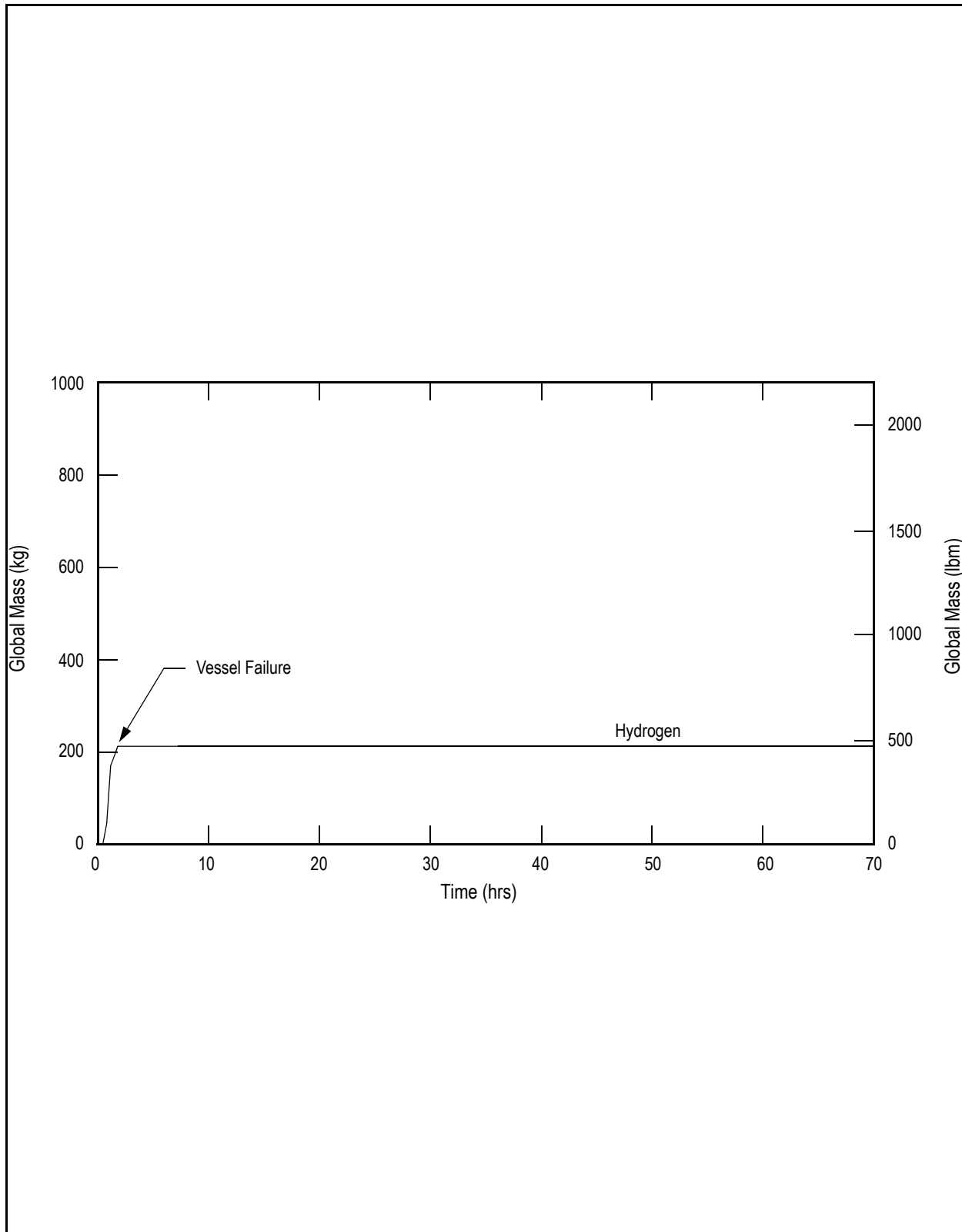
Figure 19E.2-2f LCLP-PF-R-N: Loss of all Core Cooling with Vessel Failure at Low Pressure, Passive Flooder Operates and Rupture Disk Opens: Mass of Non-Condensables
