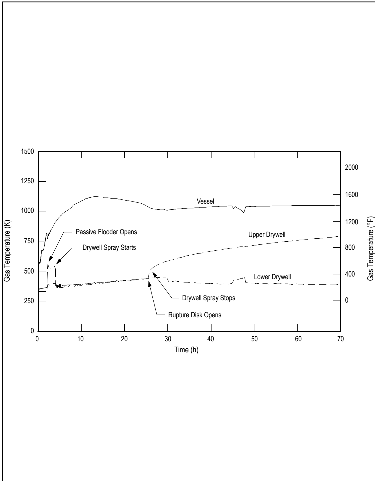
Figure 19E.2-4d LCHP-PS-R-N: Loss of all Core Cooling with Vessel Failure at High Pressure, Passive Flooder and Drywell Sprays Operate, Rupture Disk Opens: Gas Temperature
