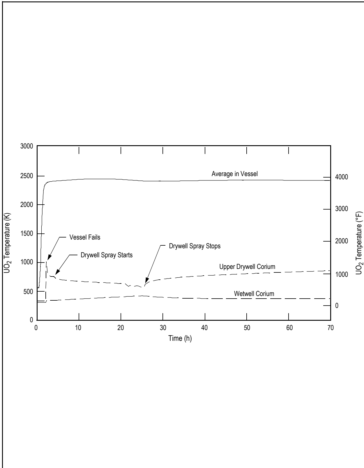
Figure 19E.2-4c LCHP-PS-R-N: Loss of all Core Cooling with Vessel Failure at High Pressure, Passive Flooder and Drywell Sprays Operate, Rupture Disk Opens: UO 2 Temperature
