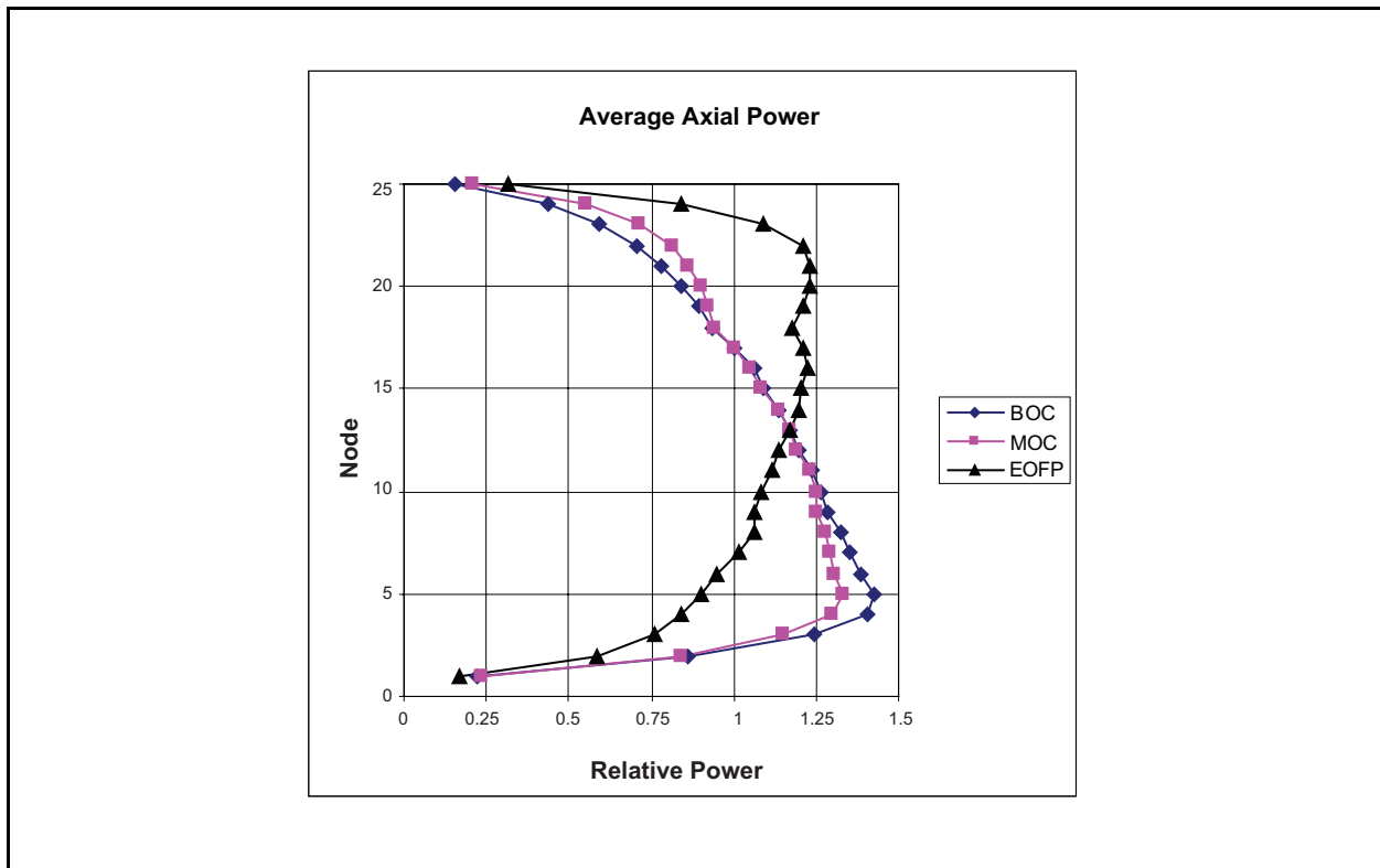
Figure 4A-3b Axial Power Distribution at BOC, MOC and EOFP
