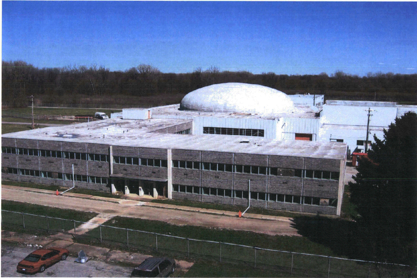
Exhibit 1, View of PBRF Showing ROLB and Reactor Building
