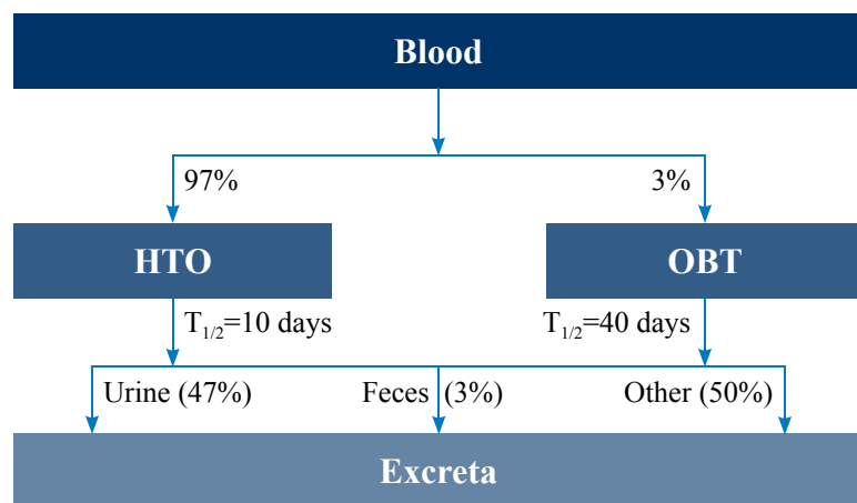
Figure 6.1: ICRP Model for the Biokinetics of Tritiated Water
