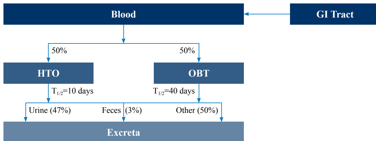
Figure 6.2: ICRP Model for the Biokinetics of Organically Bound Tritium
