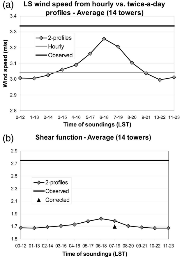
FIG. 10. (a) Observed winds, calculated from hourly V_{\text{ref}} , and calculated from daily averages of V_{\text{ref}} with 2-times-per-day soundings values of LS wind speed, averaged over all two-level towers of the KSC network. (b) Values of the shear function \rho averaged over all hours and all KSC two-level towers obtained with all 12-h-apart pairs of sounding times. The value obtained with correction factors at 0700–1900 LST (corresponding to 0000 and 1200 UTC in Florida) is shown with a rhomboidal mark. Reproduced from Archer and Jacobson (2006).
