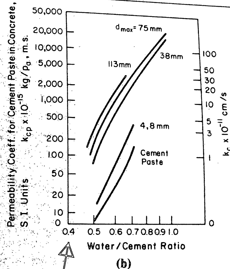
Figure 5-2 Influence of water/cement ratio and maximum aggregate size on concrete permeability: (a) K_q is a relative measure of the flow of water through concrete in cubic feet per year per square foot of area for a unit hydraulic gradient. [(a), From Concrete Manual, 8th Edition , U.S. Bureau of Reclamation, 1975, p. 37, (b), adapted from Beton-Bogen , Aalborg Cement Co., Aalborg, Denmark, 1979.]
