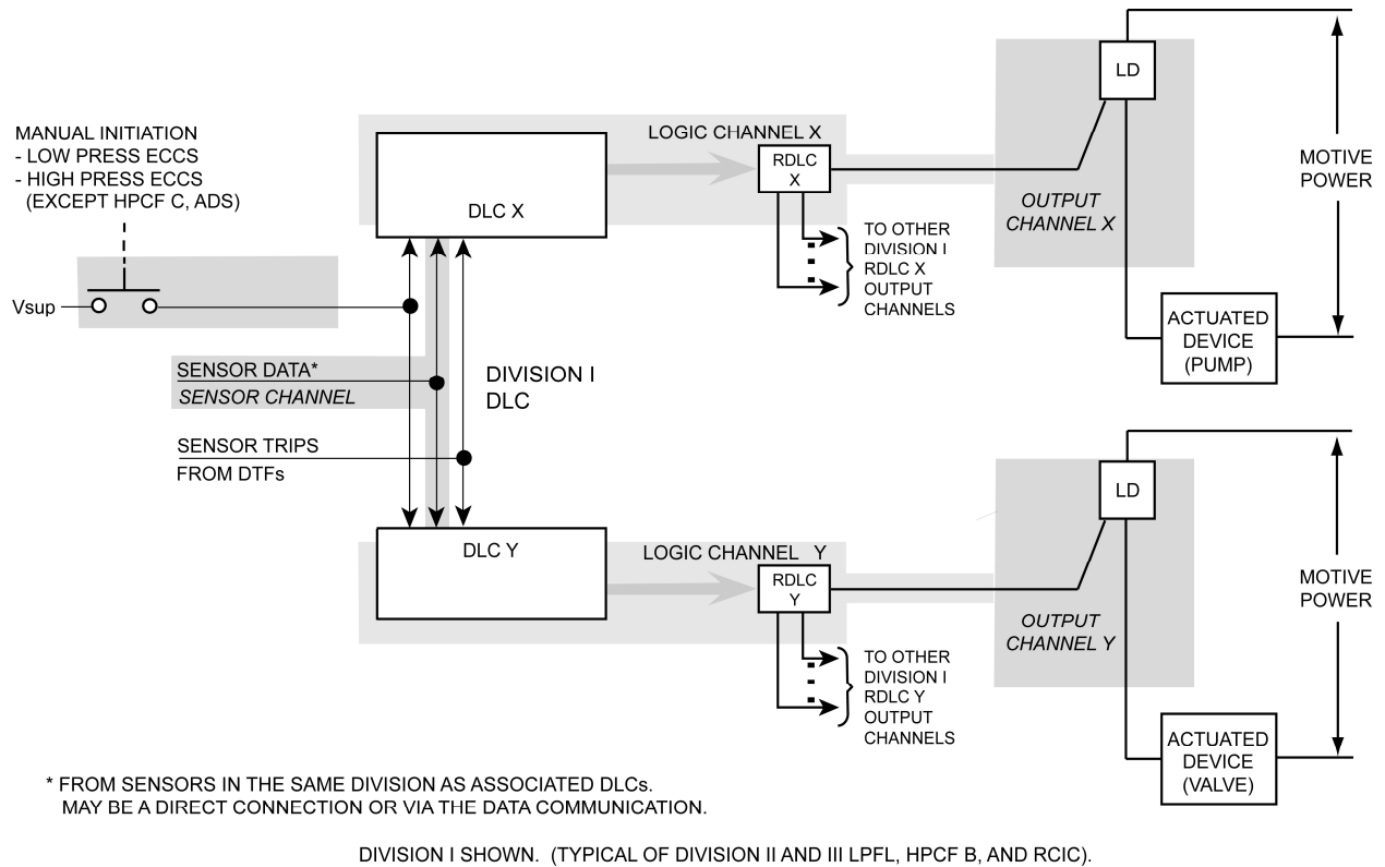
Figure B 3.3.1.4-2 ESF Actuation Channel Structure for LPFL B, C, HPCF B, RCIC
