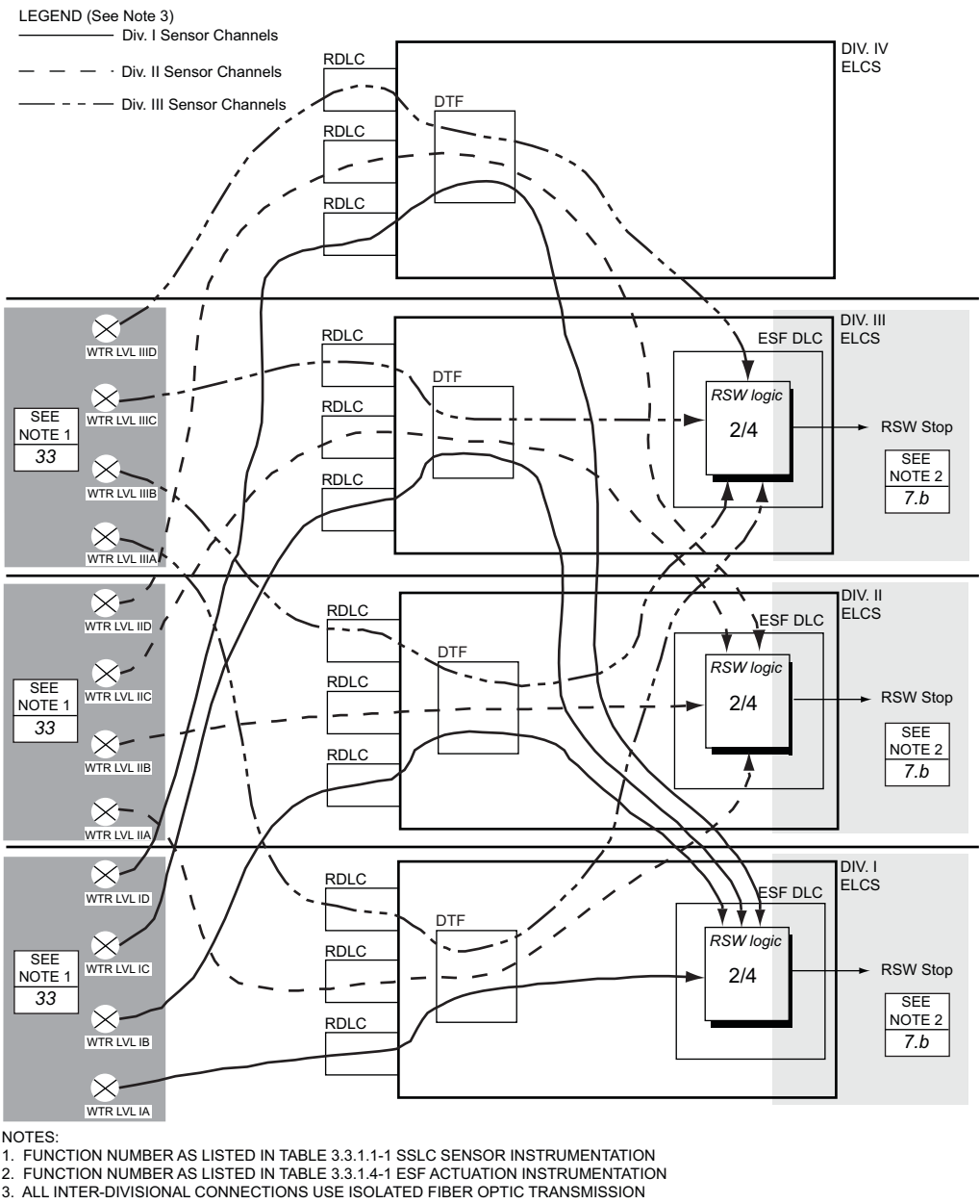
FIGURE B 3.3.1.1-2 RCW/RSW HX ROOM LEAK DETECTION INSTRUMENTATION CHANNELS
