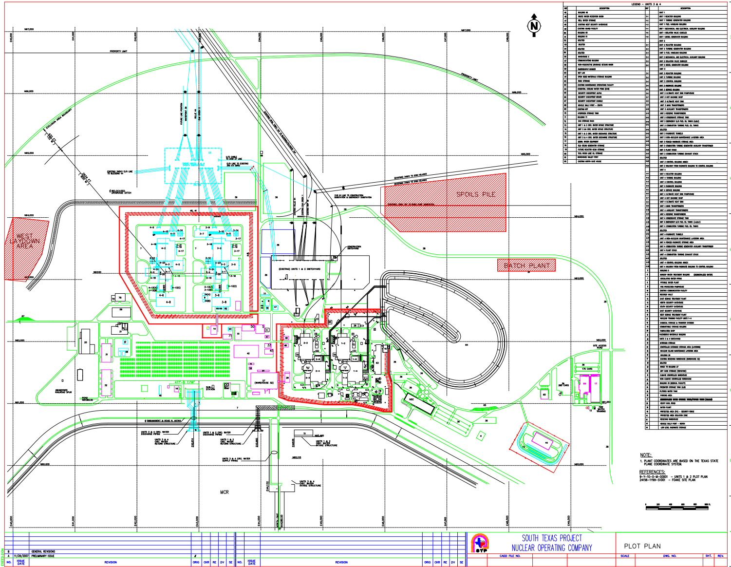
Figure 1.1-1 Site Layout
