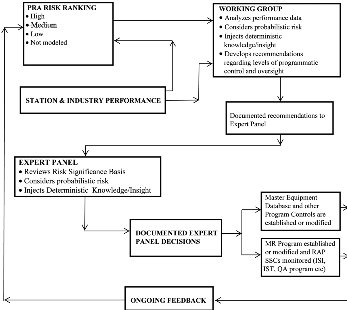
Figure 17.4S-1 Reliability Assurance Process
