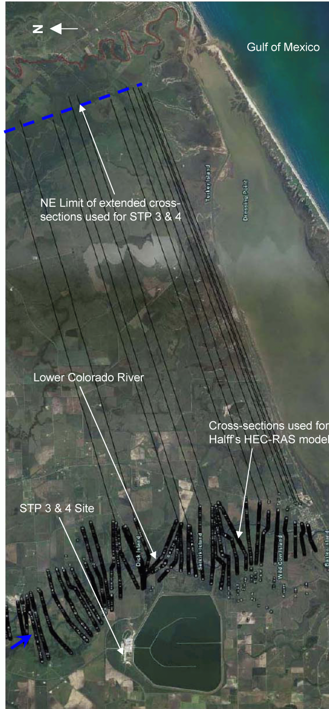
Figure 2.4S.3-10 Extended Cross sections – Most downstream section to STP 3 & 4 Site
