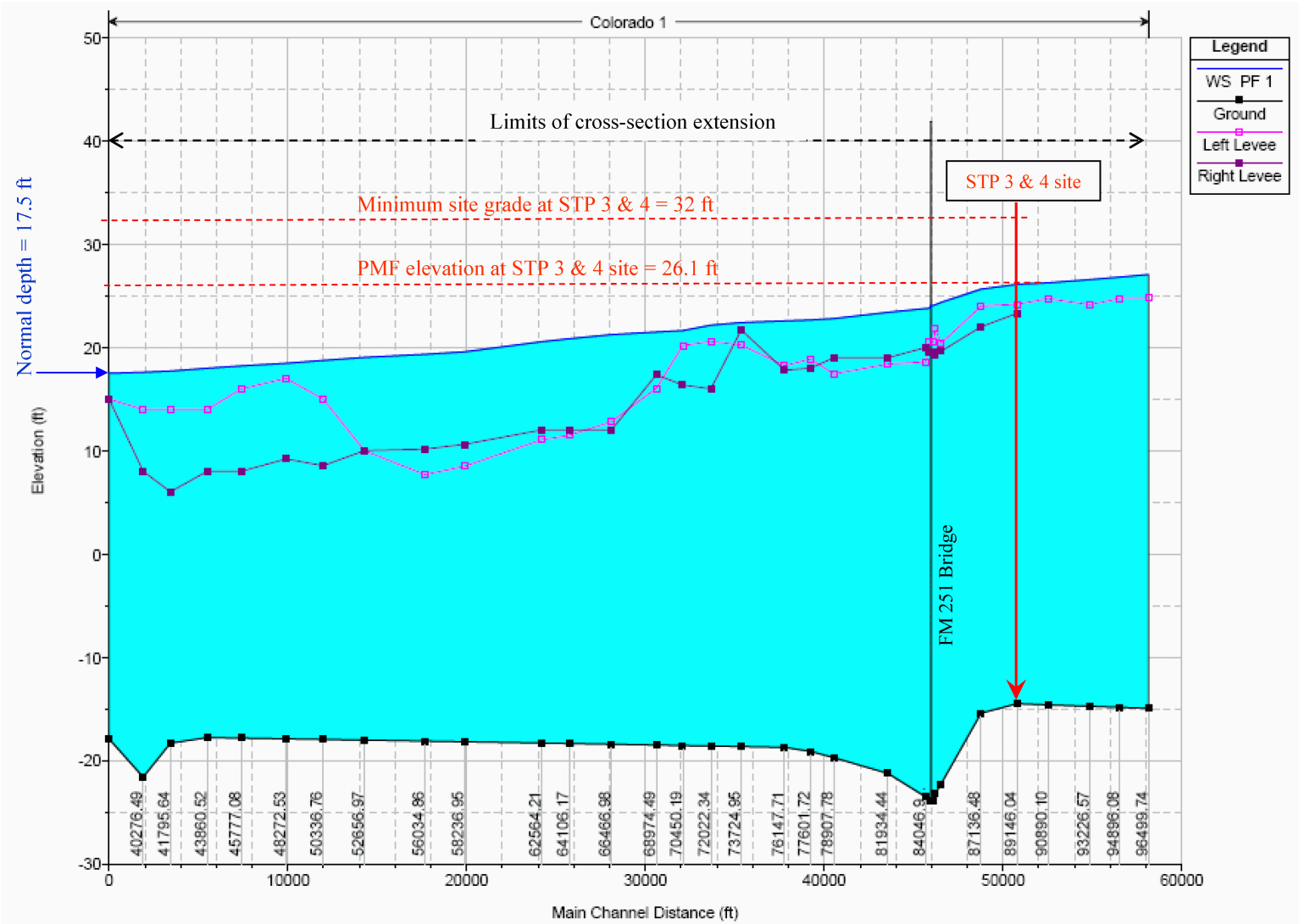
Figure 2.4S.3-11 PMF Elevation at STP 3 & 4 Site for Normal Depth Boundary Condition (Manning's n values equal to 1.2 times those used in the Half model)
