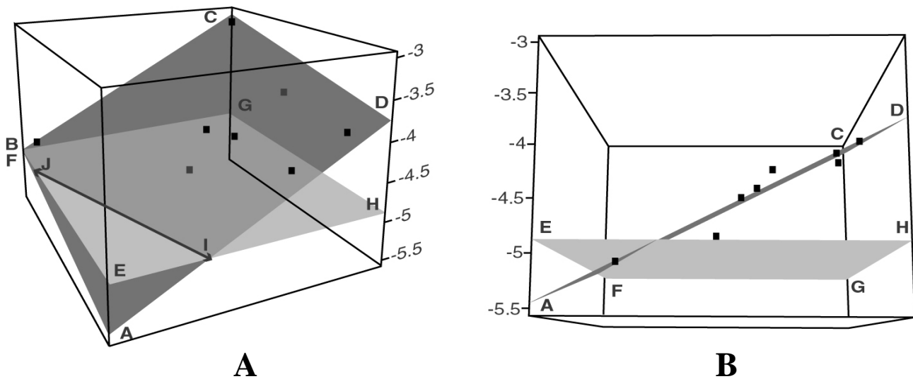
Figure 5. (A) 3D view of fault plane (ABCD) as defined by hypocenters (filled black squares) looking northeast. The intersection of a horizontal plane (EFGH) with the fault plane defines the strike (IJ) of the fault plane as 342^\circ dipping approximately 32^\circ to the southwest. (B) View of Figure 5A looking north showing side view of fault plane (AD) from a point below the surface illustrating fit of hypocenters to fault plane. Errors in depth estimates are approximately \pm 0.5 km for all events except two (Table 1). Vertical scale is kilometers below surface.
