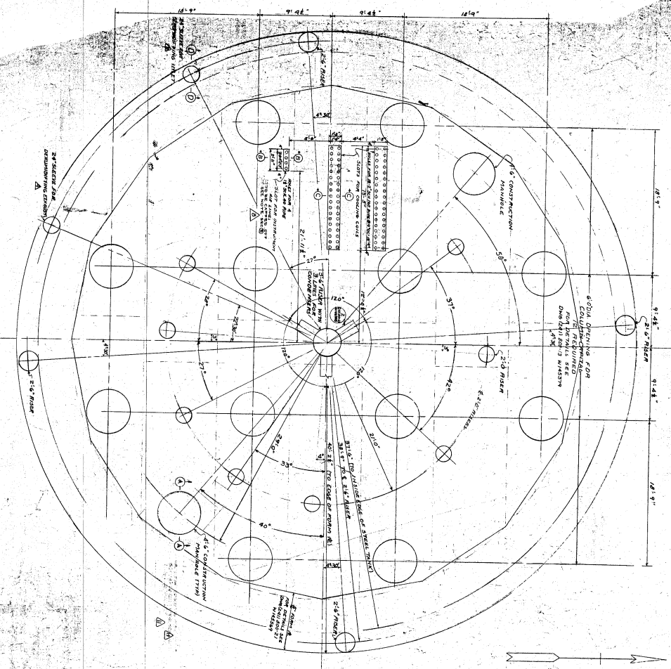
PLAN OF TOP 75' DIAMETER STEEL TANKS 1.3.79-II
