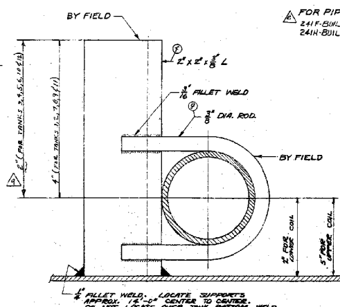
TYPICAL COIL SUPPORT SECTION (A)
