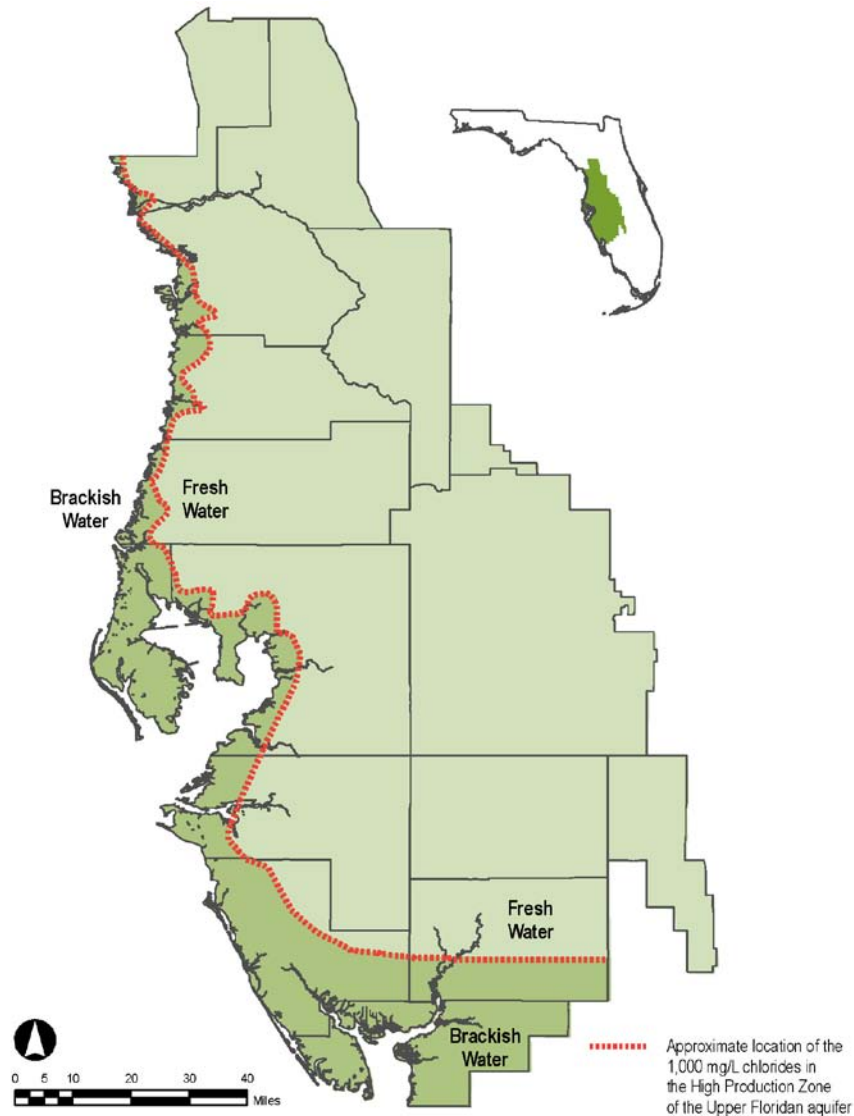
Figure 4-2 Generalized Location of the Freshwater/Saltwater Interface in the District.
