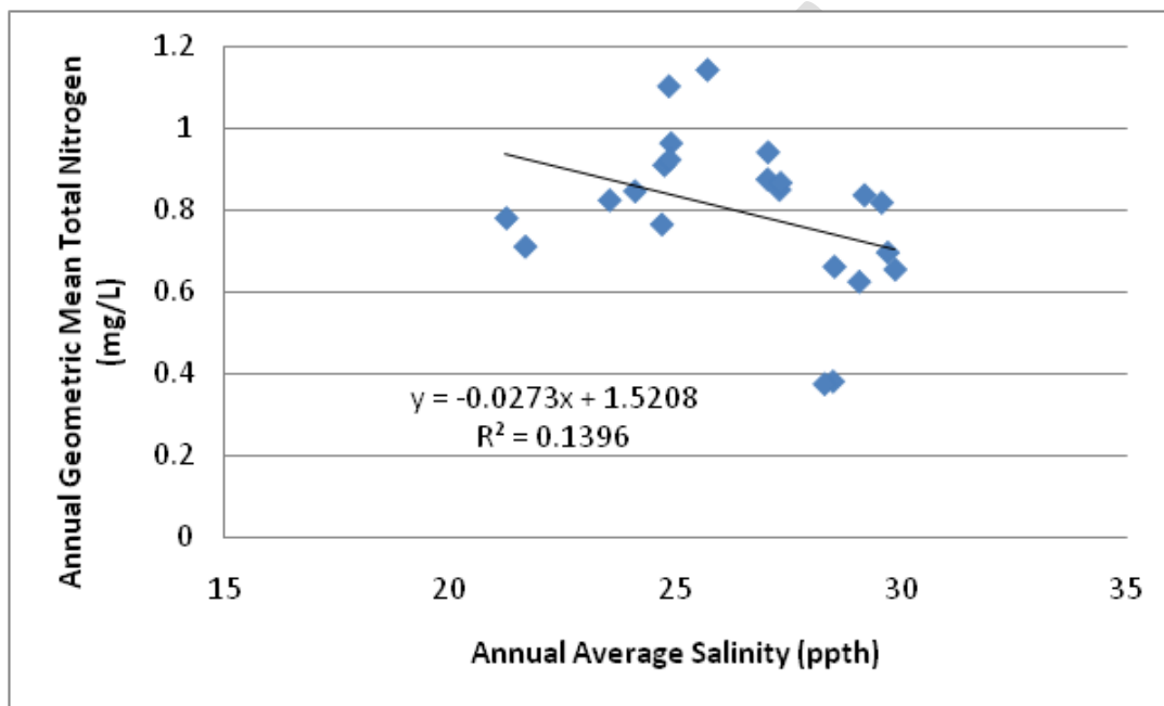
Figure 62. Annual average salinity versus annual geometric mean total nitrogen for sites CKF020C1 and CKF030C1 at Cedar Keys collected by the SRWMD from 1996-2006 (n = 22 site-years).
