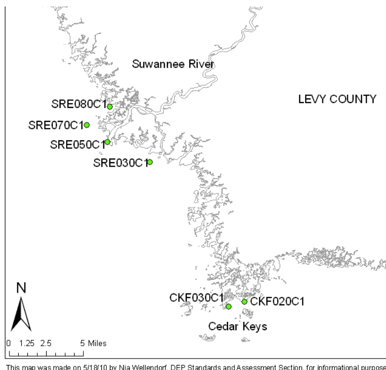
Figure 57. Location of SRWMD sampling sites in the Suwannee River Estuary (SRE) and Cedar Keys (CKF).
