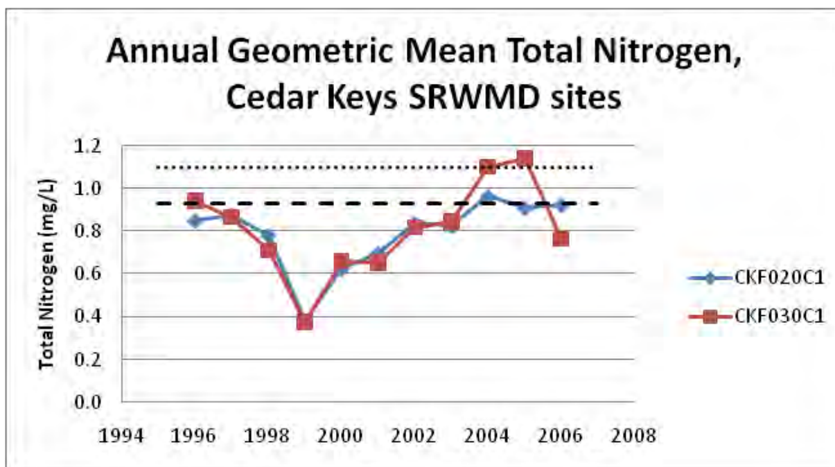
Figure 63. Annual geometric mean Total Nitrogen for Cedar Keys SRWMD sites, 1996-2006. The dashed and dotted lines indicates the 75 th and 90 th percentile of all annual geometric means, respectively (from both sites, n=22 annual geometric means, calculated with lognormal distribution function).
