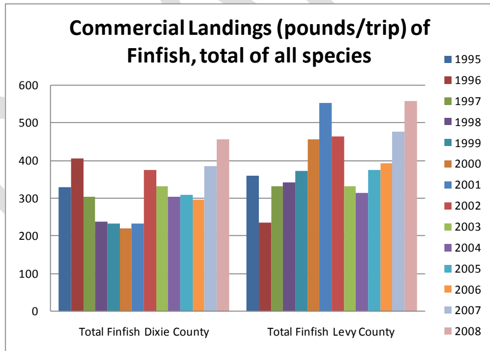
Figure 27. Total commercial finfish catch (pounds/trip) for Dixie and Levy Counties from 1995-2008. Data from the Florida Fish and Wildlife Conservation Commission.
