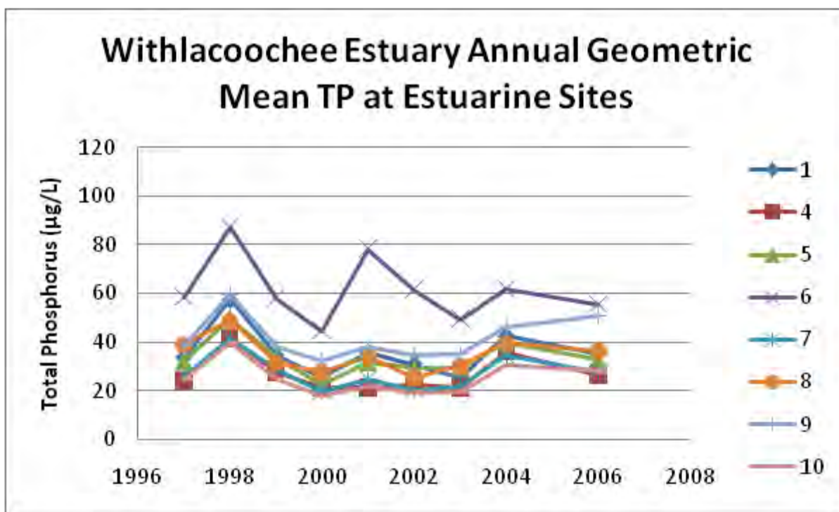
Figure 42. Mean TP at Project COAST Withlacoochee estuarine sites.
