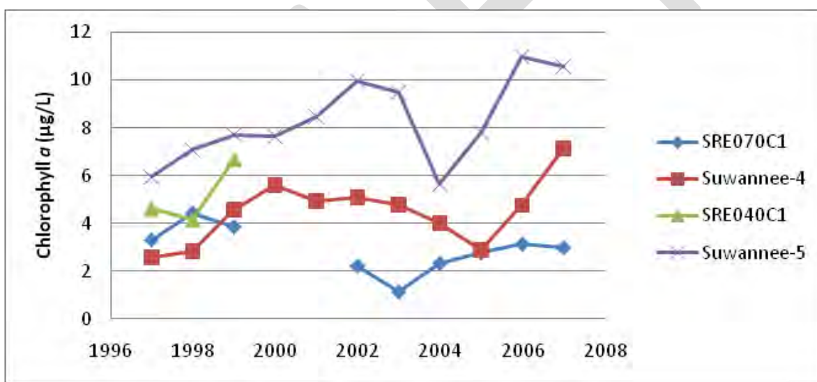
Figure 76. Comparison of annual geometric mean chlorophyll a (uncorrected) at 2 pairs of sites in the Suwannee Estuary in which the members of each pair are located fairly close to one another. Site pairs as in Figure 73.
