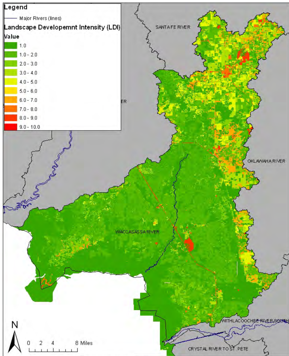
Figure 6. Landscape Development Intensity coefficients of land uses within the Waccasassa watershed, based on 2005-2008 aerial photos. LDI coefficients as in Table 3.
