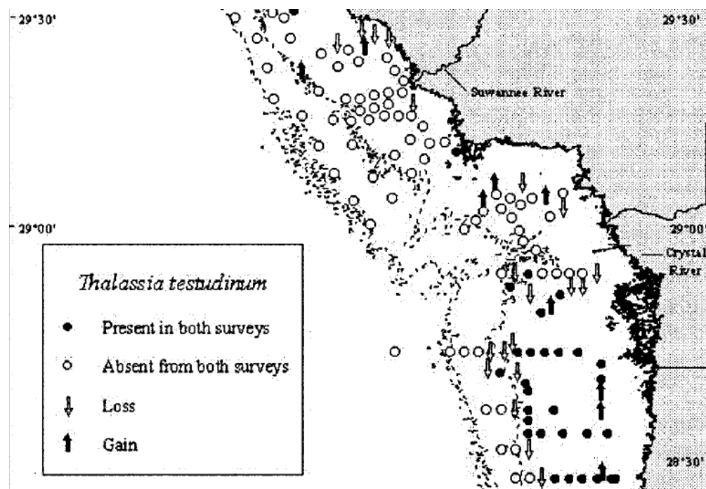
Figure 12. Distribution map for Thalassia testudinum , showing comparison of 1984 and 2000 surveys (from Hale et al. 2004).
