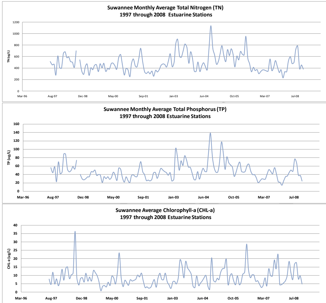
Figure 33. Long term average data for the Suwannee Estuary, including all estuary sites (excludes freshwater sites) (from Frazer and Jacoby 2010).
