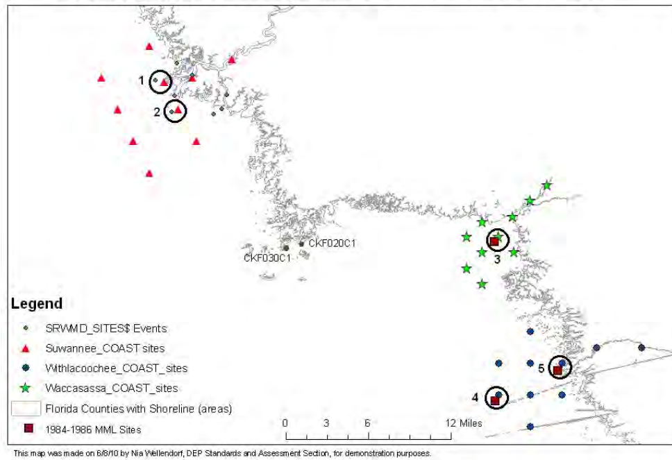
Figure 73. All study sites for which FDEP analyzed data within this report. Circled areas indicate pairs of sites sufficiently close enough in space for data comparison. 1 – COAST Suwannee-4 = SRWMD SRE070C1; 2 – COAST Suwannee-5 = SRWMD SRE040C1; 3 – MML WACC-10 = COAST Waccasassa-8; 4 – MML WITH-10 = COAST Withlacoochee-7; 5 - MML WITH-7 = COAST Withlacoochee-6.
