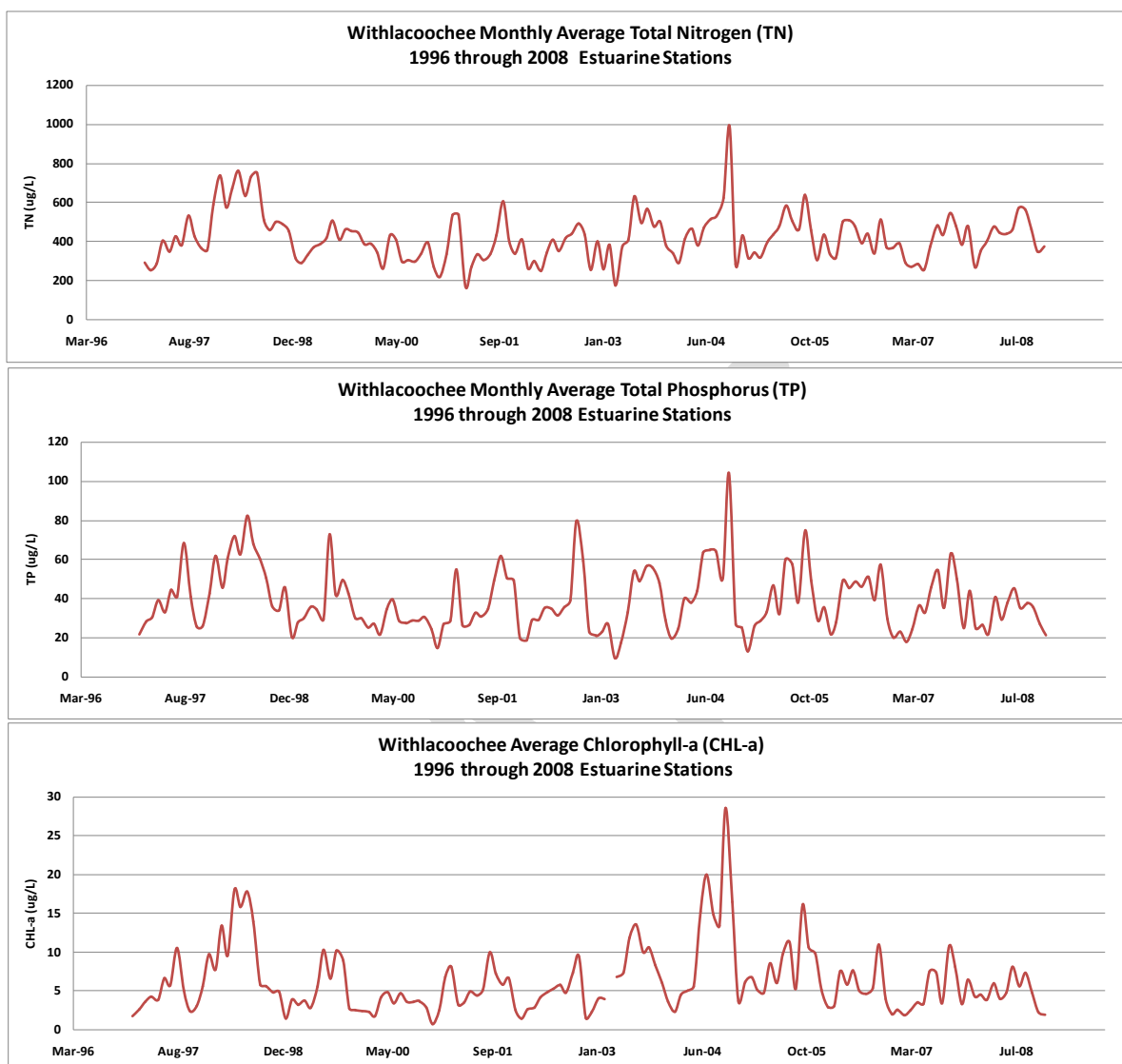
Figure 35. Long term average data for the Withlacoochee Estuary, including all estuary sites (excludes freshwater sites). From Frazer and Jacoby (2010).
