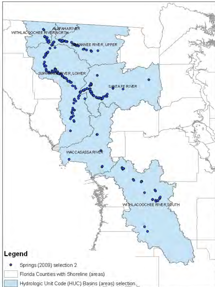
Figure 1. Study area of the Suwannee, Waccasassa, and Withlacoochee (South) watersheds. This region has numerous karst features, and here the springs are noted as blue points.
