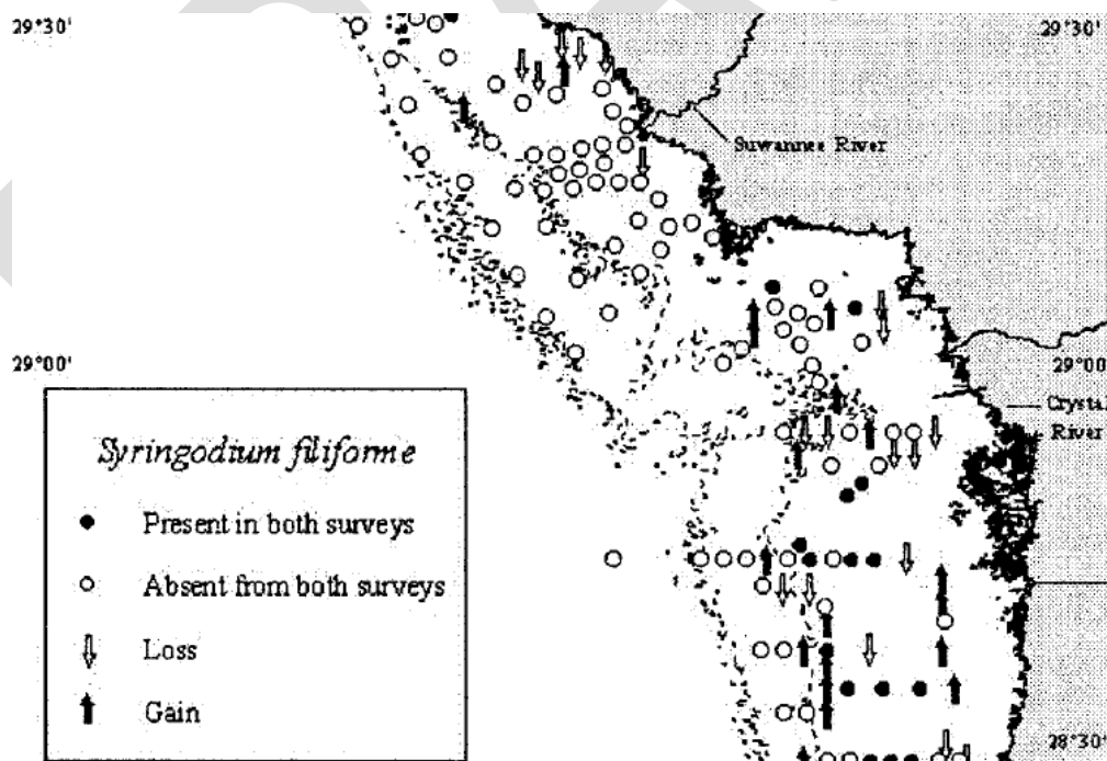
Figure 13. Distribution map for Syringodium filiforme , showing comparison of 1984 and 2000 surveys (from Hale et al. 2004).
