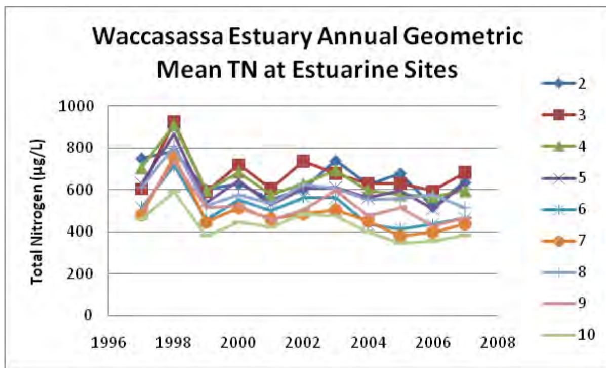
Figure 38. Mean TN at Project COAST Waccasassa estuarine sites.
