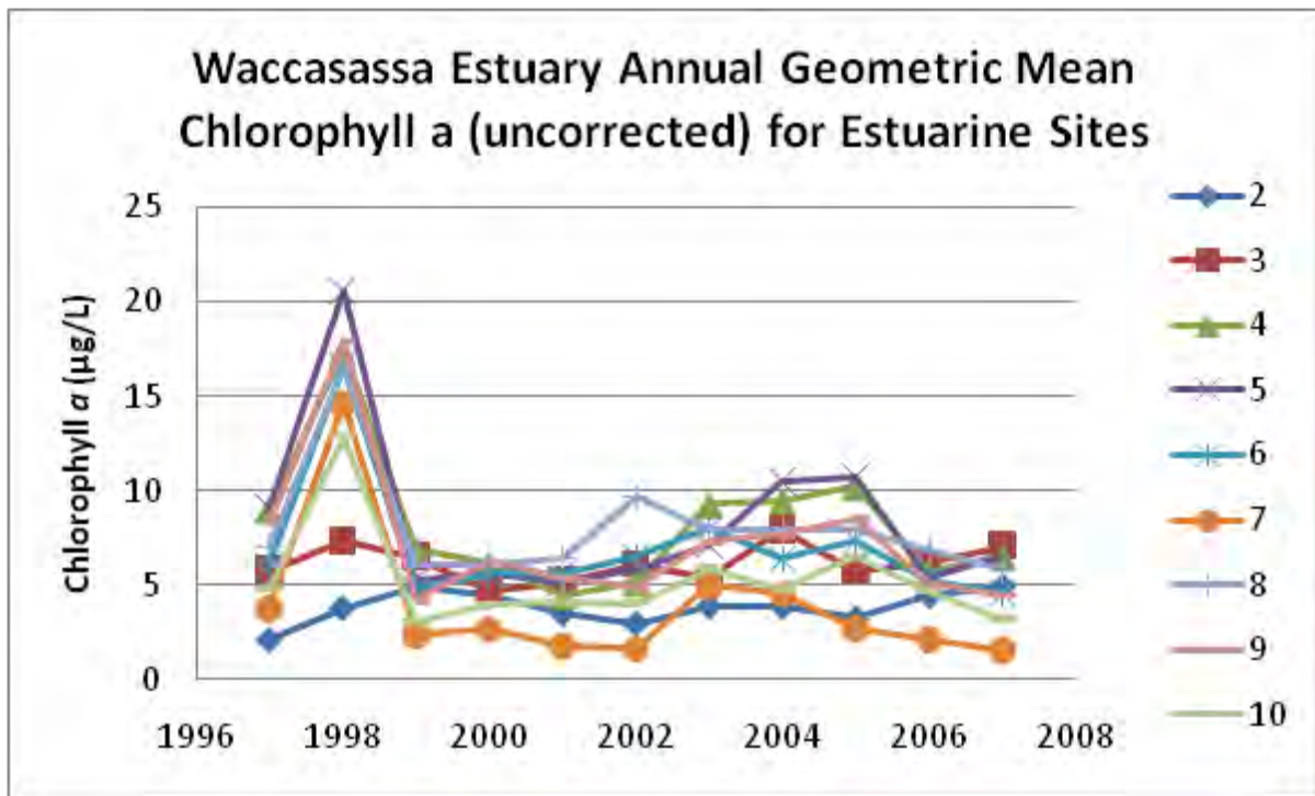
Figure 44. Mean chlorophyll a at Project COAST Waccasassa estuarine sites.
