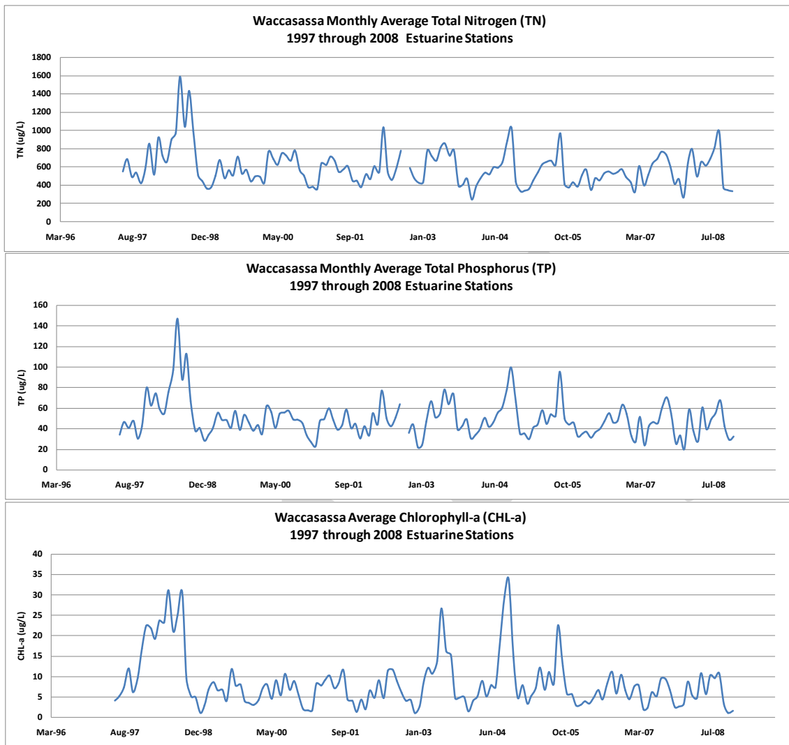
Figure 34. Long term average data for the Waccasassa Estuary, including all estuary sites (excludes freshwater sites). From Frazer and Jacoby (2010).
