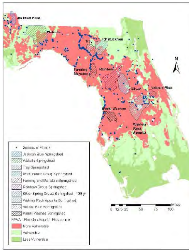
Figure 10. Aquifer vulnerability in spring areas, Figure 16 from Harrington et al. (2010).
