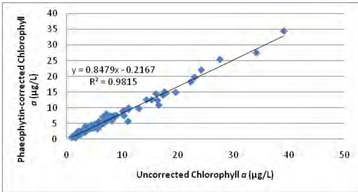
Figure 52. Comparison of uncorrected and phaeophytin-corrected chlorophyll a (µg/L) for 10 sites in the Suwannee Estuary for the first nine months of 2007.
