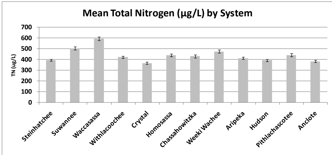
Figure 30. Mean total nitrogen (µg/L) across all sample years (approx. 1997-2009) and all estuary sites (excludes freshwater sites). From Frazer and Jacoby (2010).
