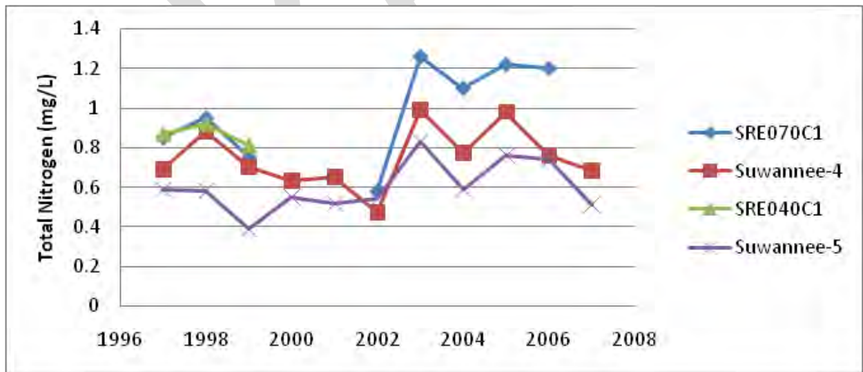
Figure 74. Comparison of annual geometric mean total nitrogen at 2 pairs of sites in the Suwannee Estuary in which the members of each pair are located fairly close to one another. Site pairs as in Figure 73.
