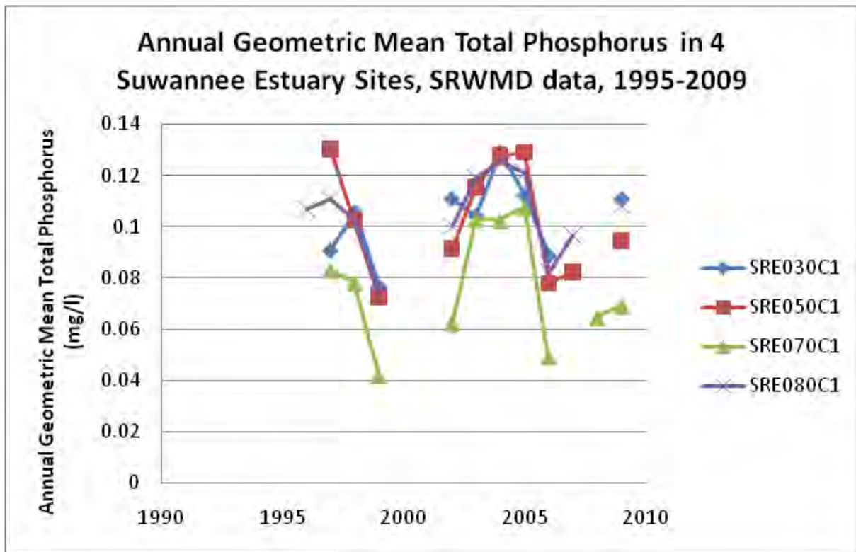
Figure 60. Annual geometric means for TP at four Suwannee Estuary sites.
