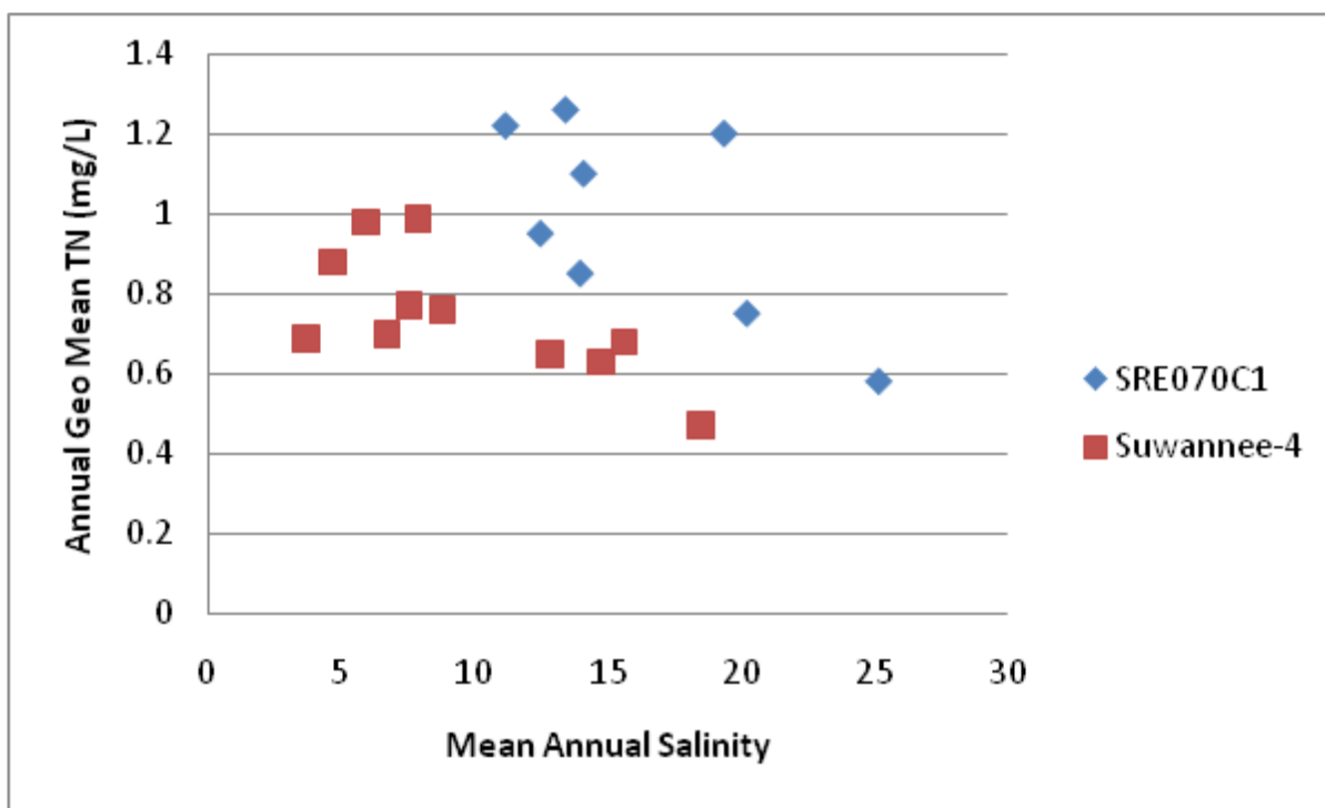
Figure 77. The relationship between mean annual salinity and annual geometric mean total nitrogen for two sites located fairly close together in the Suwannee Estuary (sites shown in Figure 73).
