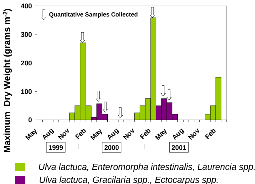
Figure 21. Observed macroalgal succession on a subset of oyster reef at the mouth of the Suwannee River, 1999-2001 (from Quinlan 2010).
