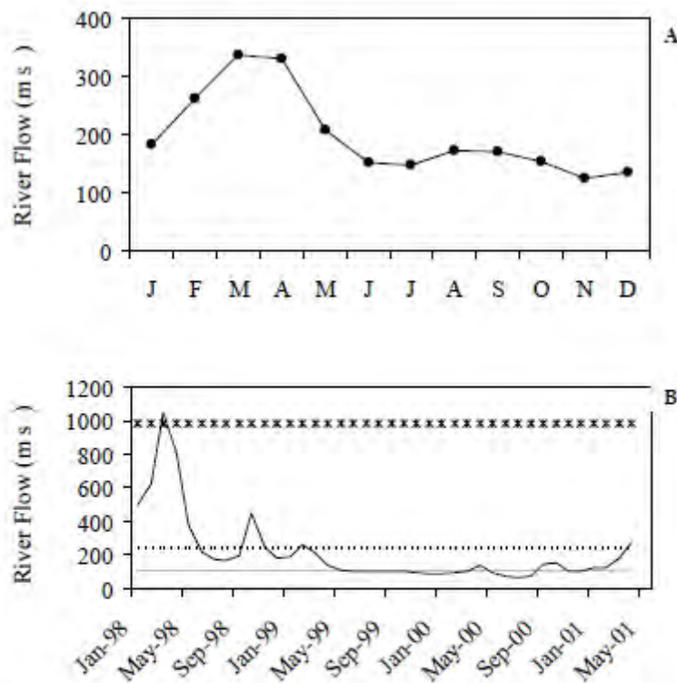
Figure 54. Flow rates in the Suwannee River at the Wilcox gauging station. (A) Long-term mean monthly flow rates from 1932 to 1999. (B) Mean monthly flow rates from 1998-2001. The dashed line (---) indicated median flow rate for the Suwannee River. The gray line represents the flow rate exceeded 99% of the time from 1960-2001, and the asterisk (***) line represents the flow rate exceeded only 1% of all dates from 1960-2001. Figure from Quinlan (2003).
