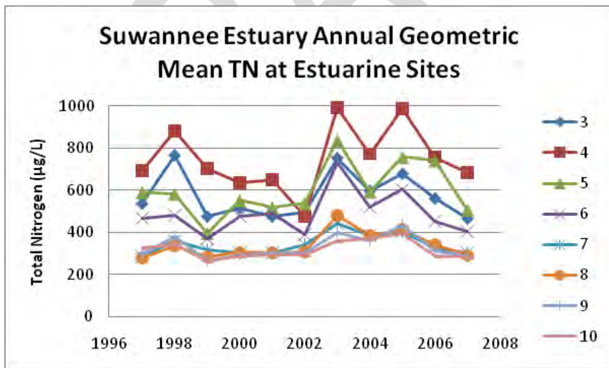
Figure 37. Mean TN at Project COAST Suwannee estuarine sites.
