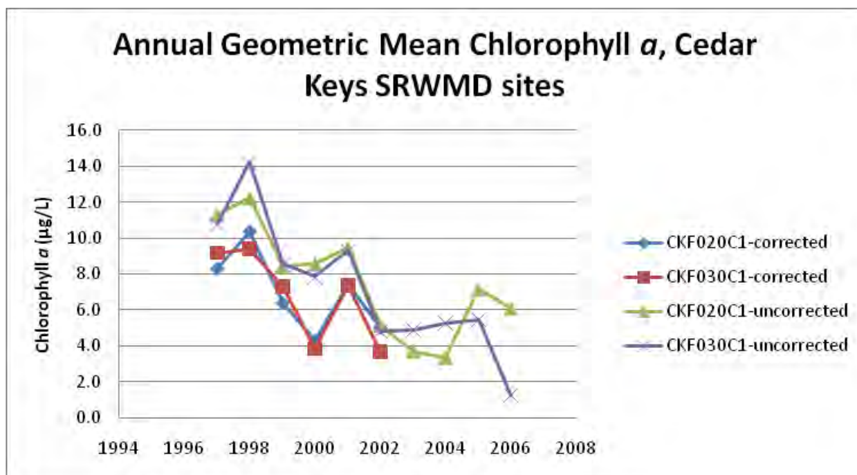
Figure 65. Annual geometric mean corrected and uncorrected chlorophyll a for Cedar Keys SRWMD sites, 1996-2006.
