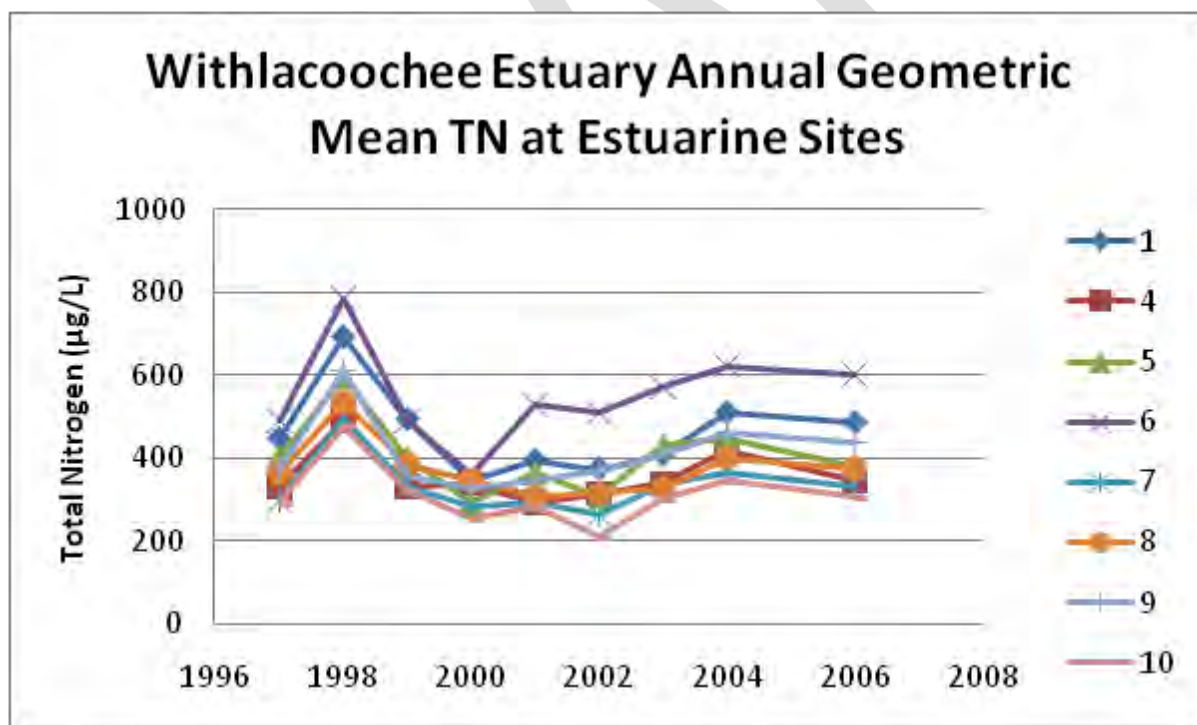
Figure 39. Mean TN at Project COAST Withlacoochee estuarine sites.
