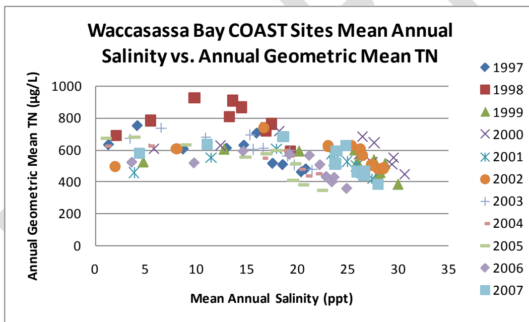
Figure 50. Salinity vs. TN in Waccasassa Bay.
