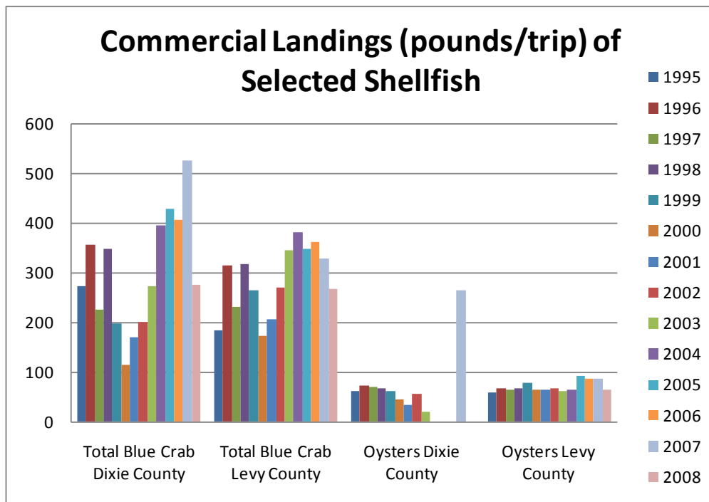
Figure 25. Total commercial blue crab and oyster catch (pounds/trip) for Dixie and Levy Counties from 1995-2008. Data from the Florida Fish and Wildlife Conservation Commission.
