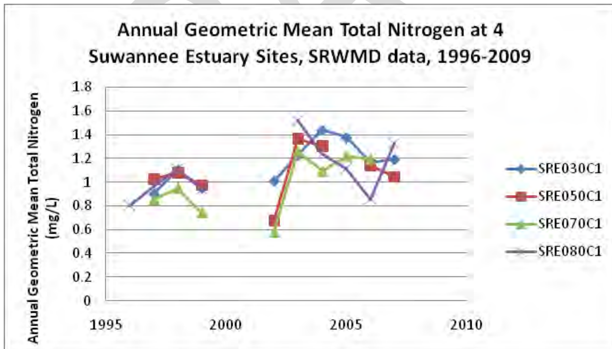
Figure 59. Annual geometric means for TN at four Suwannee Estuary sites.
