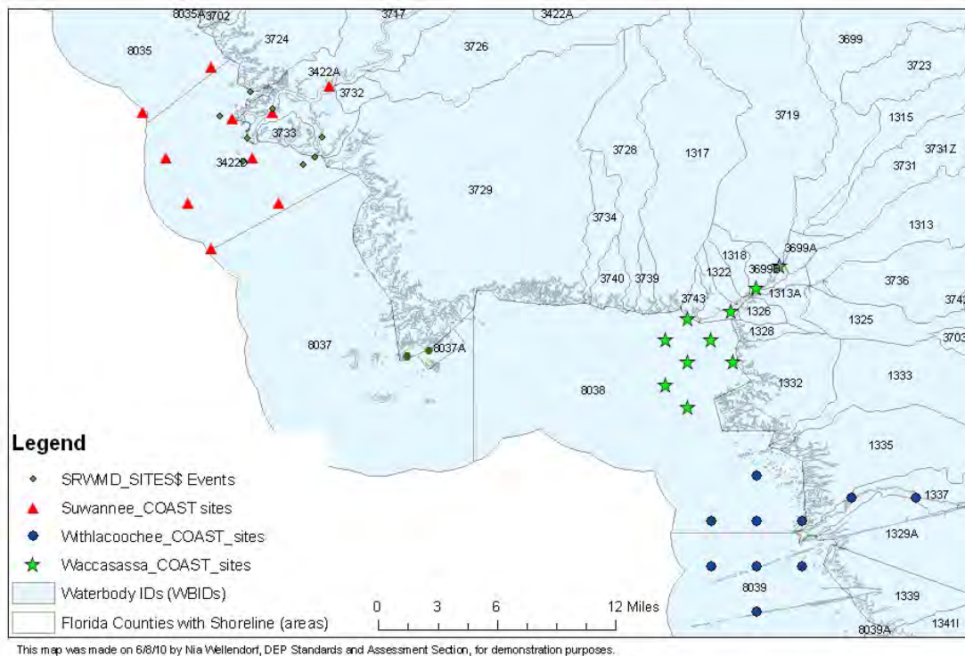
Figure 78. WBIDs in the Suwannee, Waccasassa, and Withlacoochee Estuary regions, and sampling stations from Project COAST and the SRWMD.
