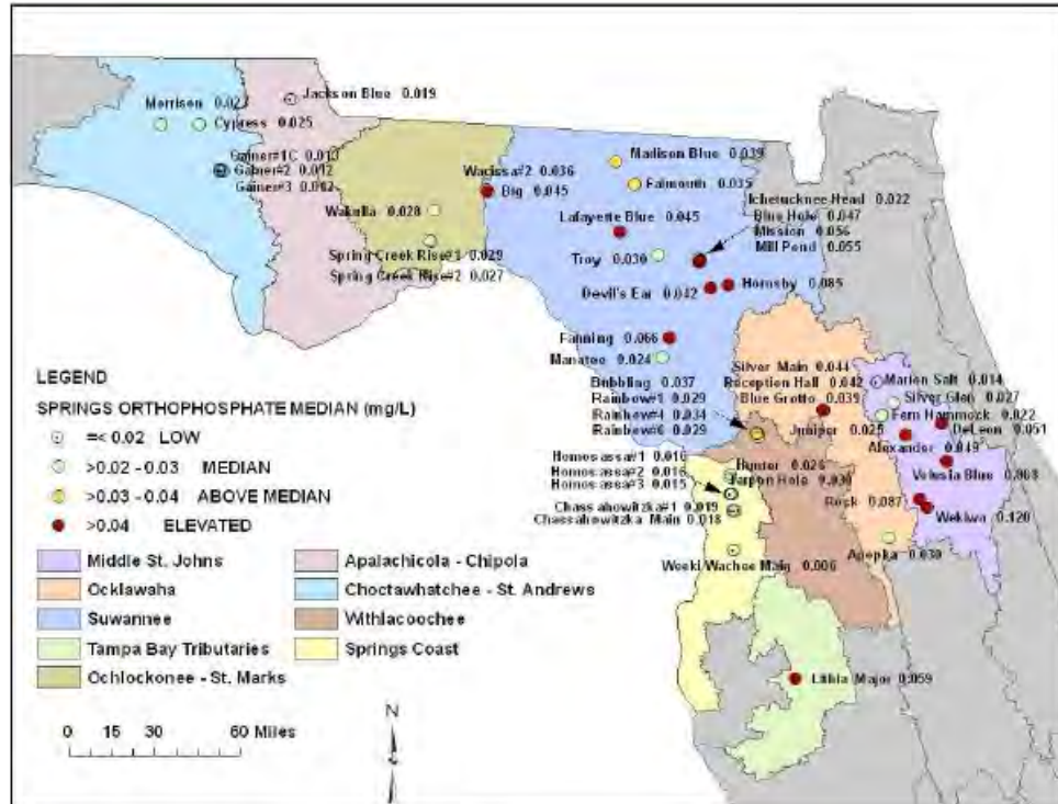
Figure 9. Median orthophosphate concentrations in the Spring Network (2001-2006) from Harrington et al. (2010).
