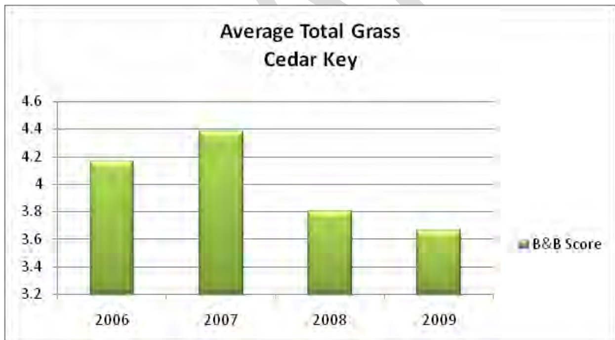
Figure 17. Average total grass coverage, Cedar Keys, 2006-2009. AVG B&B represents the average Braun-Blanquet ranking assigned at each of 100 sampling quadrats per year. Ranks are abundance codes ranging from 1-5.
