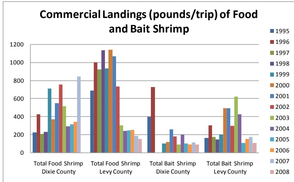
Figure 26. Total commercial shrimp catch (pounds/trip) for Dixie and Levy Counties from 1995-2008. Data from the Florida Fish and Wildlife Conservation Commission.
