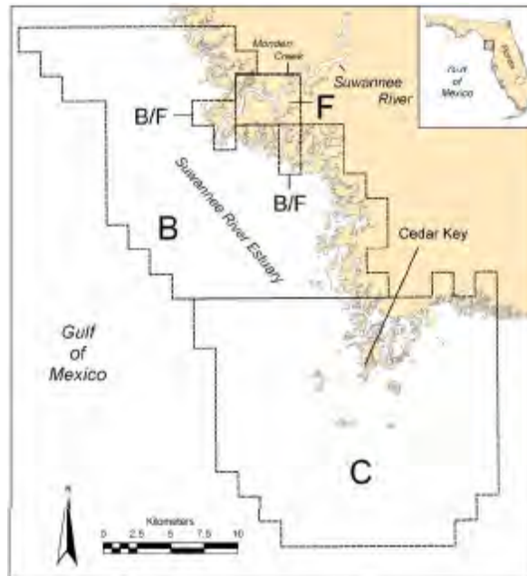
Figure 24. Map of Cedar Key sampling area of the Fisheries Independent Monitoring Program. Zones are labeled B, C, and F. Grids containing portions of Zones B and F are labeled B/F.
