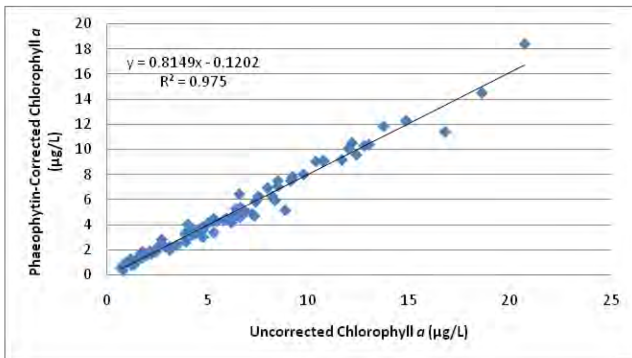
Figure 51. Comparison of uncorrected and phaeophytin-corrected chlorophyll a (µg/L) for 10 sites in the Waccasassa Estuary for the first nine months of 2007.
