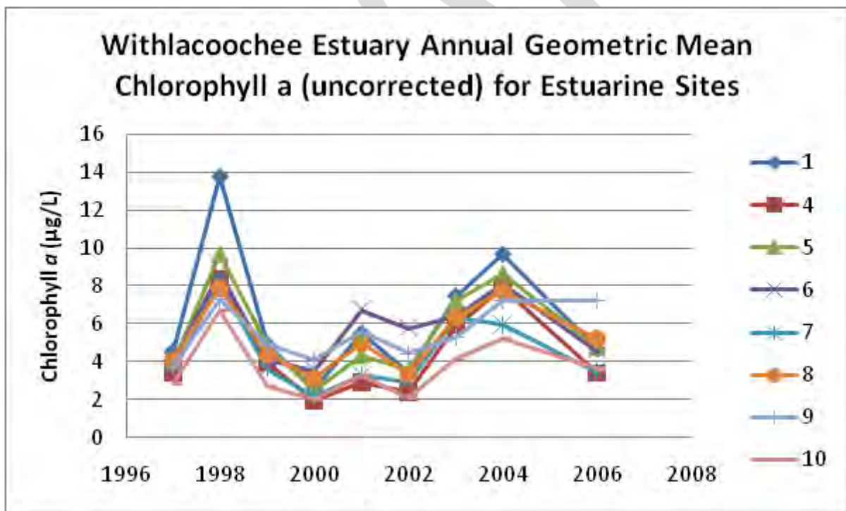
Figure 45. Mean chlorophyll a at Project COAST Withlacoochee estuarine sites.
