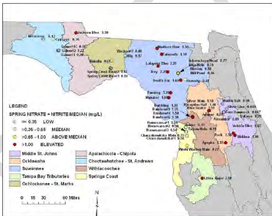
Figure 8. Median concentrations of nitrate+nitrite in the Spring Network, 2001–06 ( from Harrington et al. 2010).
