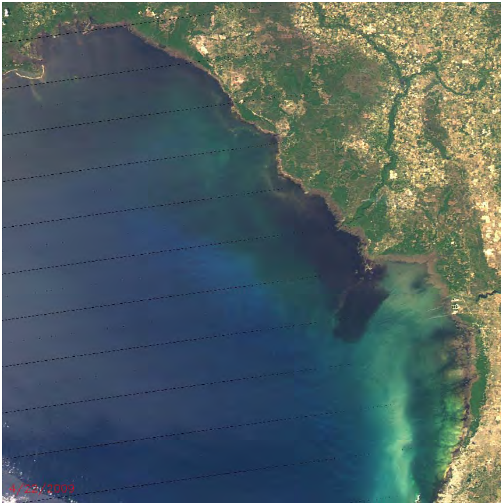
Figure 5. MODIS satellite imagery from 4/22/2009 of the Big Bend and Springs Coast, showing abundance of colored dissolved organic matter (CDOM) from the Suwannee River surrounding Cedar Keys to the south and extending north to Horseshoe Beach.
