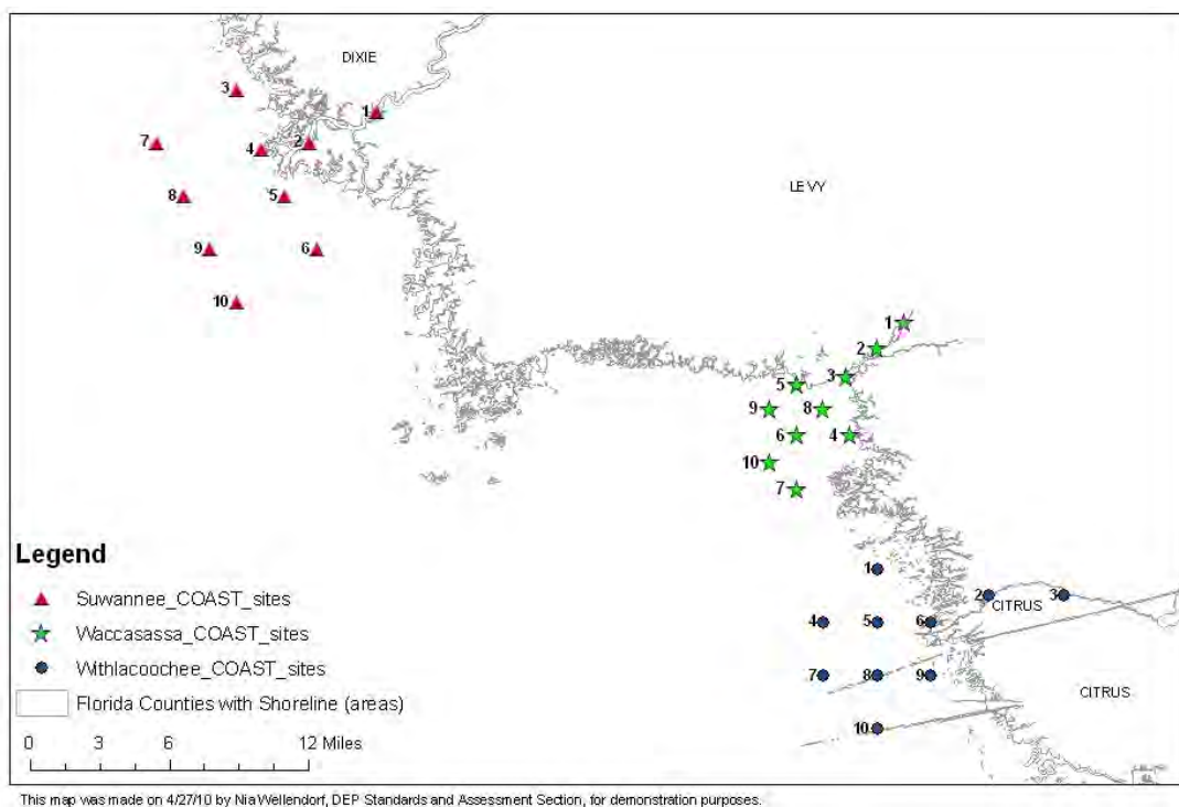
Figure 36. Project COAST sampling sites in the Suwannee, Waccasassa, and Withlacoochee estuaries.
