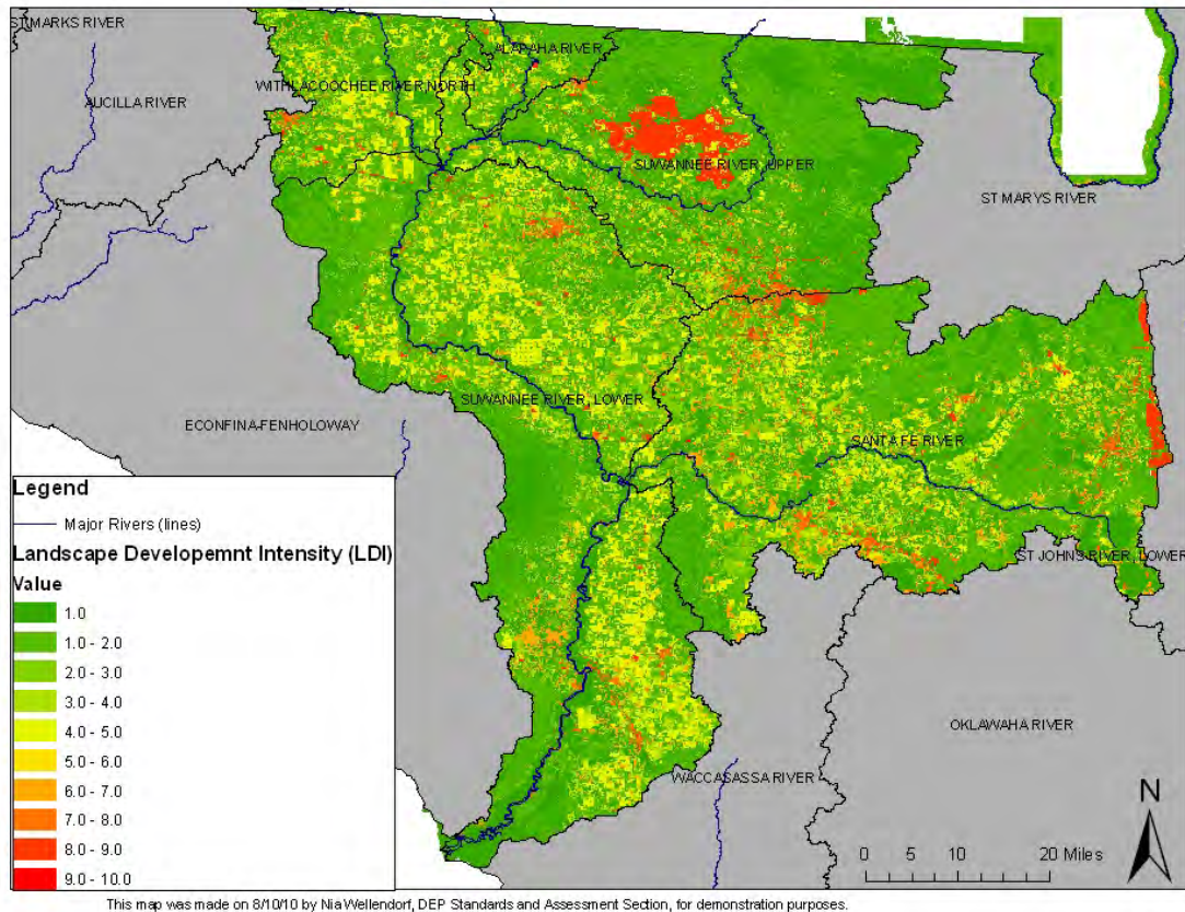
Figure 2. Landscape Development Intensity coefficients of land uses within the Florida portion of the Suwannee Watershed, based on 2005-2008 aerial photos. LDI coefficients as in Table 3.
