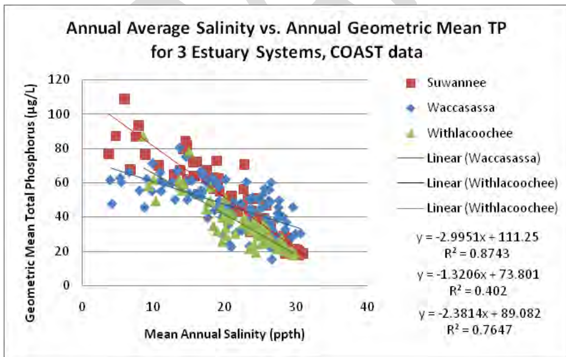
Figure 47. Stations 1 and 2 excluded for Suwannee, Station 1 excluded for Waccasassa, and Stations 2 and 3 excluded for Withlacoochee. R^2 = 0.87 for Suwannee, R^2 = 0.40 for Waccasassa, R^2 = 0.76 for Withlacoochee.
