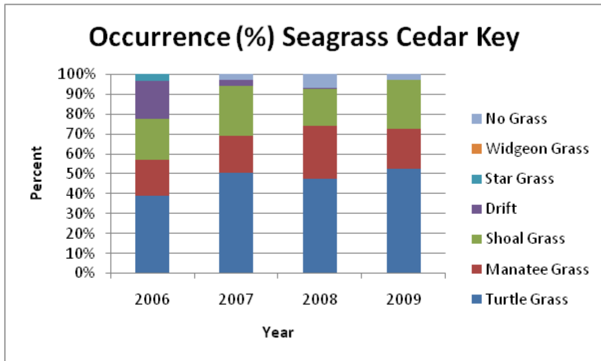
Figure 16. Frequency of occurrence of seagrass species at Cedar Keys, 2006-2009.
