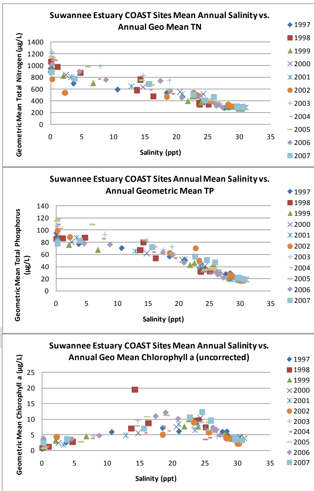
Figure 48. Average annual salinity for each site plotted against the annual geometric means for total nitrogen, total phosphorus, and chlorophyll a for each site sampled for Project Coast 1997-2007.
