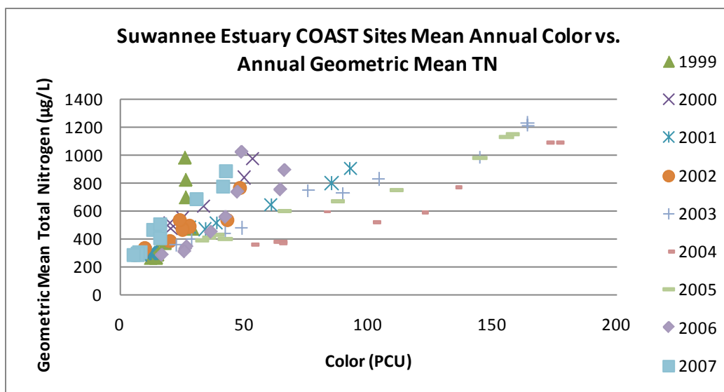
Figure 49. Color vs. TN in the Suwannee estuary.
