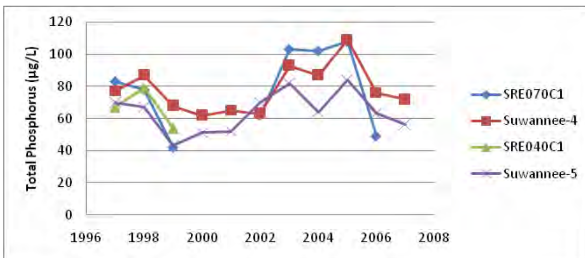
Figure 75. Comparison of annual geometric mean total phosphorus at 2 pairs of sites in the Suwannee Estuary in which the members of each pair are located fairly close to one another. Site pairs as in Figure 73.
