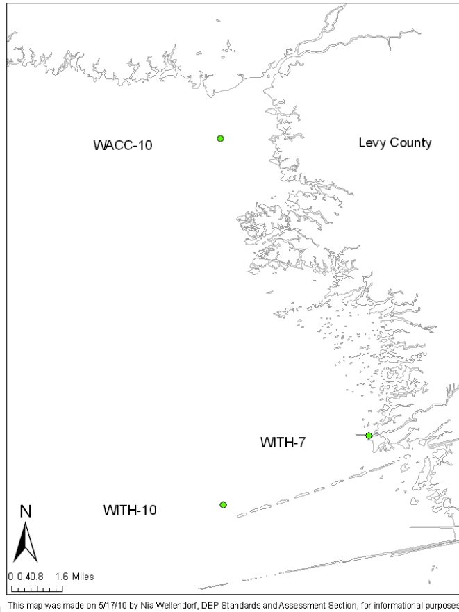
Figure 28. Locations of sampling sites for which data were analyzed from the 1984-1985 Mote Marine Lab study in the Waccasassa and Withlacoochee estuaries.
