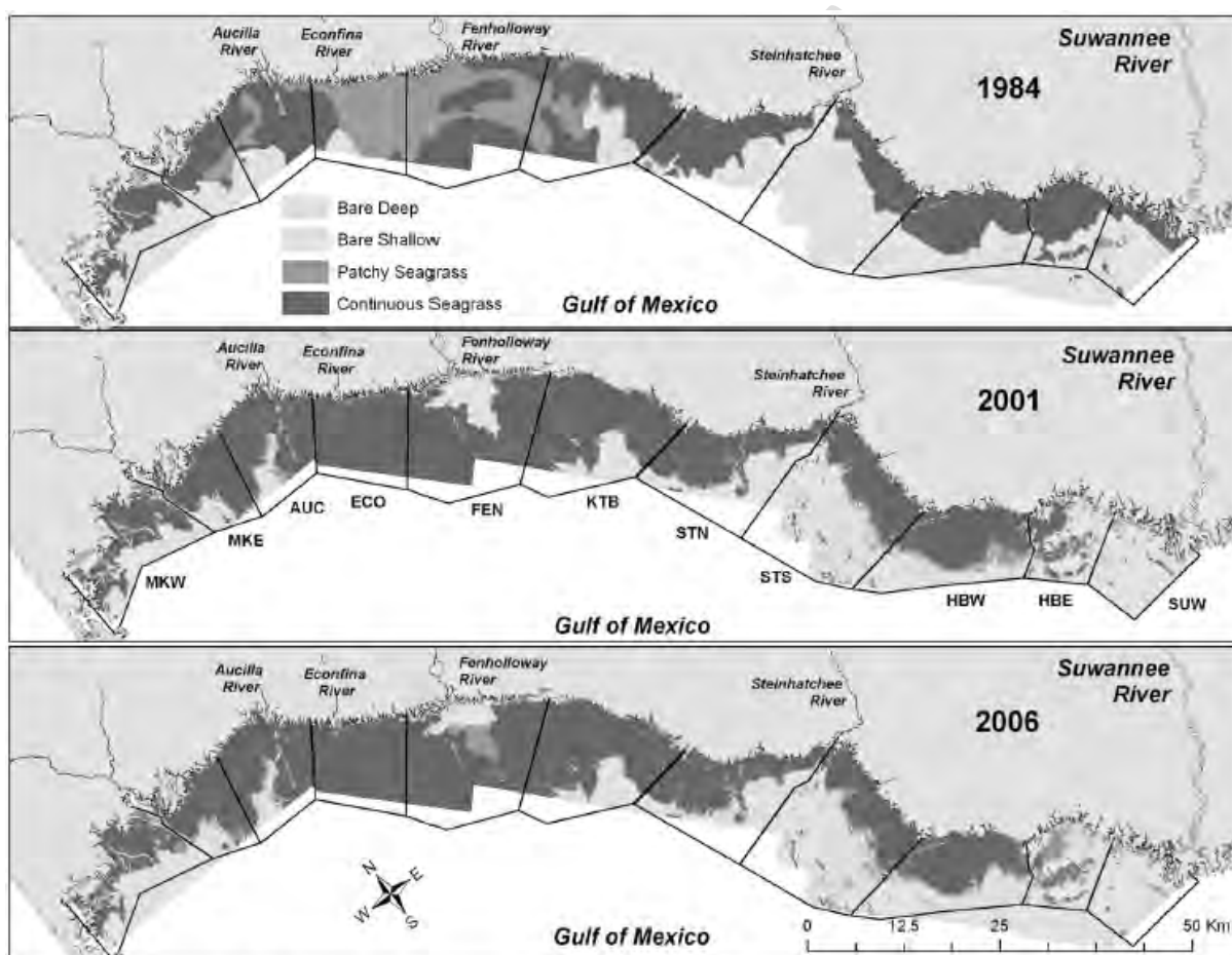
Figure 11. Big Bend seagrass cover in 1984, 2001, and 2006. Of note for this report is the apparent decline in seagrass coverage north of Suwannee Sound potentially due to effects from the Suwannee River (from Carlson et al. 2010).
