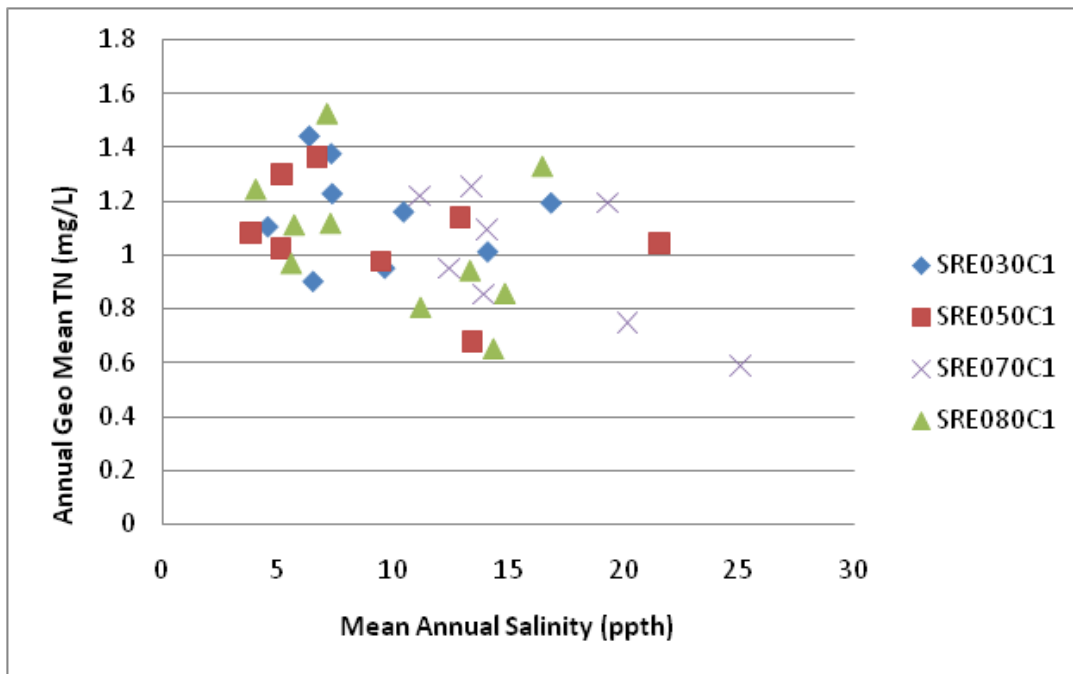
Figure 58. Annual mean salinity vs. annual geometric mean TN for 4 sites in the Suwannee Estuary, sampled by SRWMD or their contractors. Only site-years with four or more data points were used. Salinity data include "0" data points from Robbie McKinney, who indicated confidence in those data points (especially for earlier years). Data are from sites as in Figure 38.
