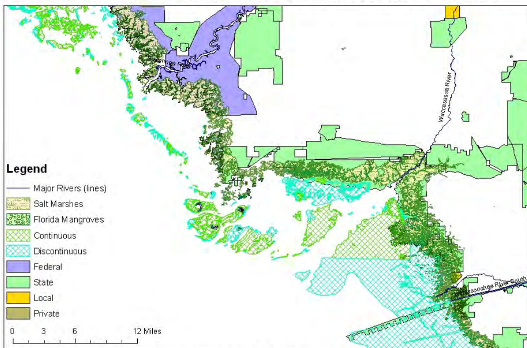
Figure 3. Coast of Dixie and Levy Counties, estuaries of the Suwannee, Waccasassa, and Withlacoochee Rivers. Shown are conservation areas (federal, state, local, and private), seagrass coverage (continuous, discontinuous), and coverage of saltwater marshes along the shores.
