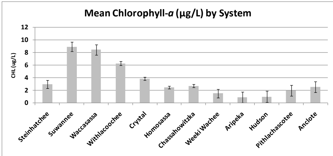
Figure 32. Mean chlorophyll a ( \mu\text{g/L} ) across all sample years (approx. 1997-2009) and all estuary sites (excludes freshwater sites). From Frazer and Jacoby (2010).
