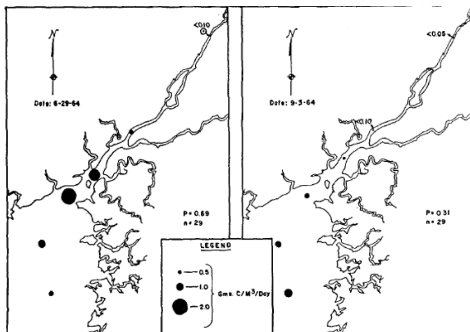
Figure 19. Variation in productivity pattern in Waccasassa Bay (from Putnam 1967). Larger circles indicate higher primary productivity.
