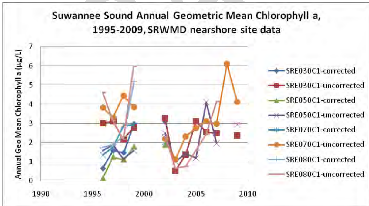
Figure 61. Annual geometric means for chlorophyll a at four Suwannee Estuary sites.
