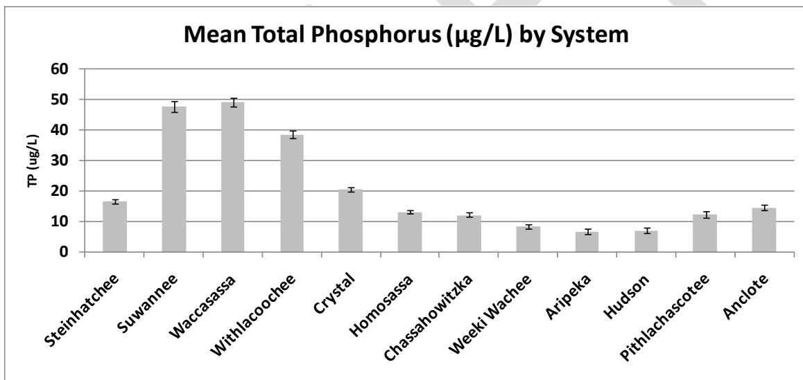
Figure 31. Mean total phosphorus (µg/L) across all sample years (approx. 1997-2009) and all estuary sites (excludes freshwater sites). From Frazer and Jacoby (2010).
