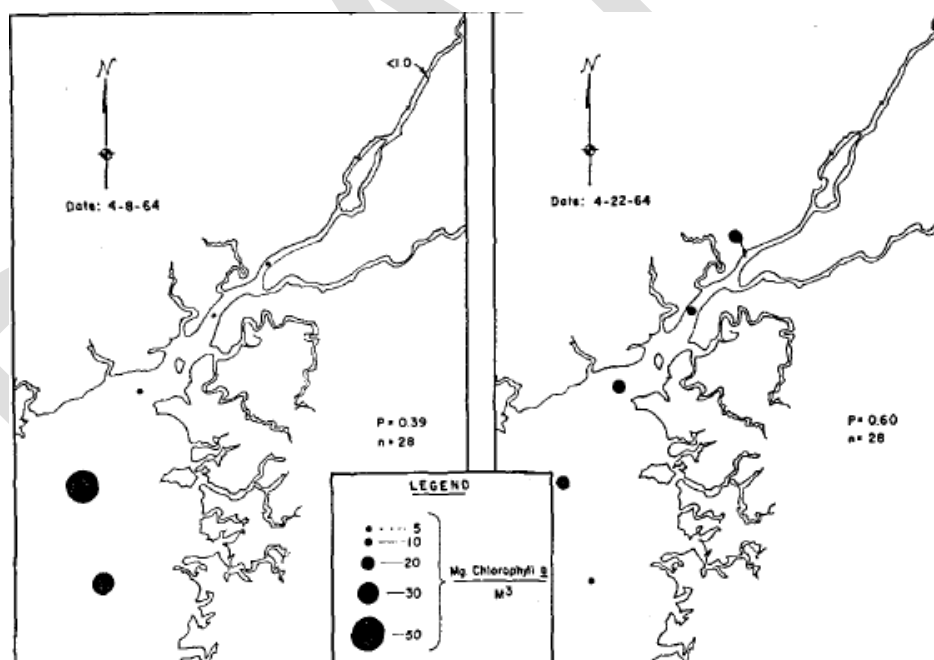
Figure 20. Variation of chlorophyll a in estuarine surface water in Waccasassa Bay (Figure 7 from Putnam 1967).
