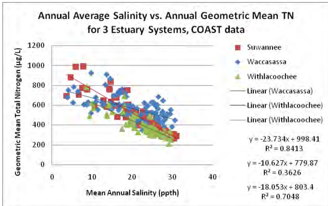
Figure 46. Stations 1 and 2 excluded for Suwannee, Station 1 excluded for Waccasassa, and Stations 2 and 3 excluded for Withlacoochee. R^2 = 0.84 for Suwannee, R^2 = 0.36 for Waccasassa, R^2 = 0.70 for Withlacoochee.
