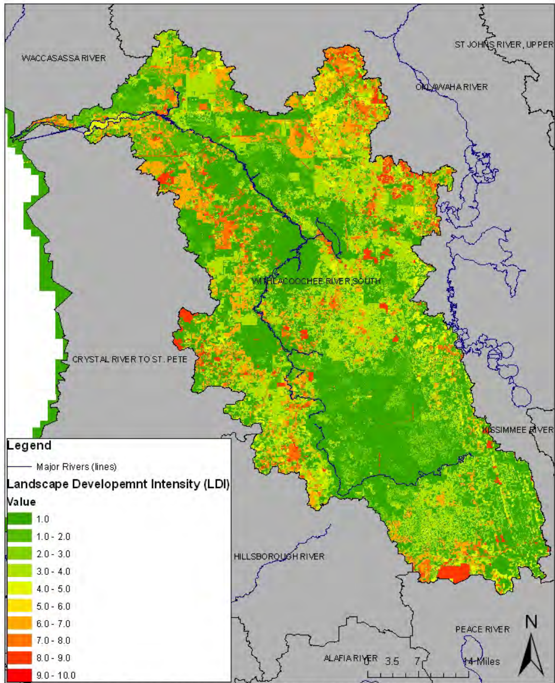
Figure 7. Landscape Development Intensity coefficients of land uses within the Withlacoochee watershed, based on 2005-2008 aerial photos. LDI coefficients as in Table 3.
