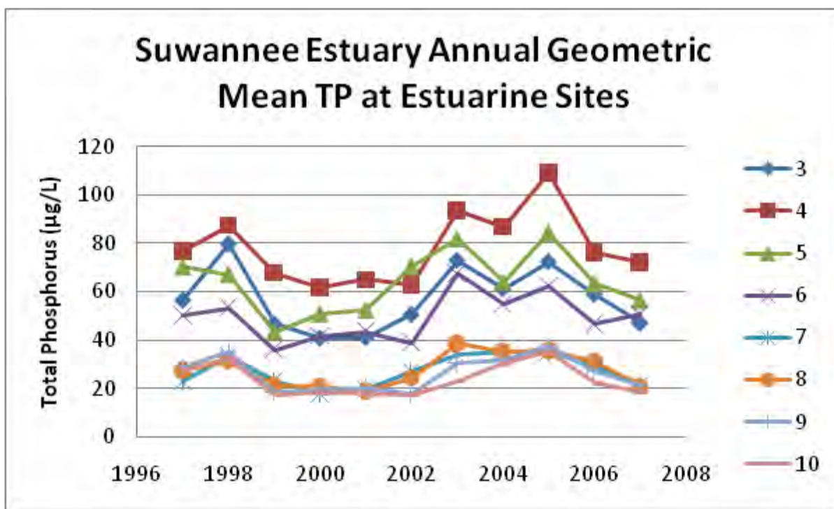
Figure 40. Mean TP at Project COAST Suwannee estuarine sites.
