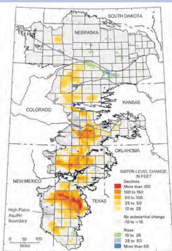
Water Level Changes in the High Plains Aquifer 1950 to 2005
