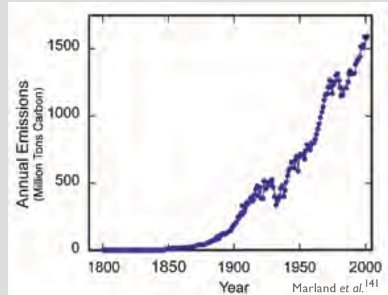
U.S. annual emissions of CO 2 from fossil-fuel use. 141
