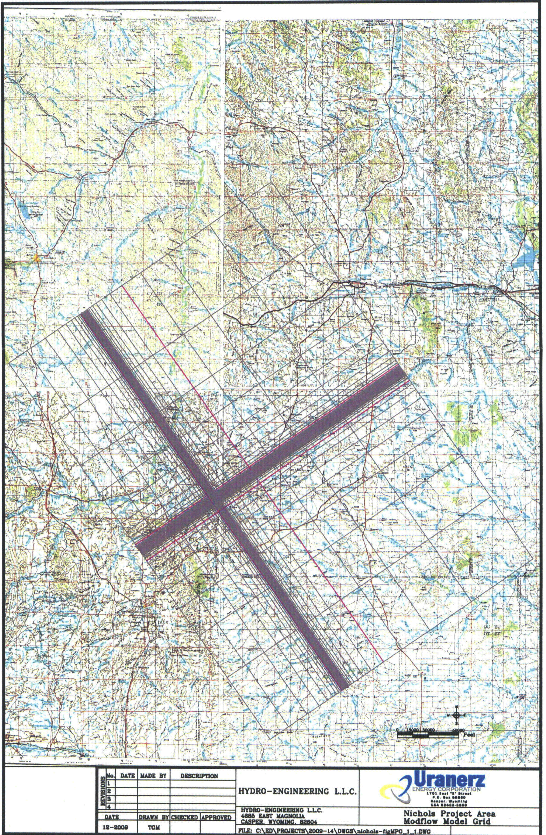
Figure MPG.1-1. Nichols Project Area Modflow Model Grid
