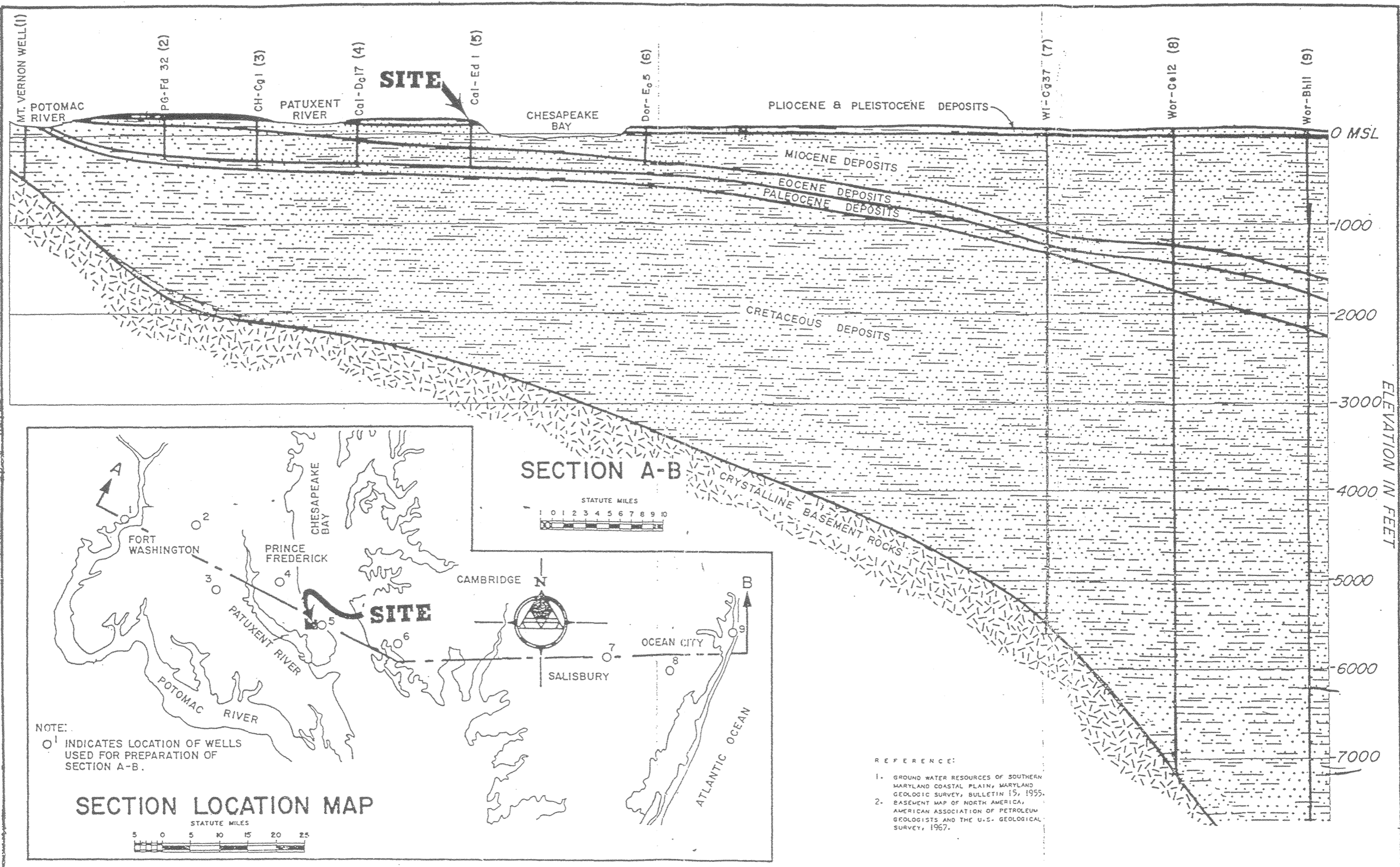
REGIONAL GEOLOGIC SECTION - COASTAL PLAIN
