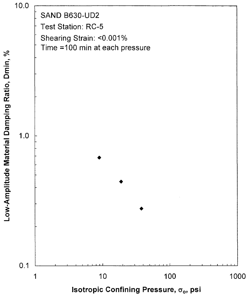
Figure B.6 Variation in Low-Amplitude Material Damping Ratio with Isotropic Confining Pressure from Resonant Column Tests
