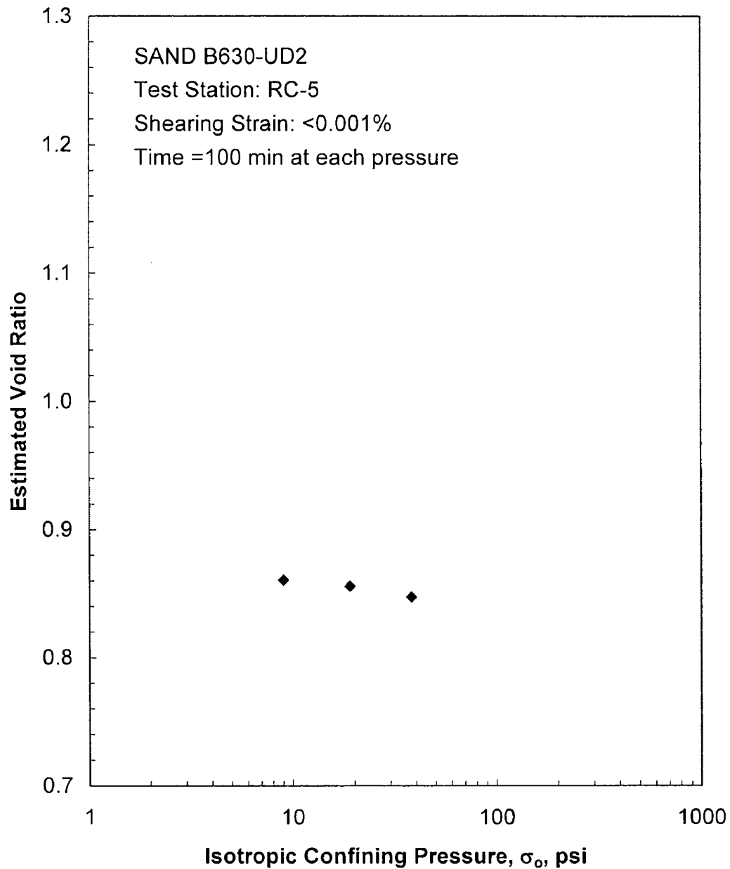
Figure B.7 Variation in Estimated Void Ratio with Isotropic Confining Pressure from Resonant Column Tests
