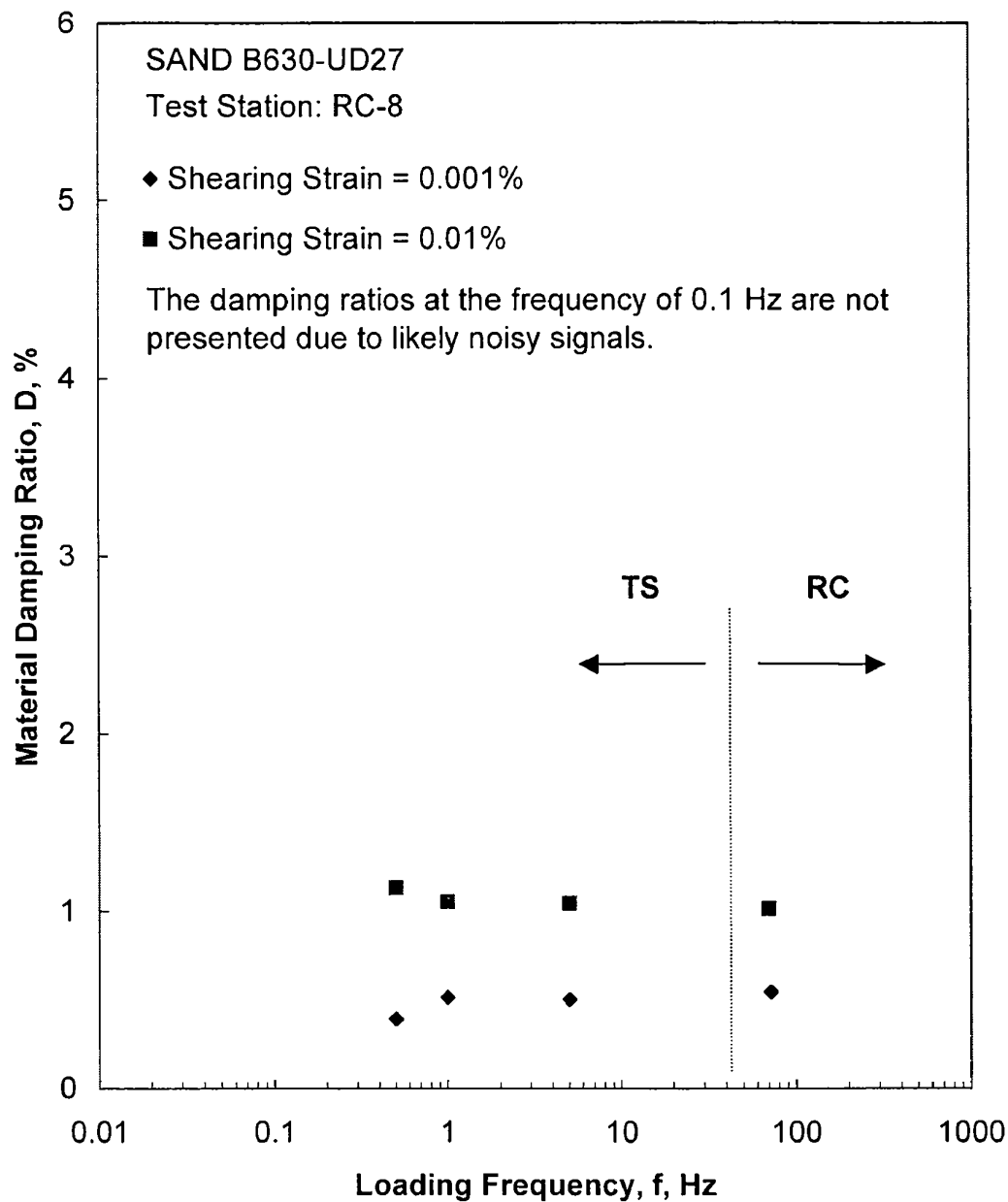
Figure G.15 Comparison of the Variation in Material Damping Ratio with Loading Frequency at an Isotropic Confining Pressure of 84 psi from the Combined RCTS Tests
