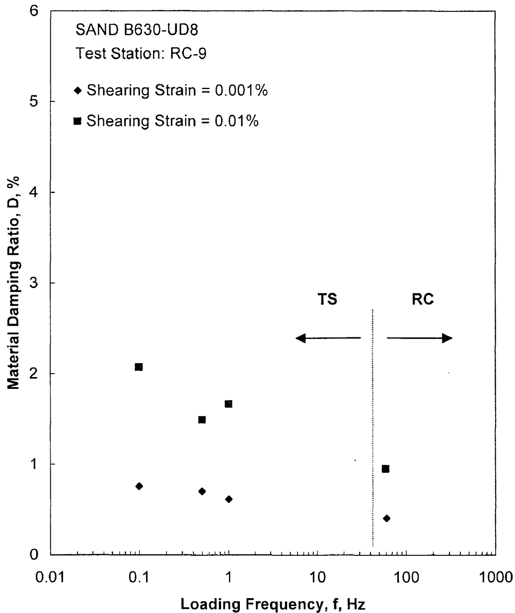
Figure A.15 Comparison of the Variation in Material Damping Ratio with Loading Frequency at an Isotropic Confining Pressure of 47 psi from the Combined RCTS Tests
