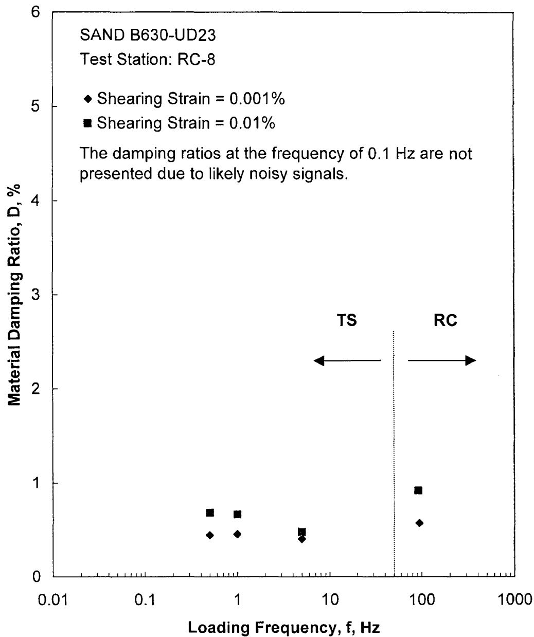
Figure F.20 Comparison of the Variation in Material Damping Ratio with Loading Frequency at an Isotropic Confining Pressure of 300 psi from the Combined RCTS Tests
