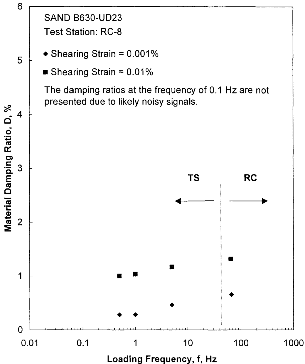
Figure F.15 Comparison of the Variation in Material Damping Ratio with Loading Frequency at an Isotropic Confining Pressure of 75 psi from the Combined RCTS Tests
