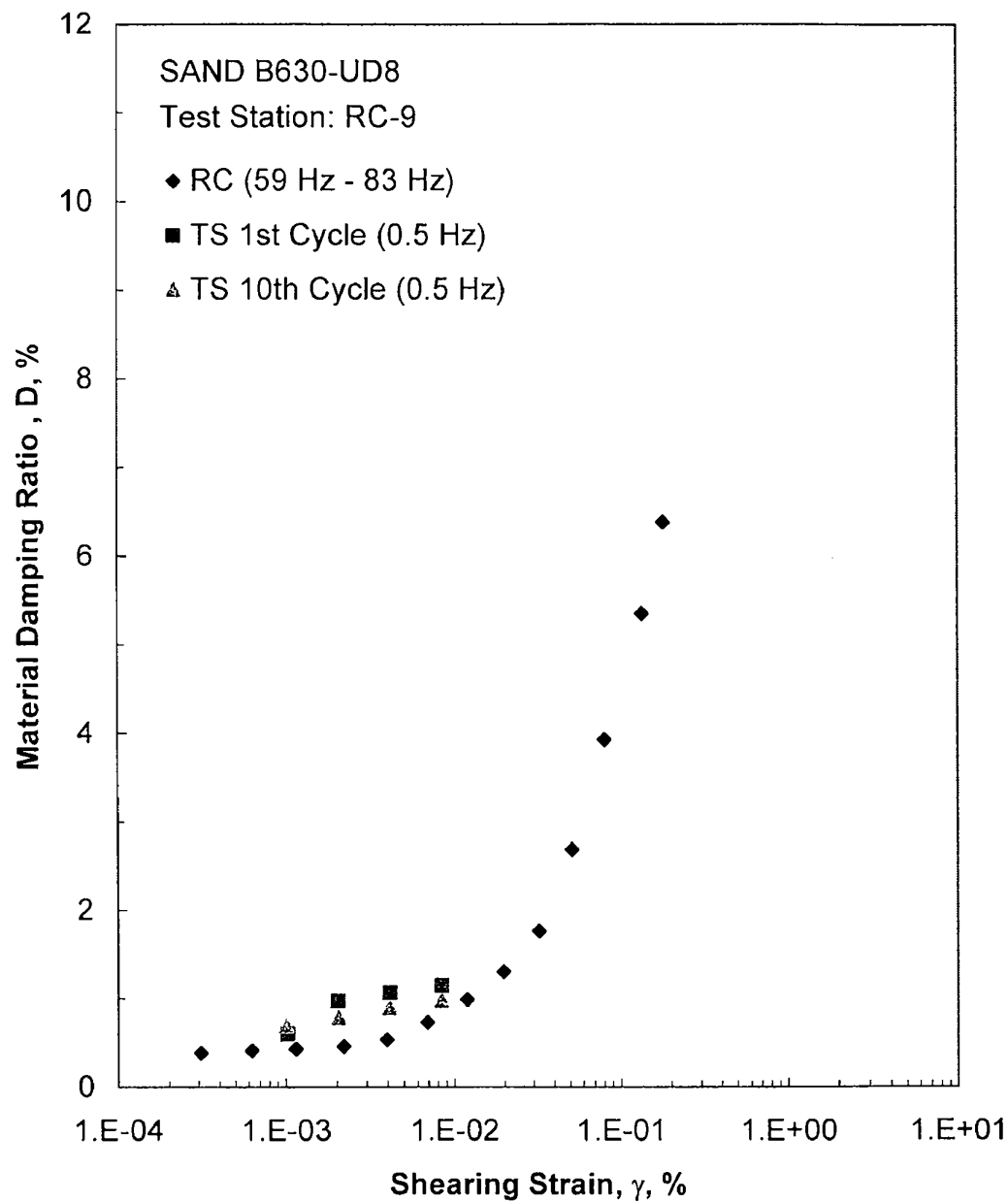
Figure A.18 Comparison of the Variation in Material Damping Ratio with Shearing Strain at an Isotropic Confining Pressure of 187 psi from the Combined RCTS Tests
