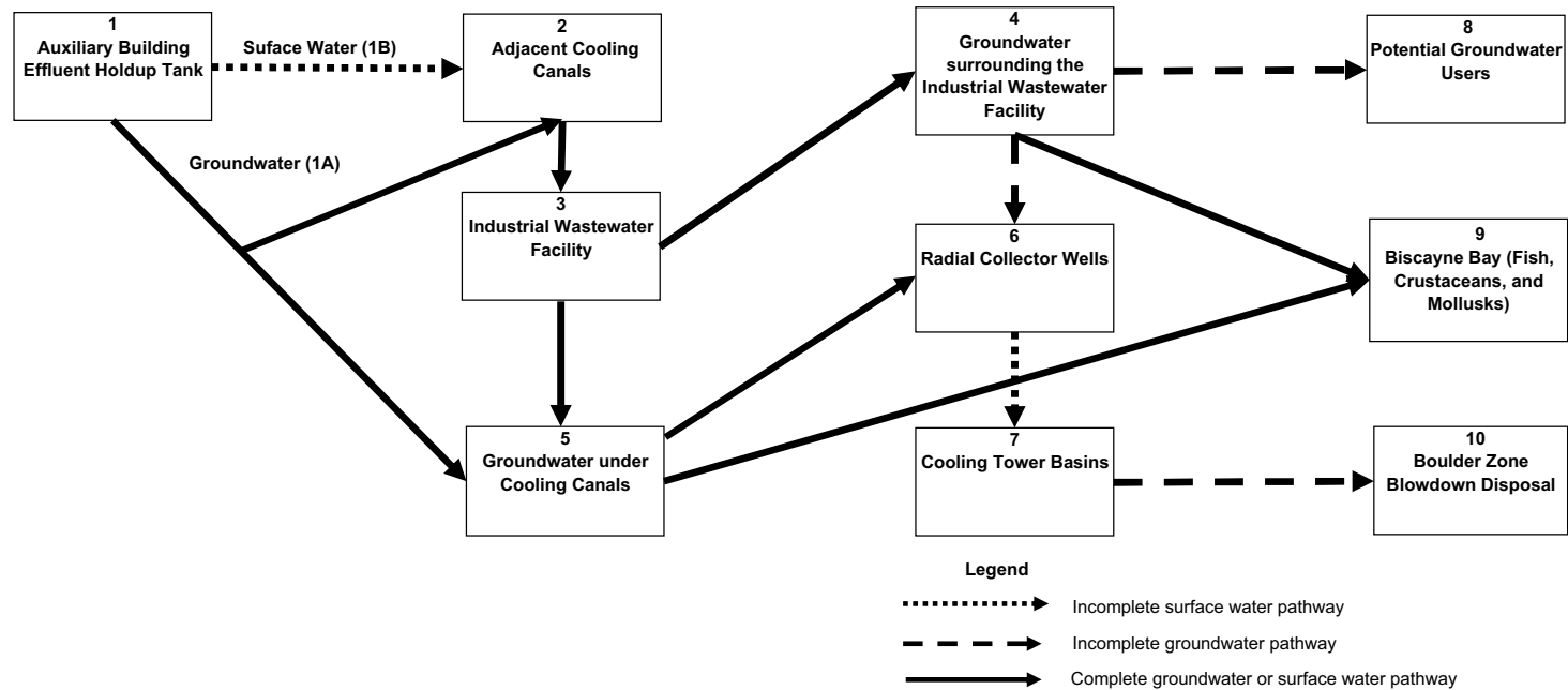
PTN COL 2.4-5 Figure 2.4.13-201 Conceptual Exposure Pathways for Evaluating Radionuclide Transport in the Biscayne Aquifer
