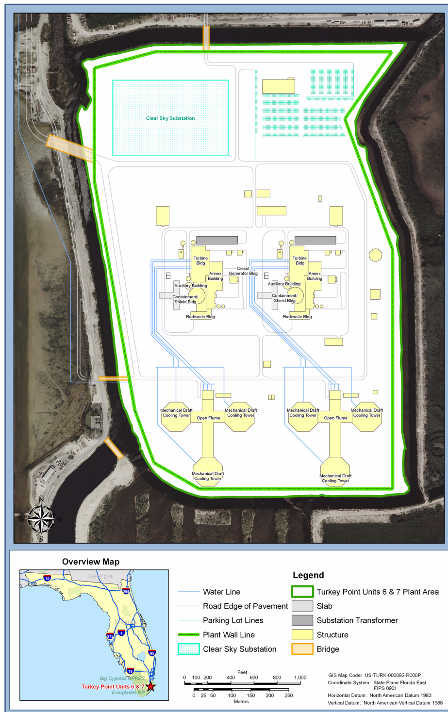
Figure 2.1-205 Principal Plant Structures within the Site Area
