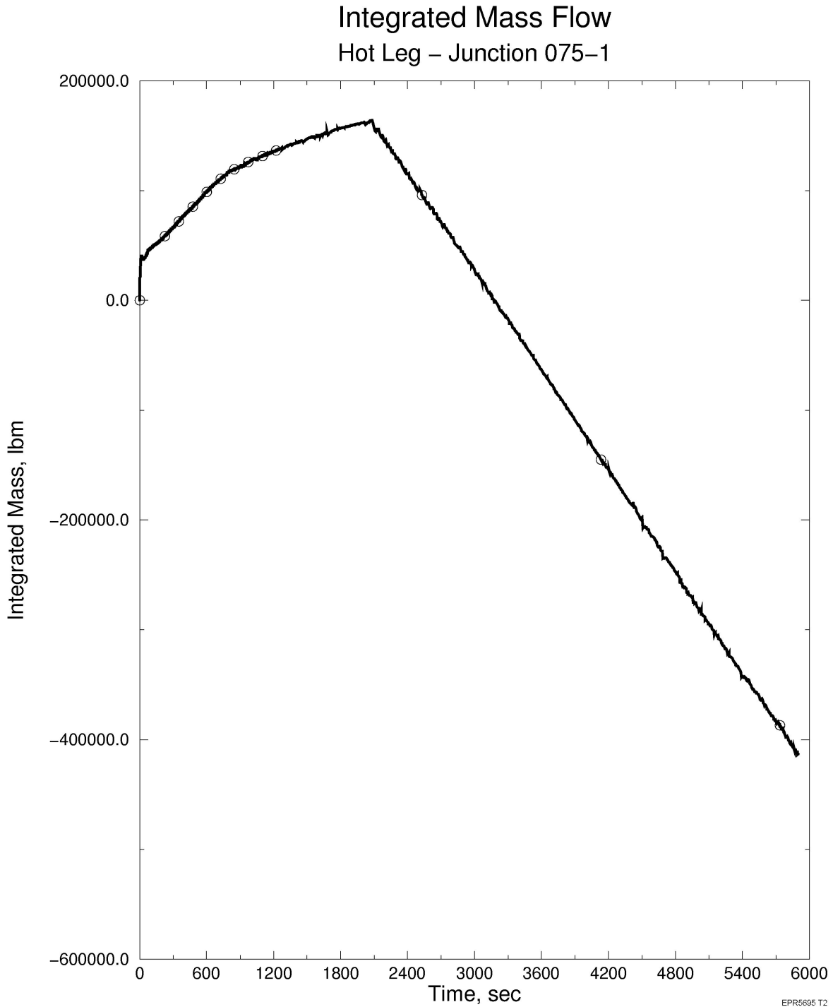
Figure 15.6-88—Upper Plenum Flow into the Hot Leg of a Loop Receiving Hot Leg Injection
