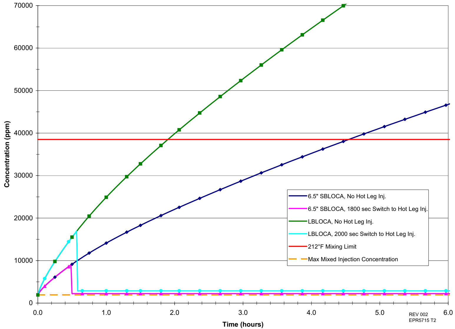
Figure 15.6-92—Time Dependent Boron Concentration During the Pool Boiling Period
