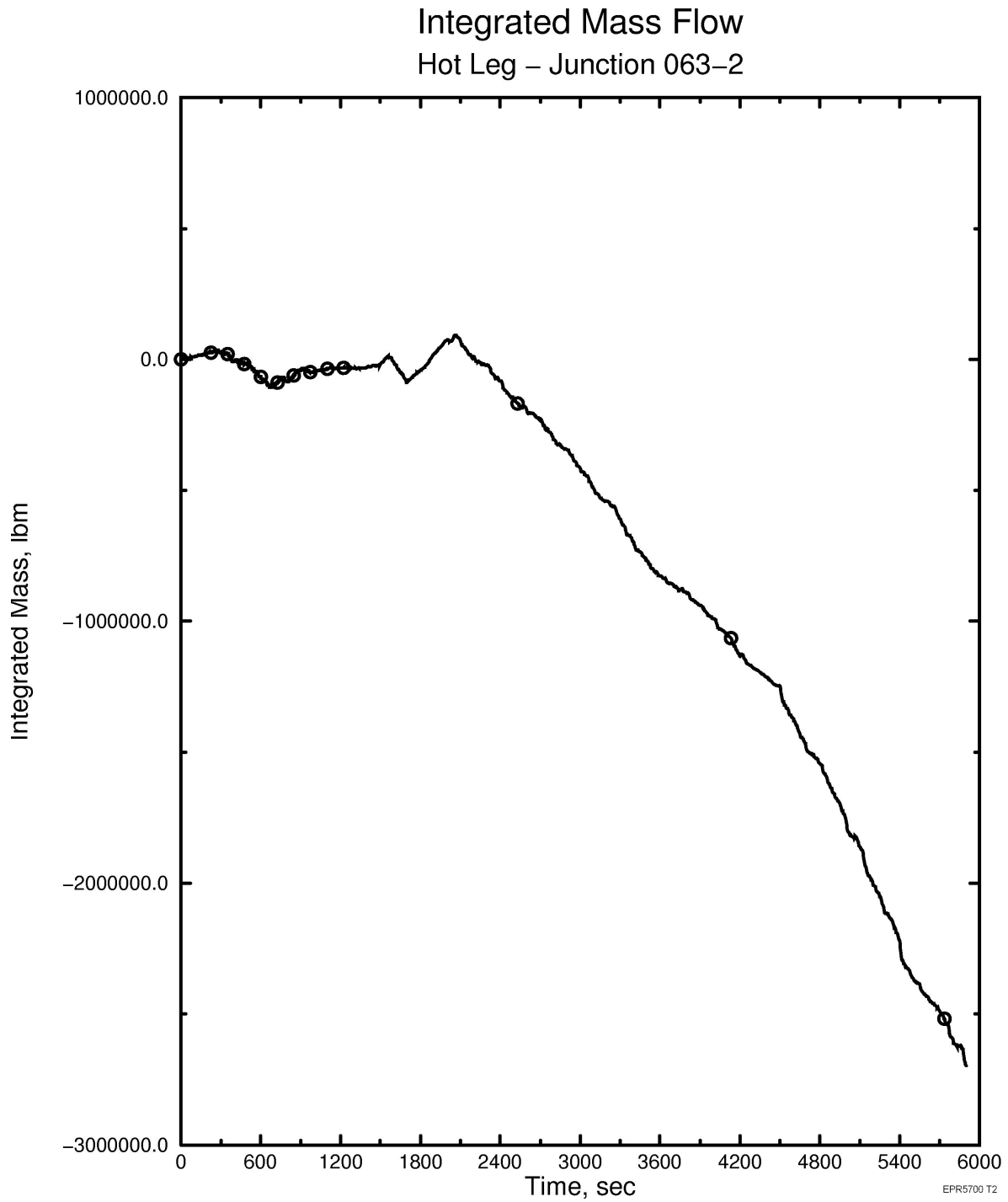
Figure 15.6-89—Peripheral Core Region Flow into Upper Plenum
