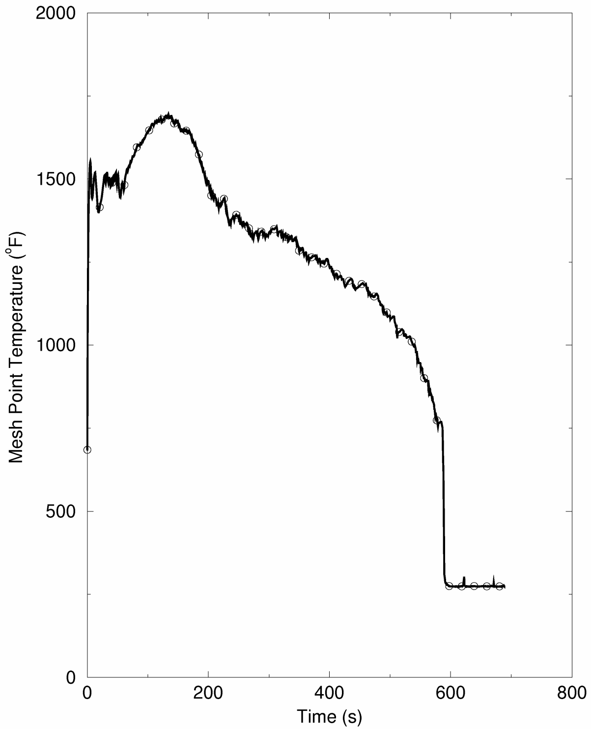
Figure 15.6-28—RLBLOCA - PCT Independent of Elevation for the Limiting PCT Case Hot Rod (Cycle 1)
