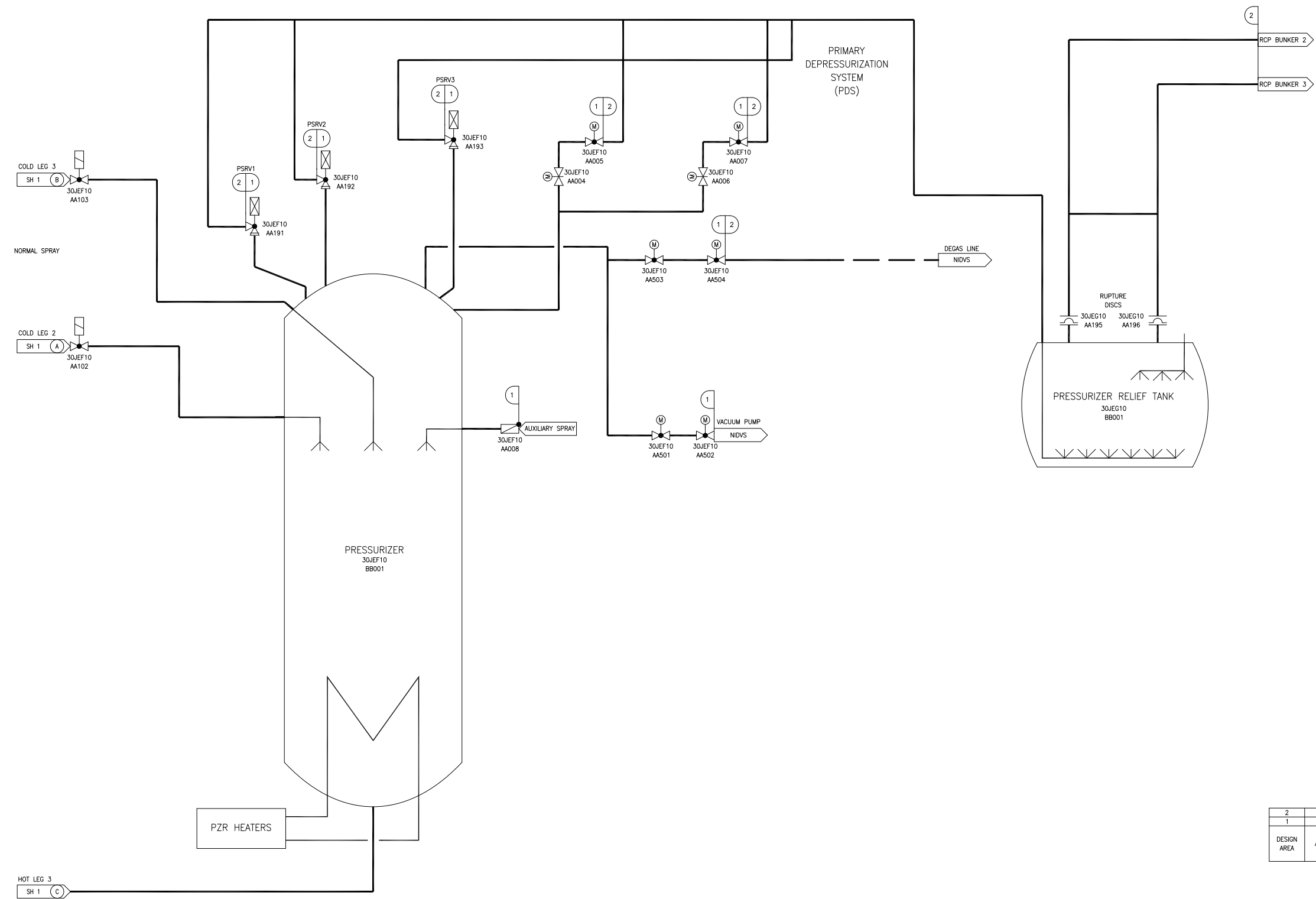
Figure 2.2.1-1—Reactor Coolant System Functional Arrangement Sheet 2 of 6
