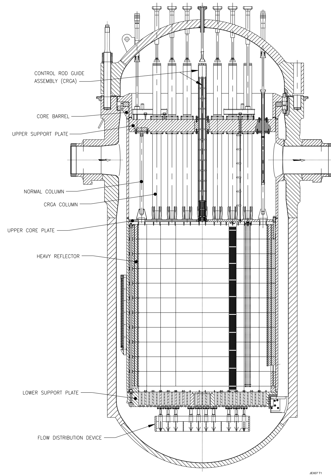
Figure 2.2.1-2—Reactor Pressure Vessel Functional Arrangement Sheet 1 of 2
