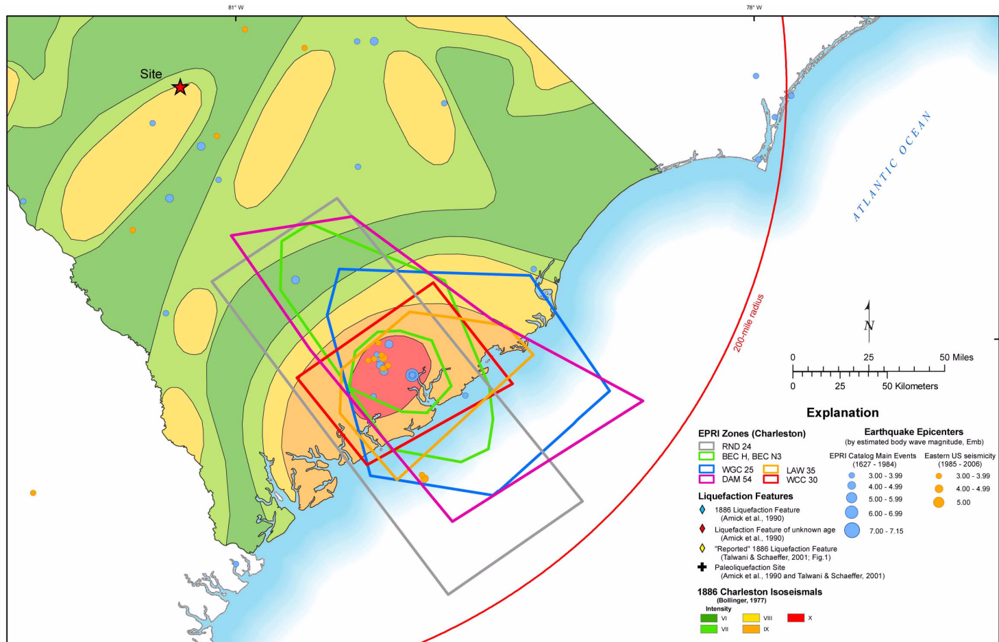
Figure 2.5.2-212. EPRI Representations of Charleston Seismic Source
