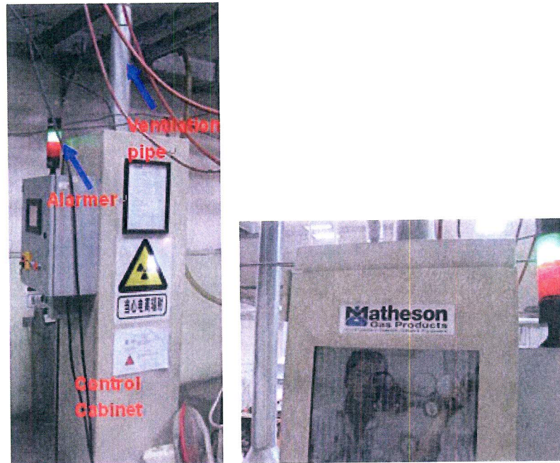
Fig. 3 Kr-85 gas operation system
