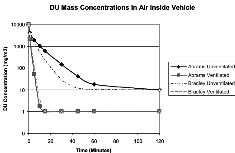
FIGURE 8-1 Committee-predicted mass concentrations of DU in air in vehicles after impact.
