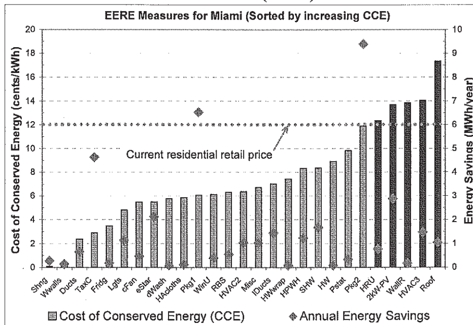
Figure A-1. Annual Energy Savings and Levelized Cost of Conserved Energy for Energy Efficiency and Renewable Energy Measures and Packages for New Homes in South Florida (Miami)
