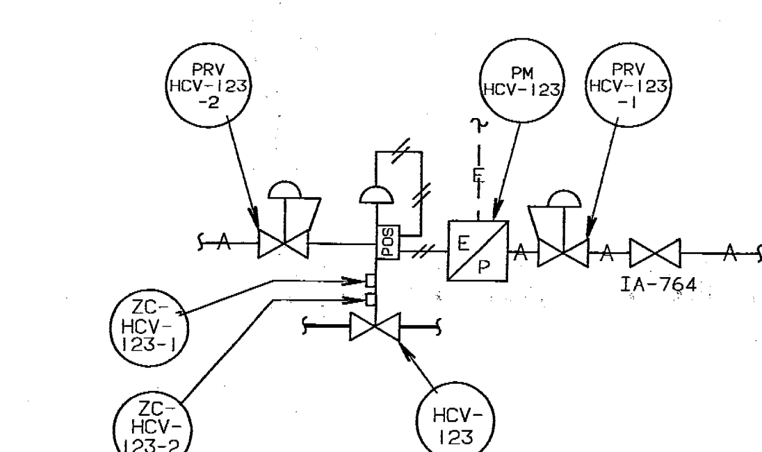
DETAIL "Y"
