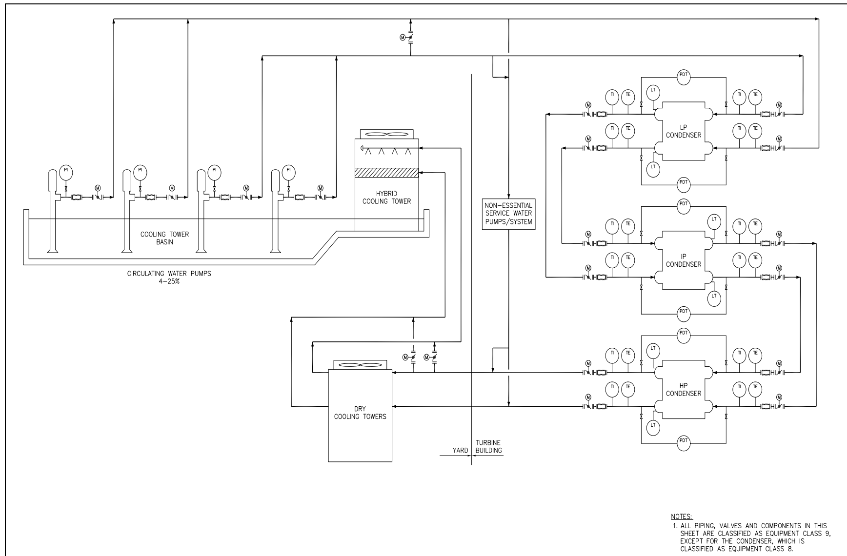
NAPS COL 10.4(1) Figure 10.4.5-1R Circulating Water System NAPS DEP 10.4(1)
