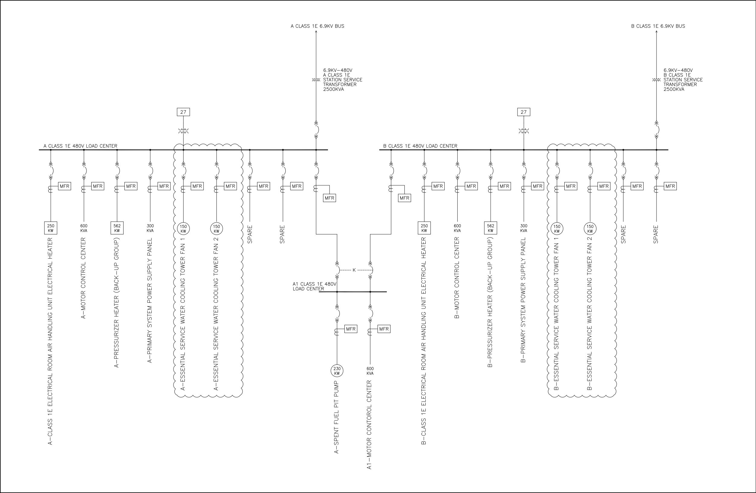
Figure 8.3.1-1R Onsite AC Electrical Distribution System (Sheet 5 of 7) — Class 1E 480V Buses A and B One Line Diagram
