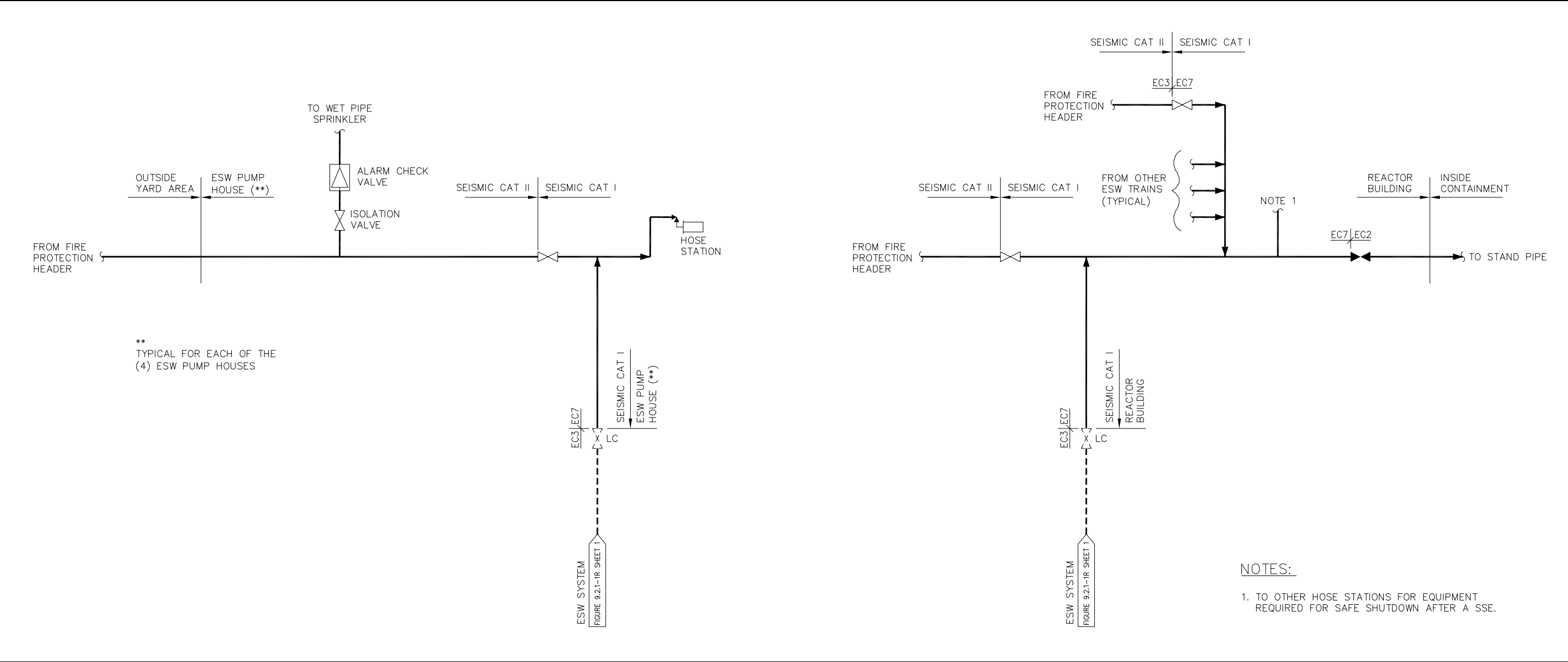
Figure 9.5.1-203 ESW to Fire Protection Cross-Tie Flow Schematic
