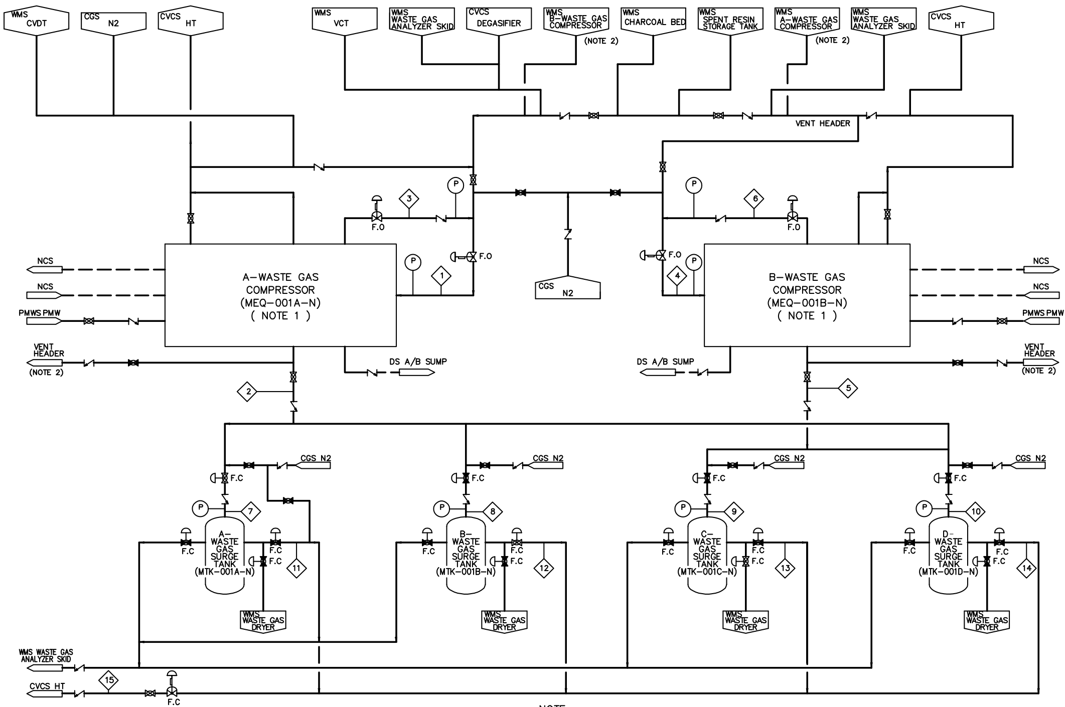
Figure 11.3-1R Gaseous Waste Management System Process Flow Diagram (Sheet 1 of 3)
