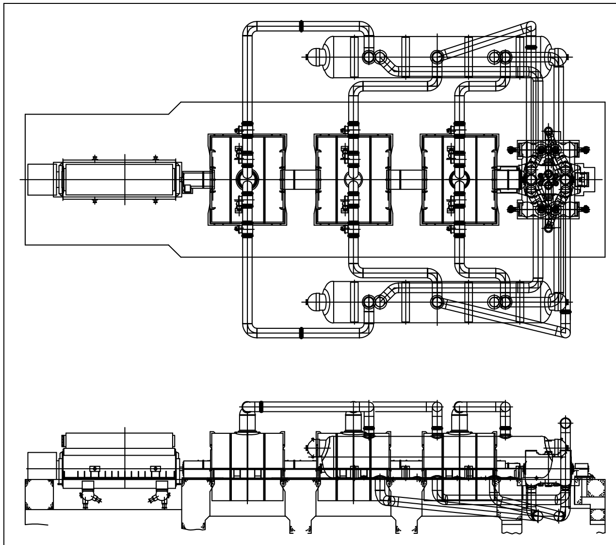
NAPS DEP 10.2(1) Figure 10.2-1R Turbine-Generator Outline Drawing
