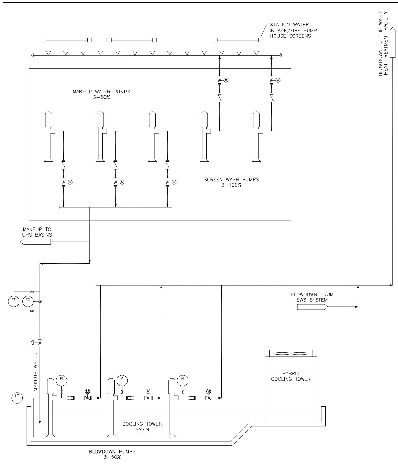
NAPS COL 10.4(1) Figure 10.4.5-201 Cooling Tower Make-Up and Blowdown System
