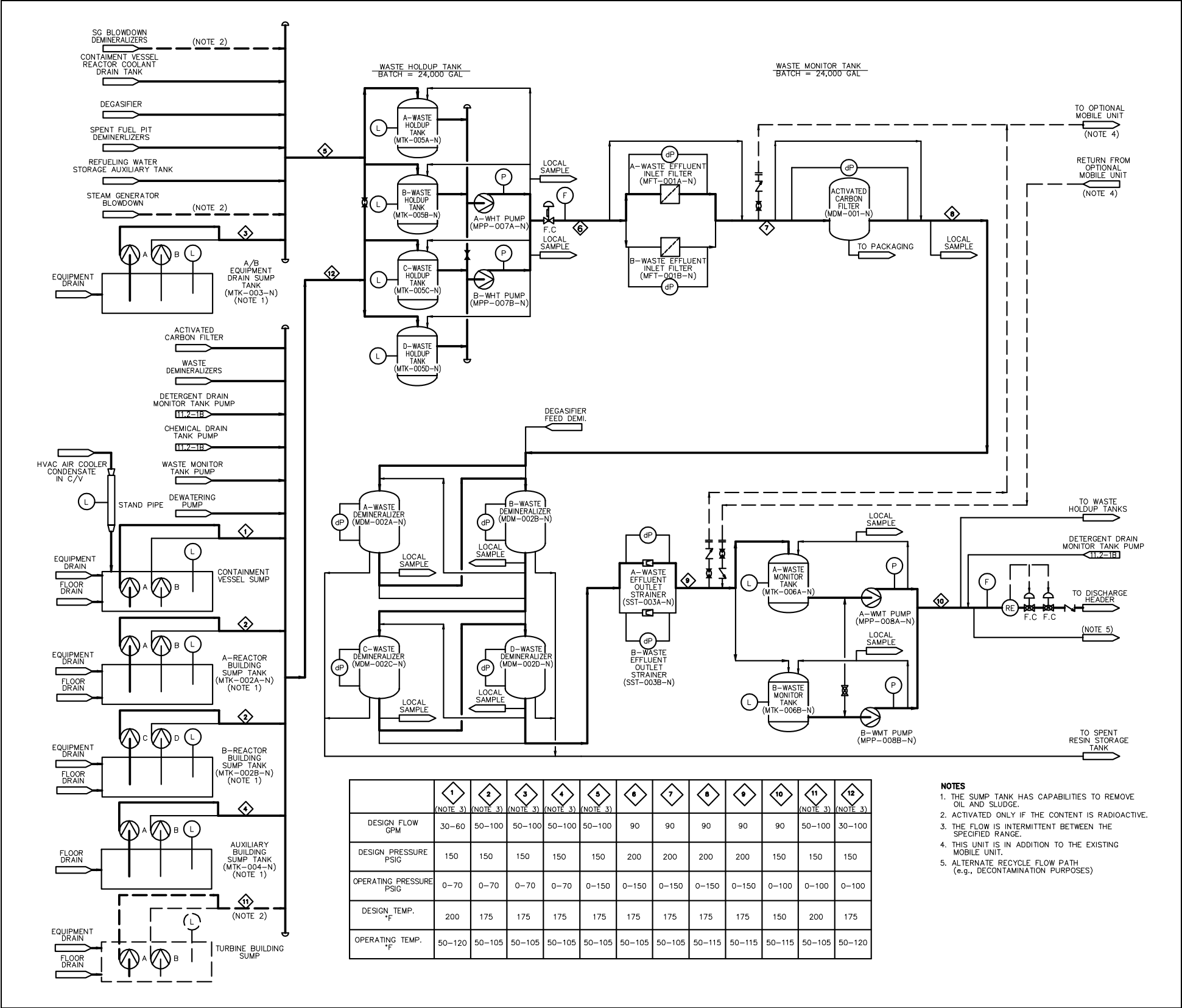
Figure 11.2-1R Liquid Waste Processing System Process Flow Diagram (Sheet 1 of 3)
