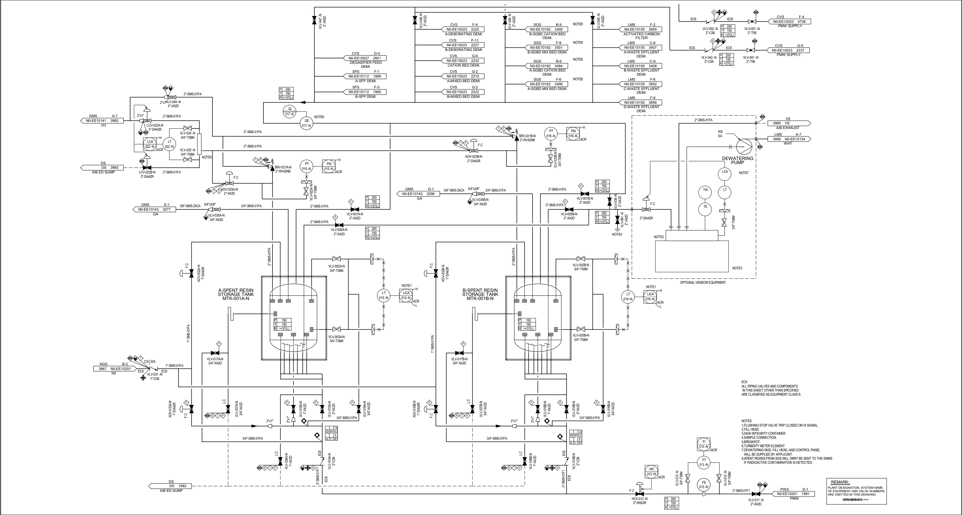
Figure 11.4-201 Solid Waste Management System Piping and Instrumentation Diagram
