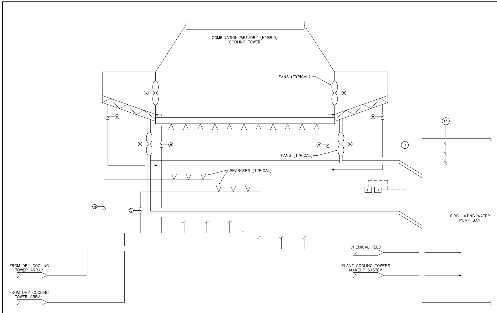
NAPS COL 10.4(1) Figure 10.4.5-203 Hybrid Cooling Tower
