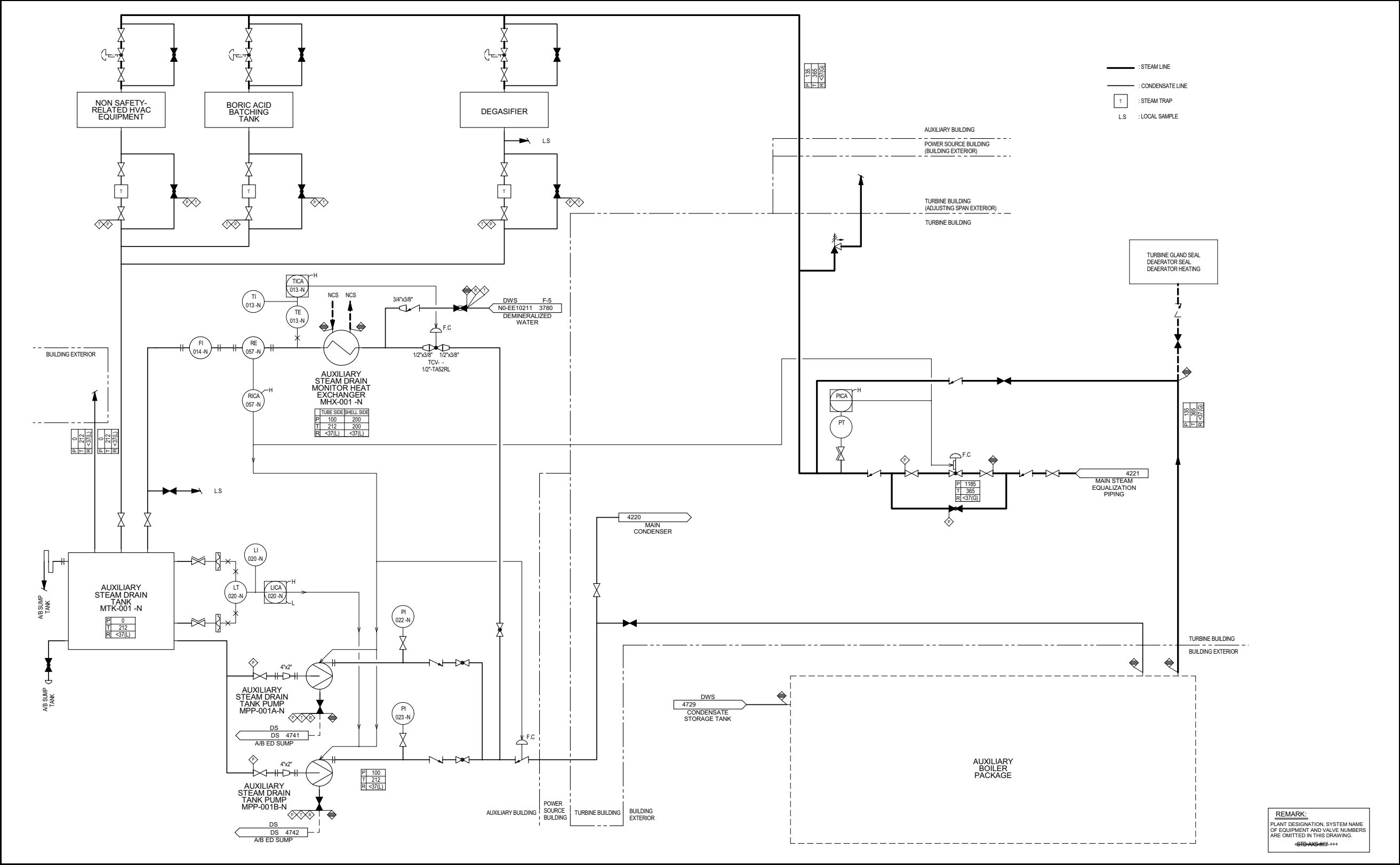
Figure 10.4-11R Auxiliary Steam Supply System Piping and Instrumentation Diagram
