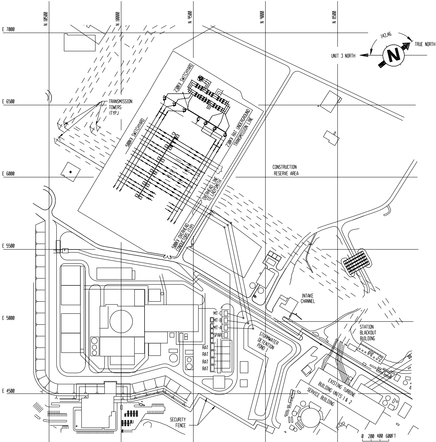
Figure 8.2-202 500/230 kV Switchyard Arrangement
