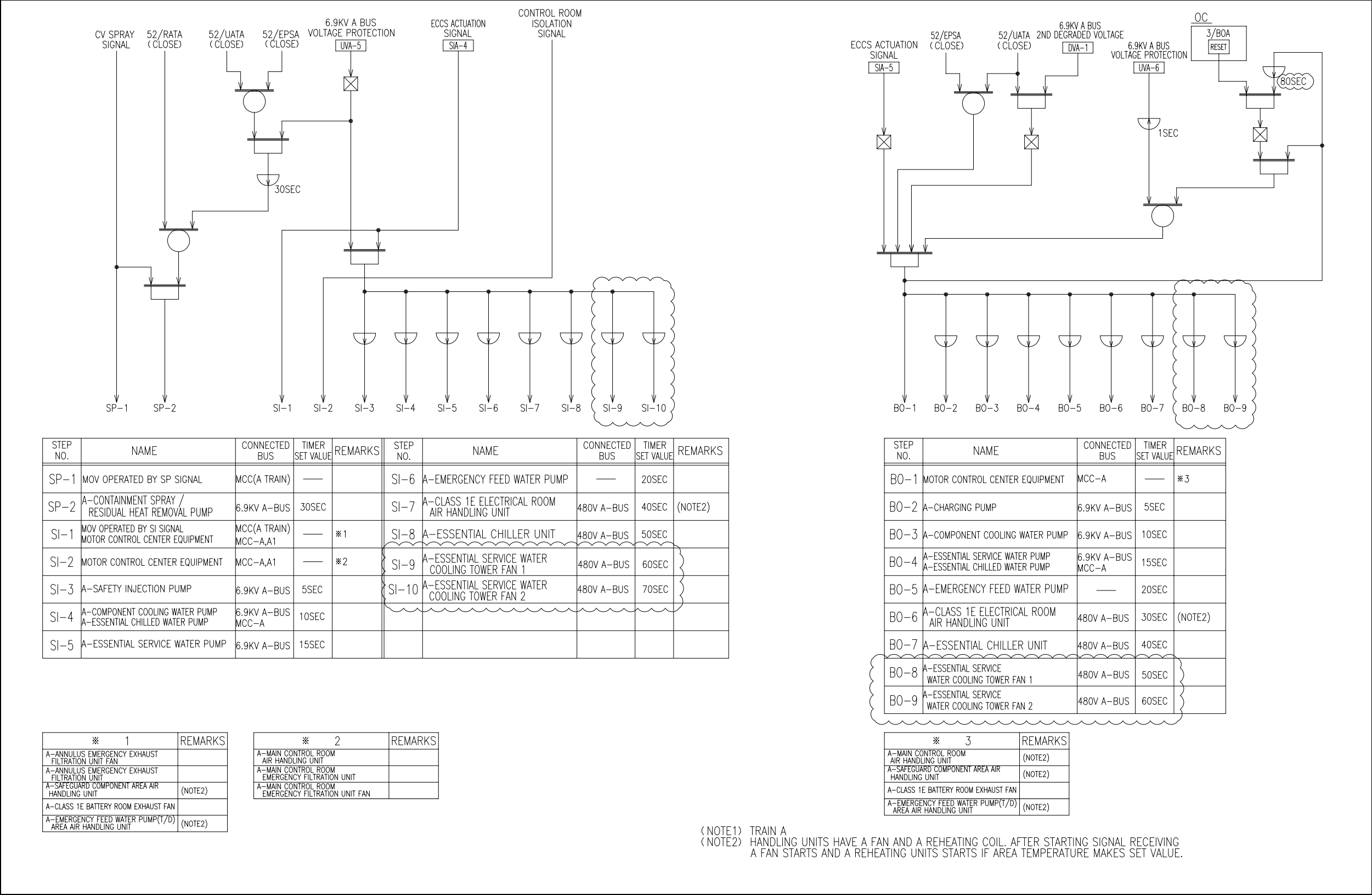
Figure 8.3.1-2R Logic Diagrams (Sheet 18 of 24) — Class 1E Train A LOOP and LOCA Load Sequencing
