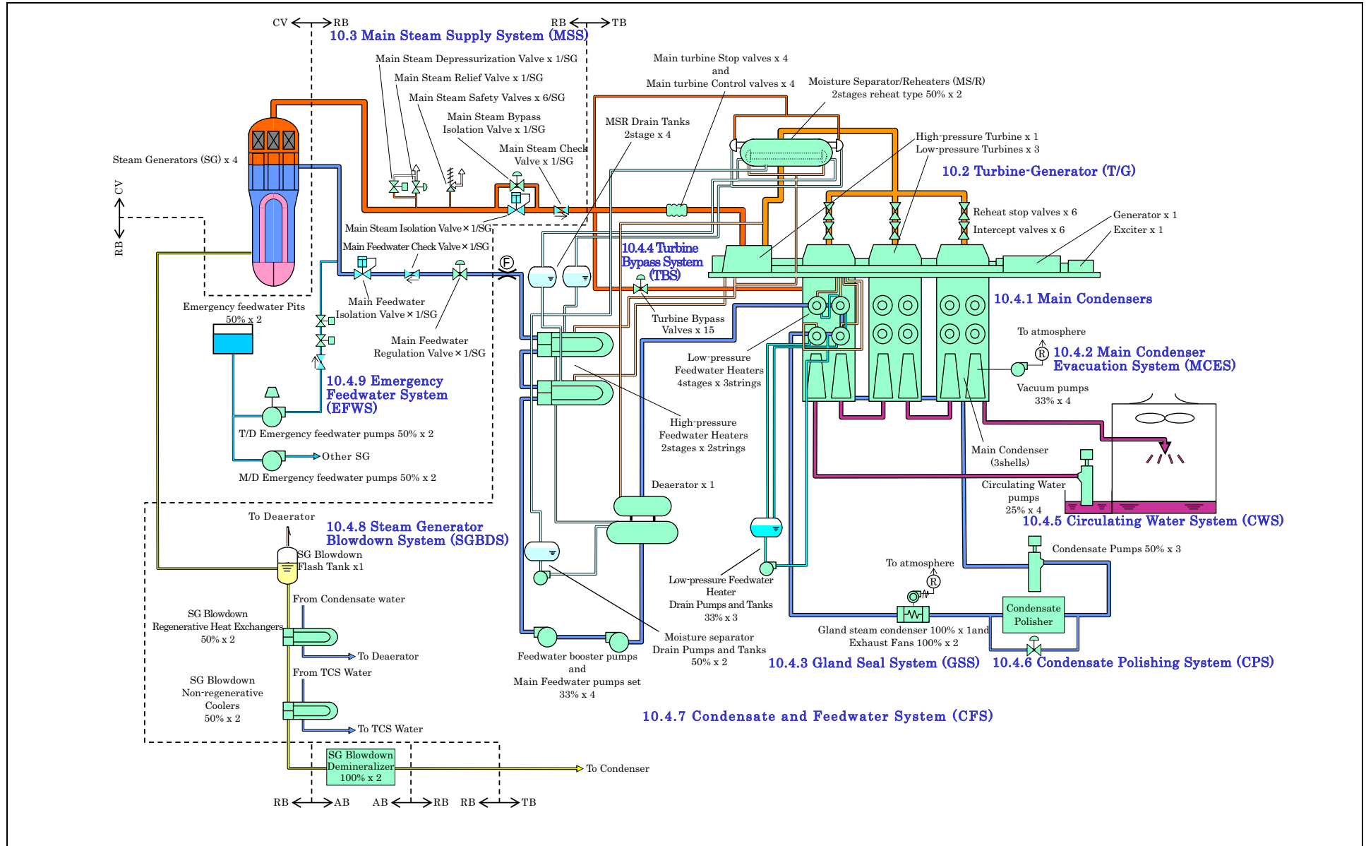
Figure 10.1-1R Overall System Flow Diagram
