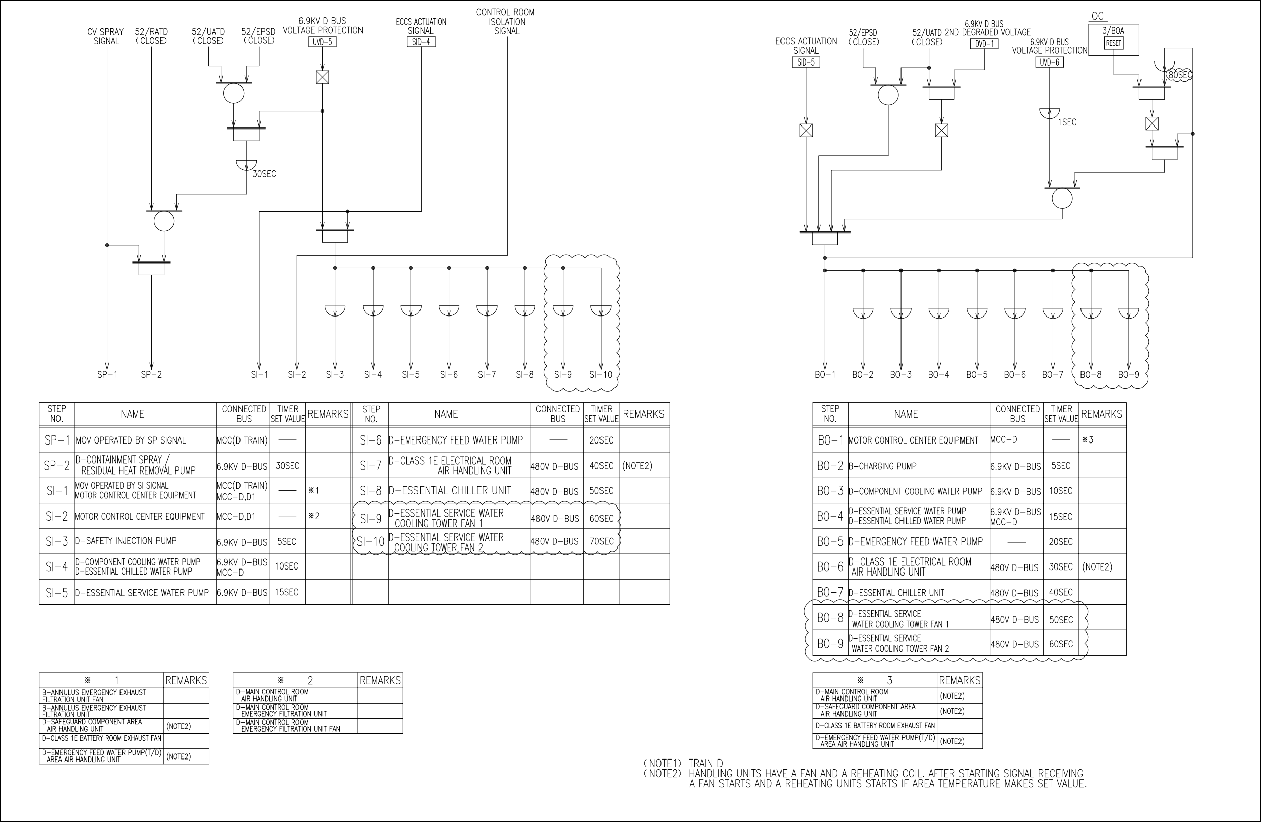
STD* COL 9.2(20) Figure 8.3.1-2R Logic Diagrams (Sheet 21 of 24) — Class 1E Train D LOOP and LOCA Load Sequencing
