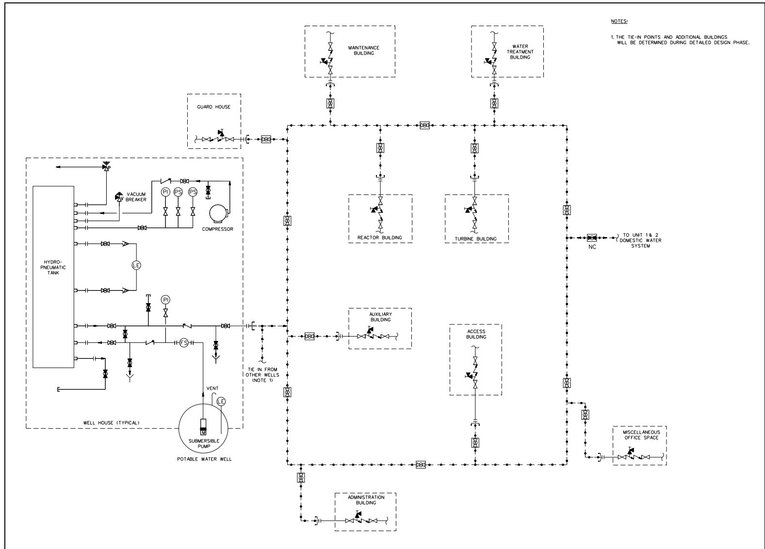
Figure 9.2.4-1R Potable and Sanitary Water System Flow Diagram (Sheet 1 of 2)
