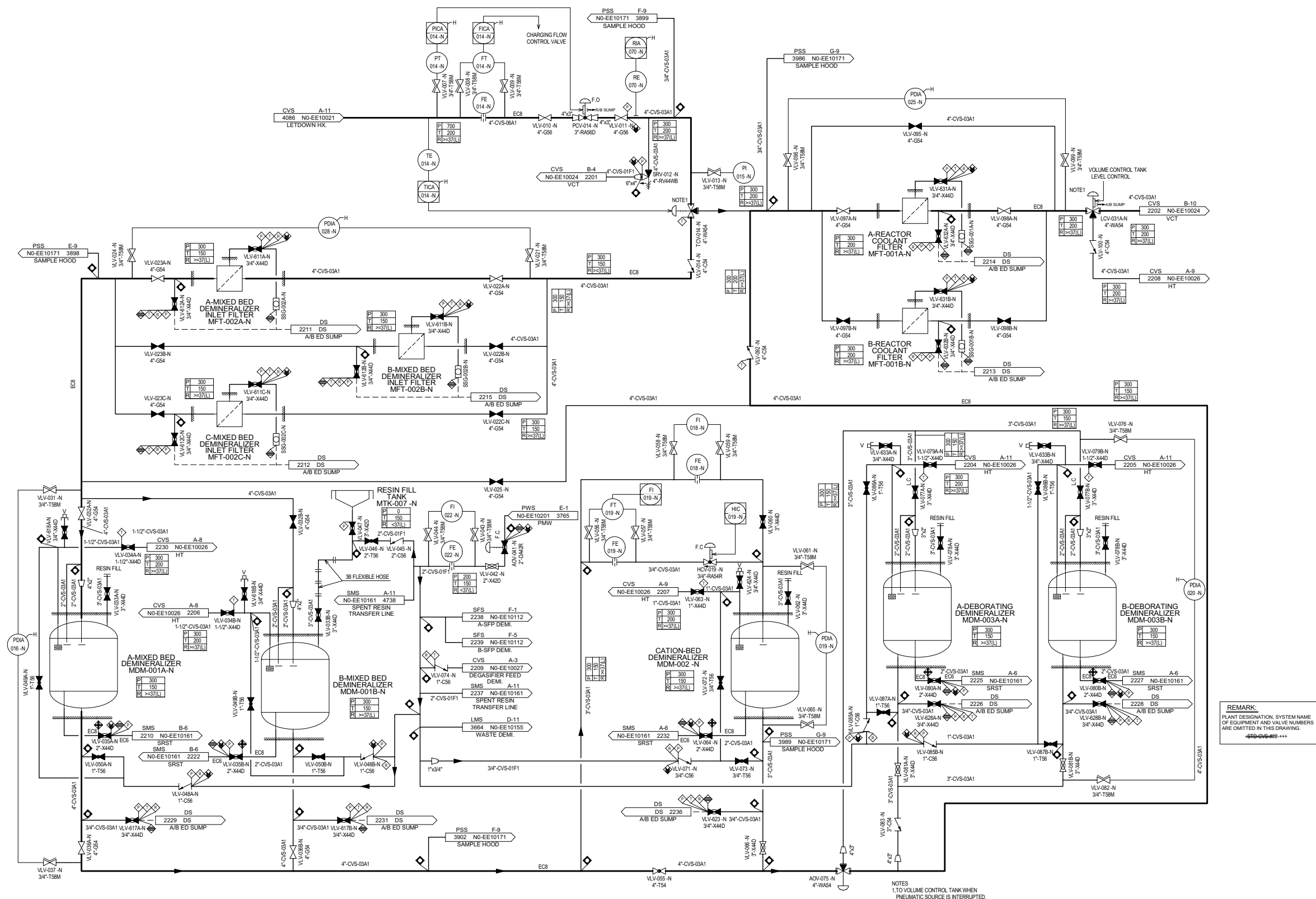
Figure 9.3.4-1R Chemical and Volume Control System Flow Diagram (Sheet 3 of 7)
