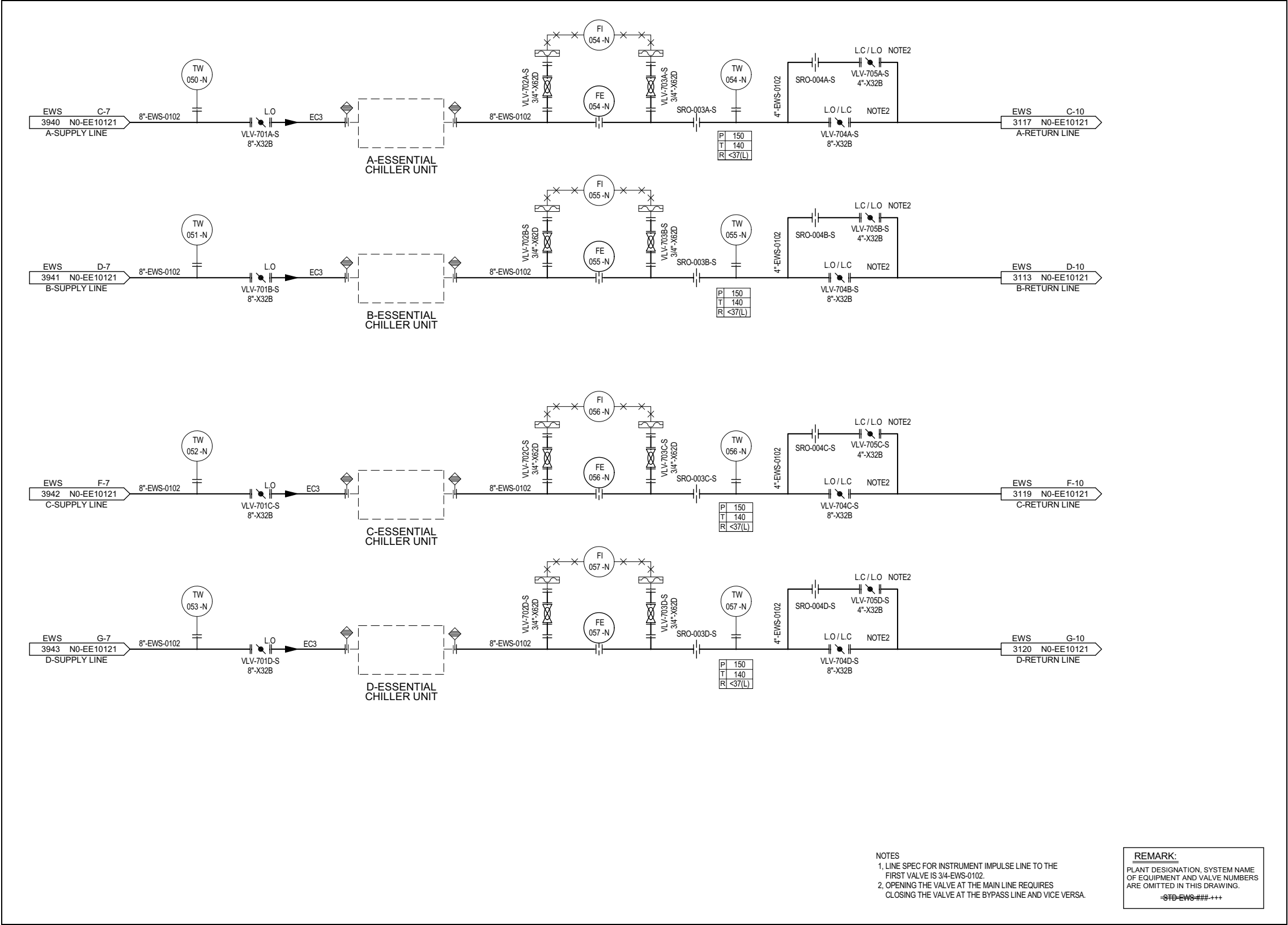
Figure 9.2.1-1R Essential Service Water System Piping and Instrumentation Diagram (Sheet 2 of 2)
