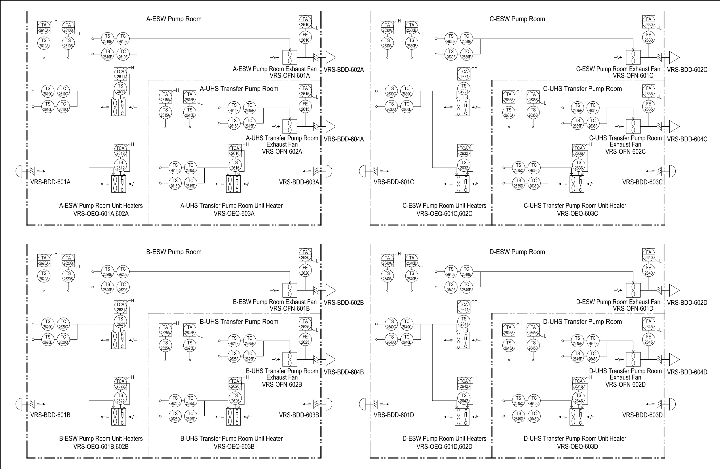
Figure 9.4-201 UHS ESW Pump House Ventilation System Flow Diagram
