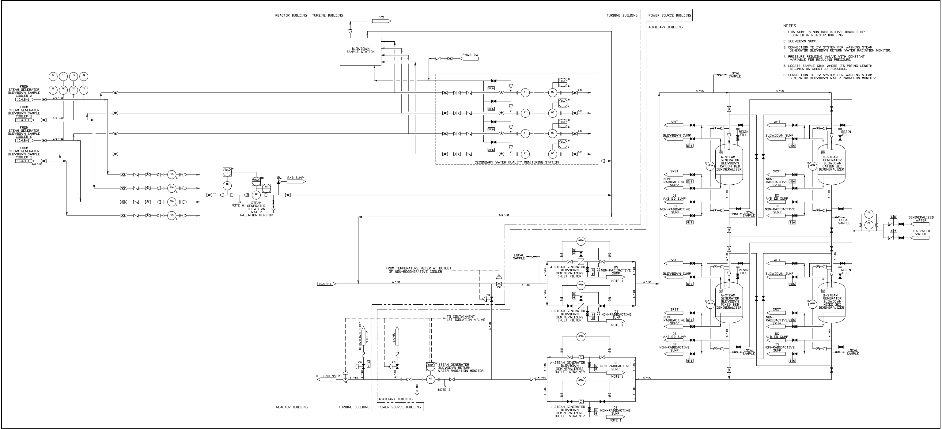
NAPS COL 10.4(2) Figure 10.4.8-2R Steam Generator Blowdown System FlowDiagram (Sheet 2 of 2)
