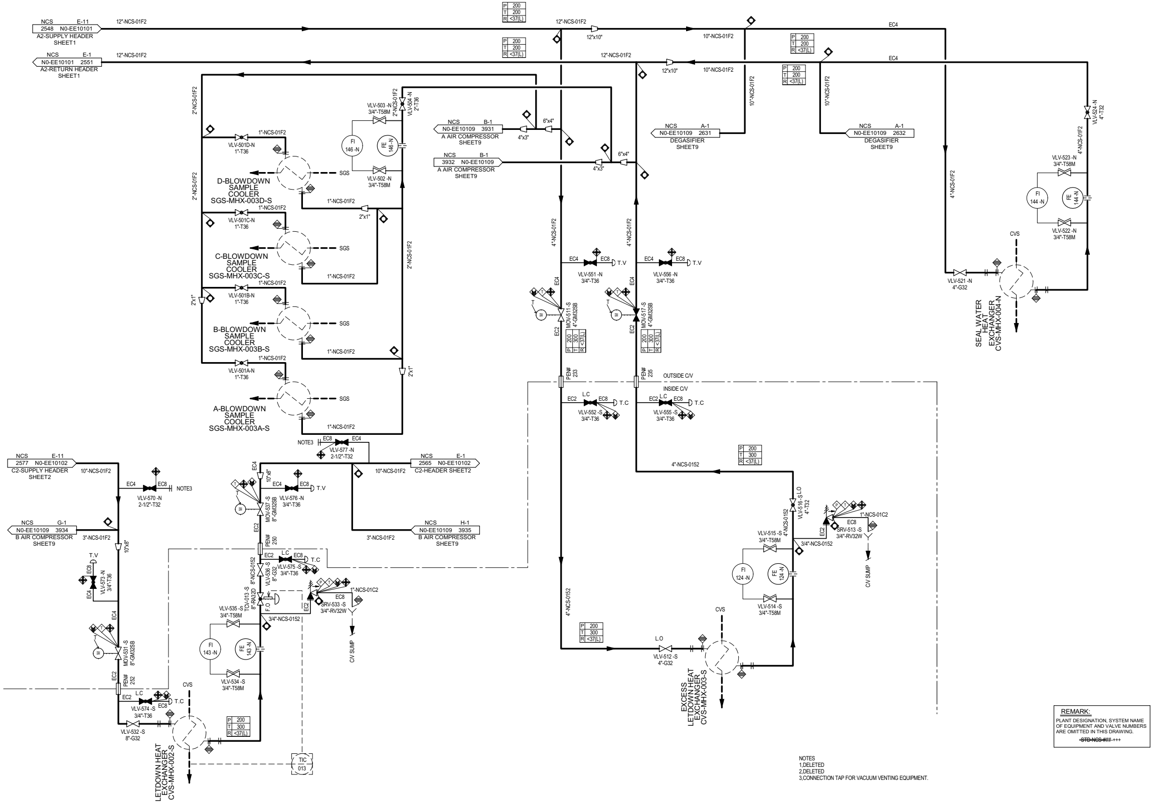
Figure 9.2.2-1R Component Cooling Water System Piping and Instrumentation Diagram (Sheet 8 of 9)
