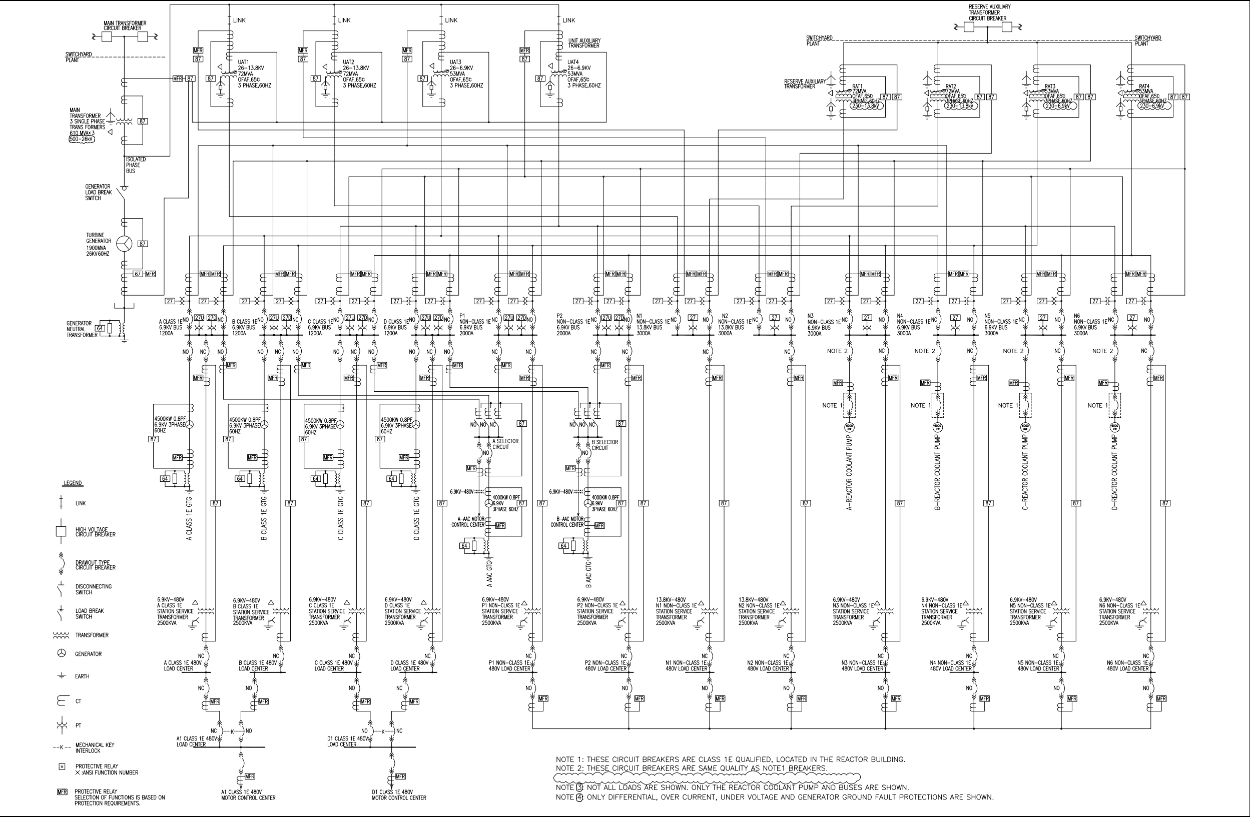
Figure 8.3.1-1R Onsite AC Electrical Distribution System (Sheet 1 of 7) — Main One Line Diagram
