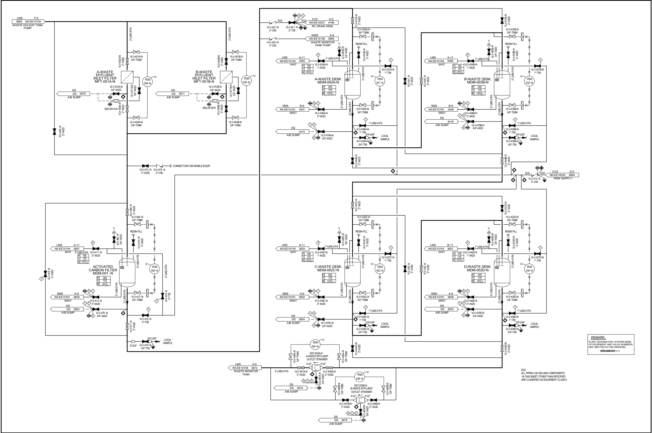
Figure 11.2-201 Liquid Waste Management System Piping and Instrumentation Diagram (Sheet 5 of 8)
