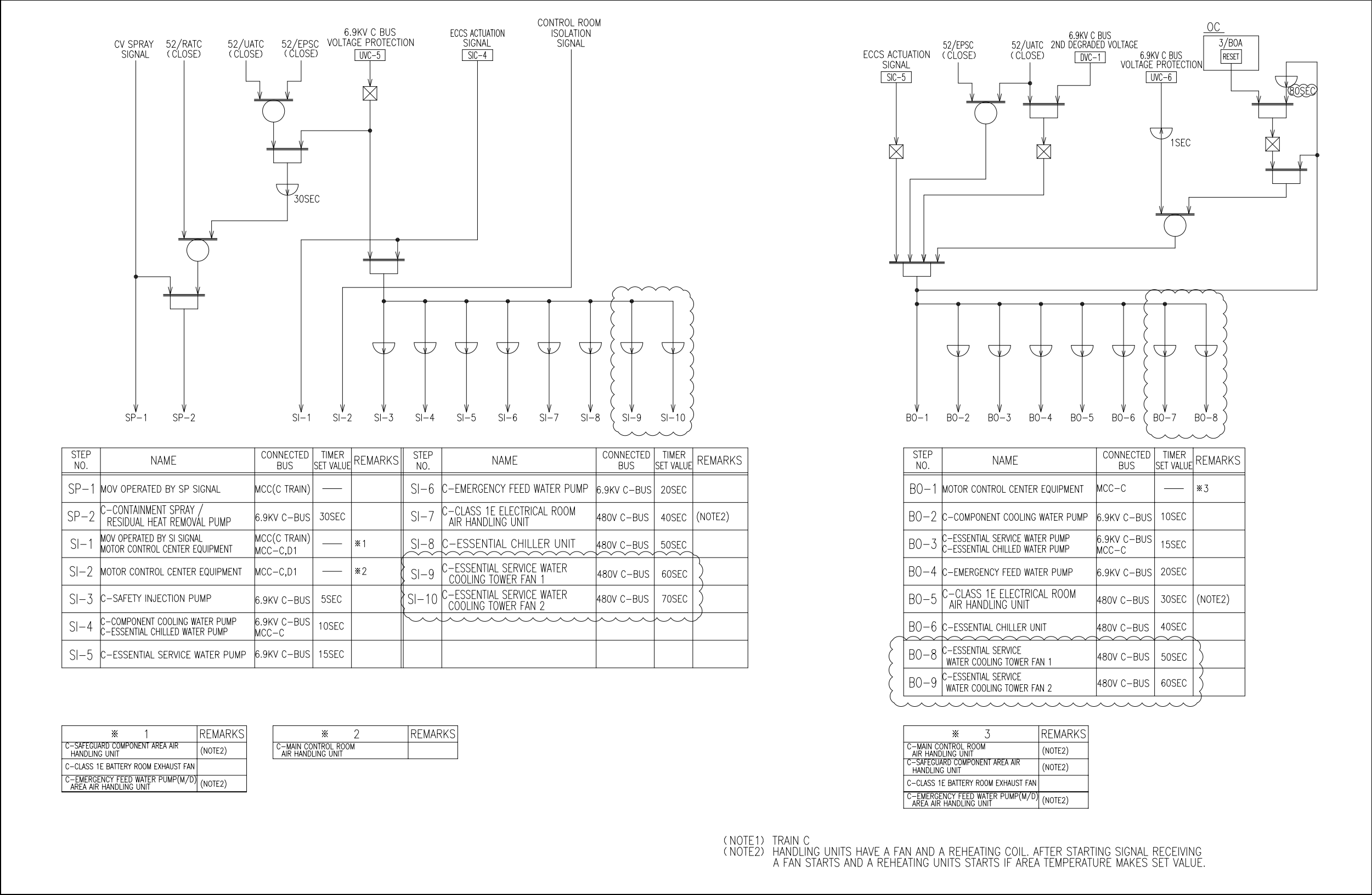
STD* COL 9.2(20) Figure 8.3.1-2R Logic Diagrams (Sheet 20 of 24) — Class 1E Train C LOOP and LOCA Load Sequencing
