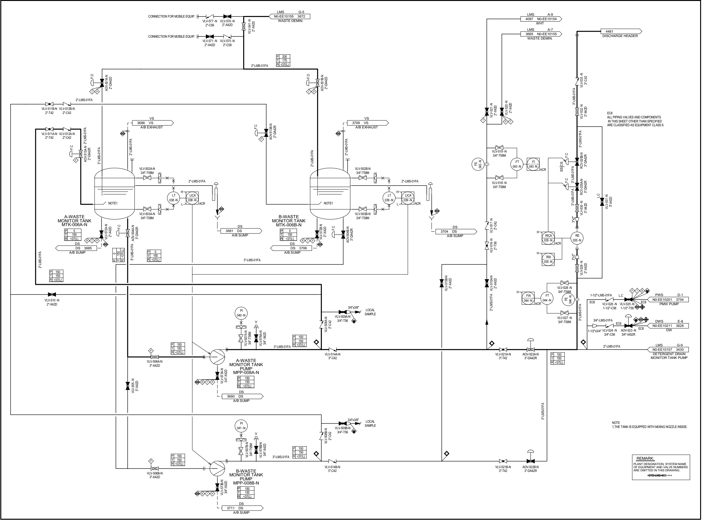
Figure 11.2-201 Liquid Waste Management System Piping and Instrumentation Diagram (Sheet 6 of 8)
