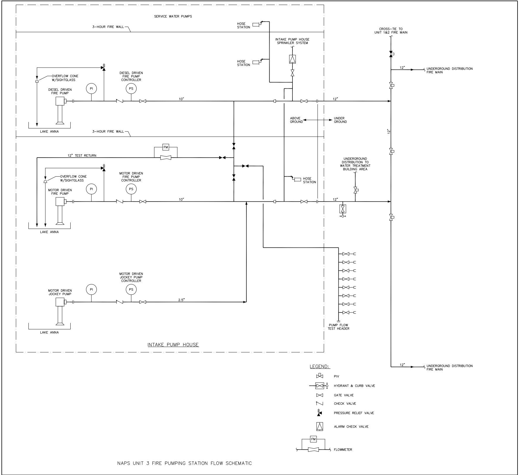
Figure 9.5.1-202 Fire Pumping Station Flow Schematic
