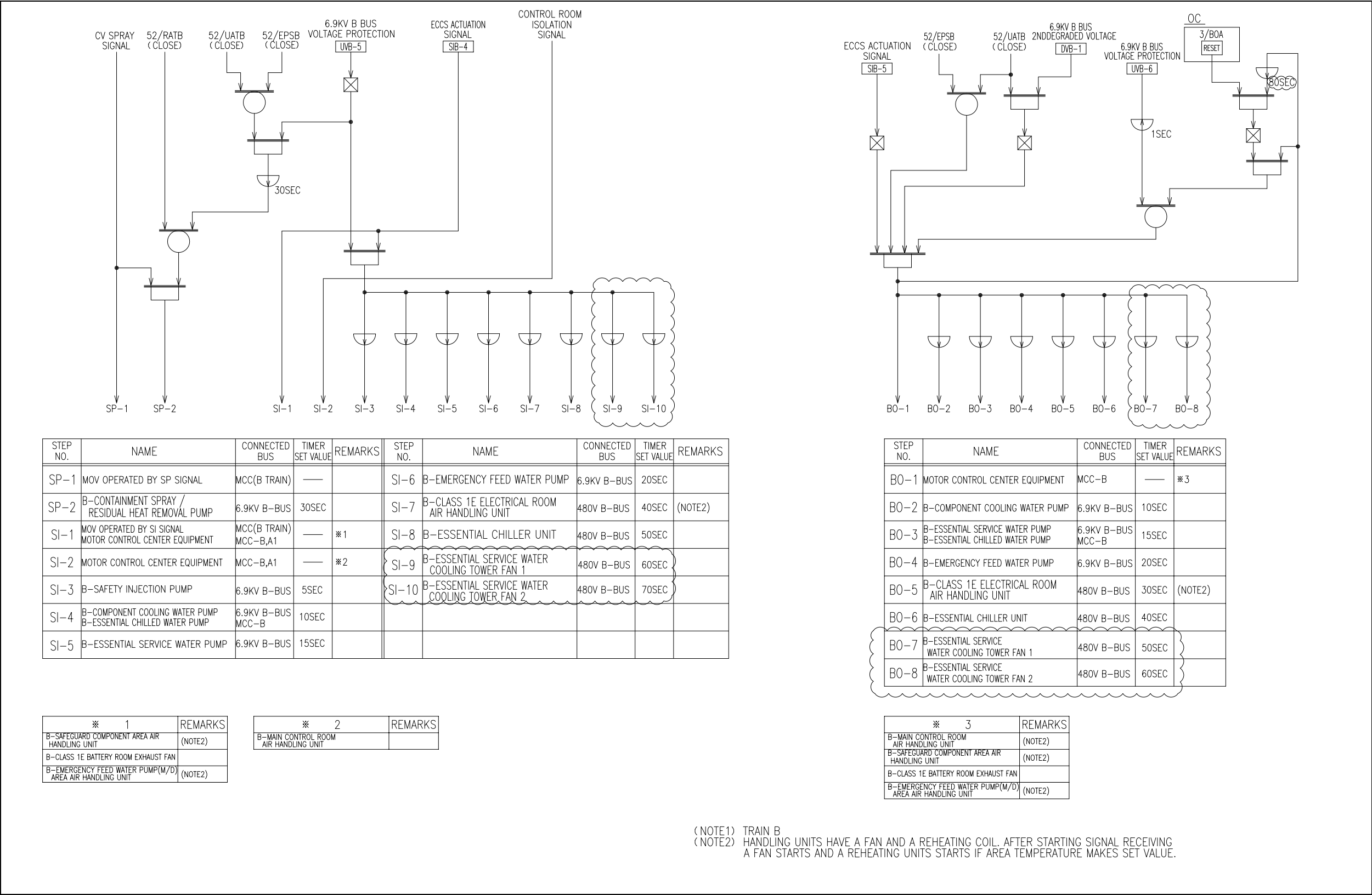
Figure 8.3.1-2R Logic Diagrams (Sheet 19 of 24) — Class 1E Train B LOOP and LOCA Load Sequencing
