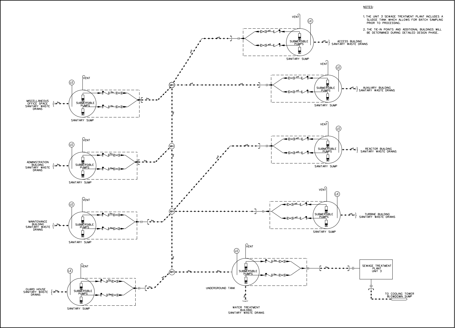
Figure 9.2.4-1R Potable and Sanitary Water System Flow Diagram (Sheet 2 of 2)
