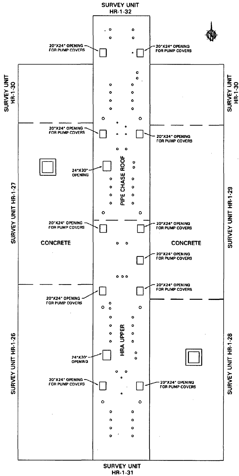
Exhibit 5, HRA Vault and Pipe Chase Roofs Showing Survey Units
