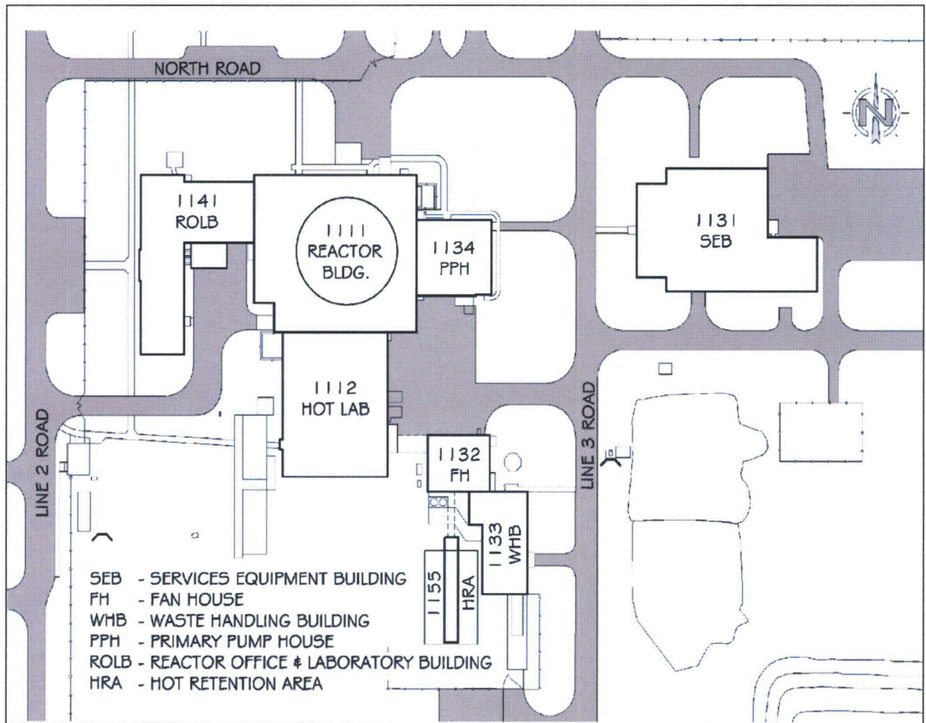
Figure 1, PBRF NW Area Showing Reactor Building, HRA and Other Support Buildings
