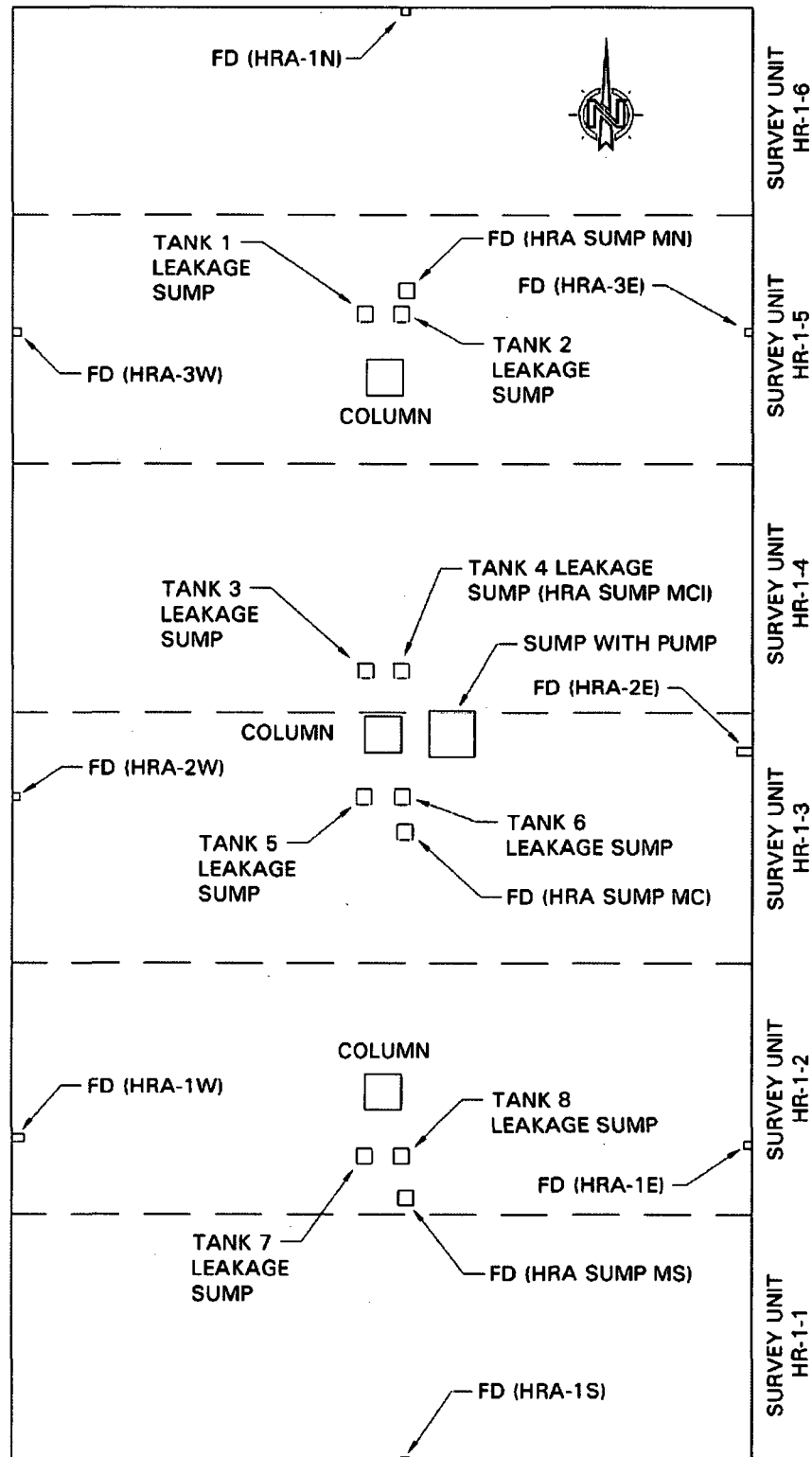
Exhibit 2, HRA Vault Floor Layout Showing Survey Units
