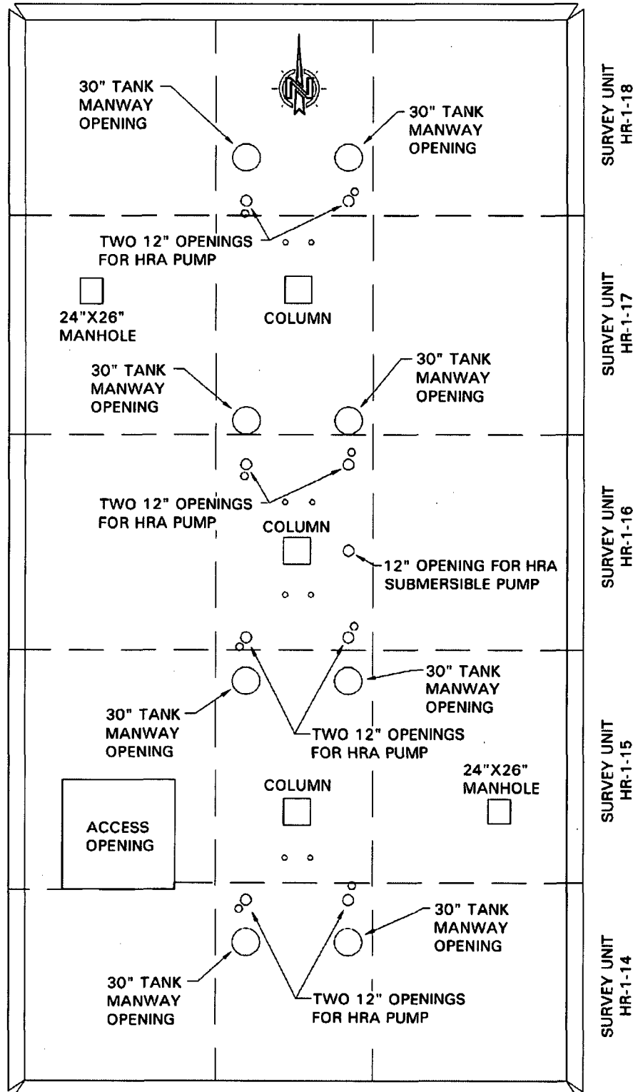
Exhibit 3, HRA Vault Ceiling Showing Survey Units
