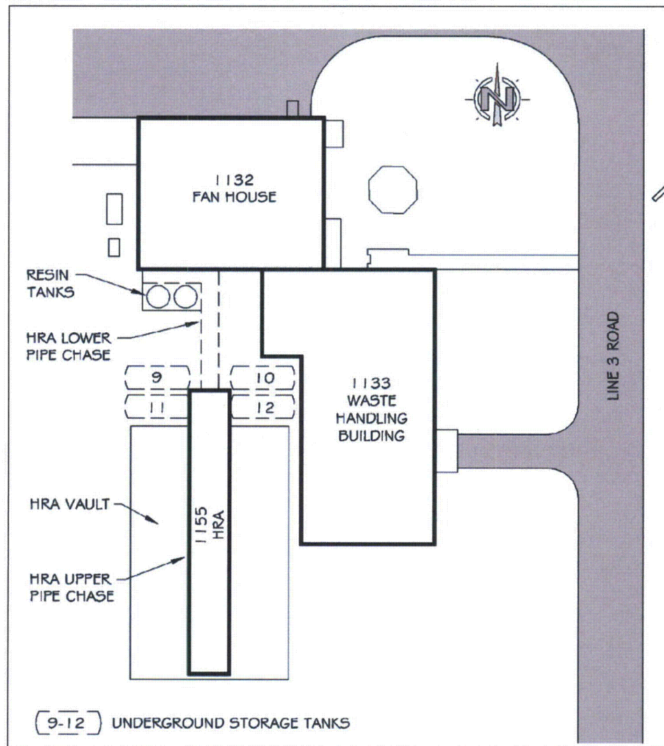
Figure 2, Expanded View Showing HRA Pipe Chase and Underground Tank Arrangement
