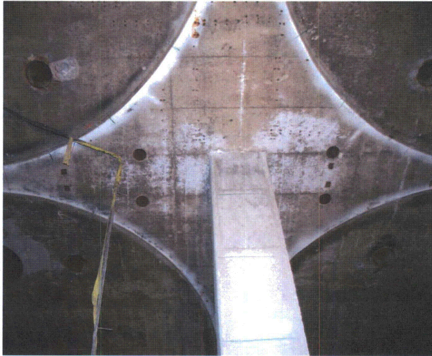
View of Ceiling in Central Vault Area Showing Support Column (Survey Unit HR-1-16)
