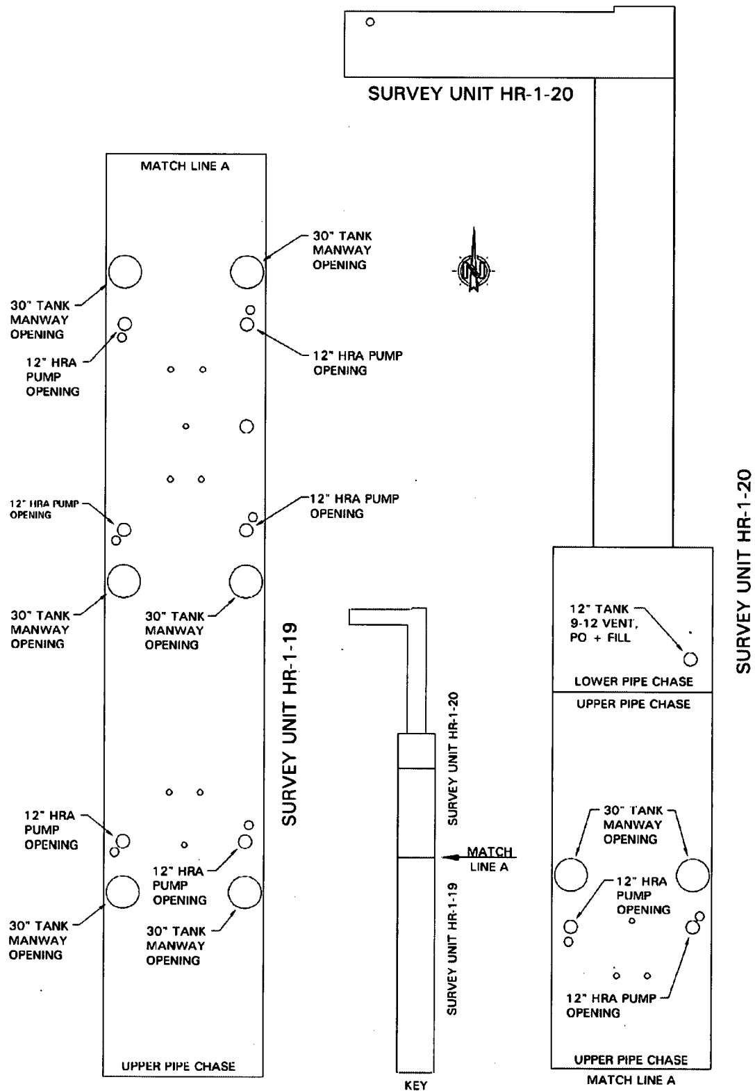
Exhibit 4. HRA Pipe Chase Floor Layout Showing Survey Units
