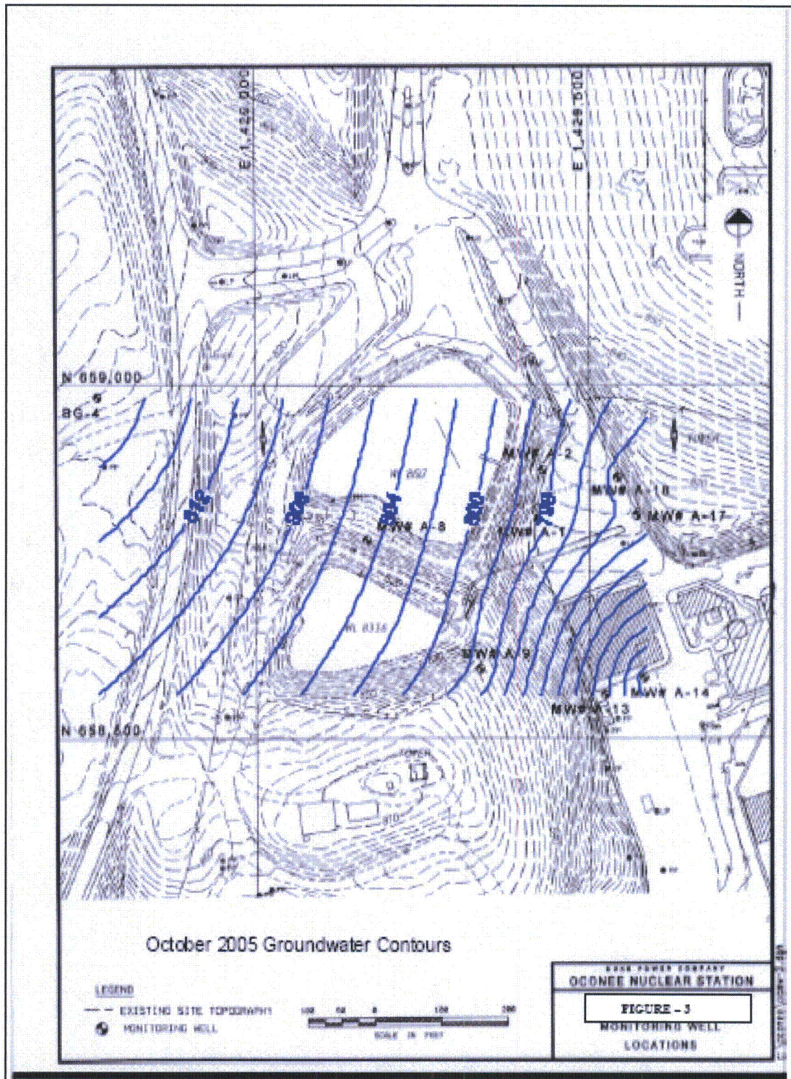
Figure 3: Groundwater Contours: CTP1 and CTP2 (October 2005)
